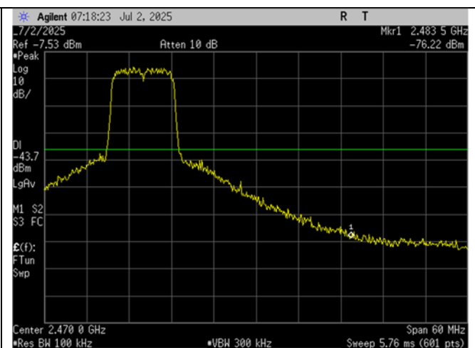
High Ch_2454MHz_10MHz BW_-20dBc_Upper Band Edge_Port 2
