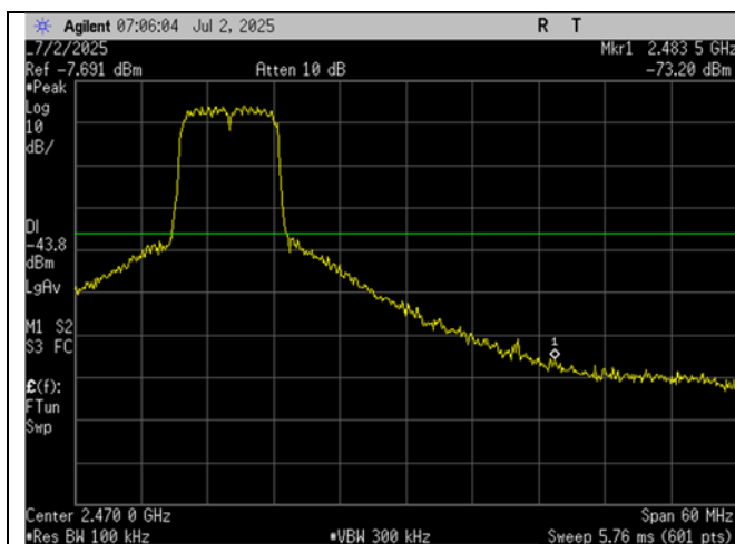
High Ch_2454MHz_10MHz BW_-20dBc_Upper Band Edge_Port 1
