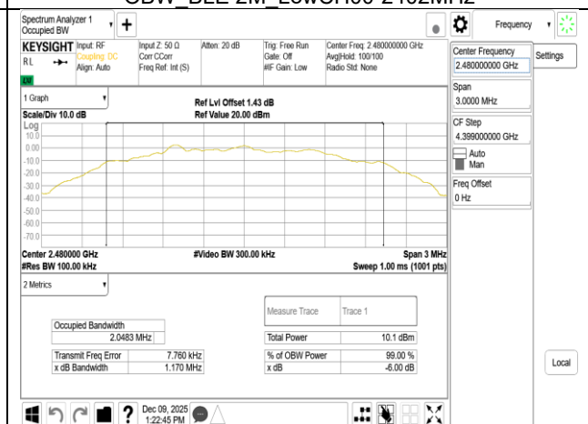
OBW_BLE 2M_HighCH39-2480MHz
