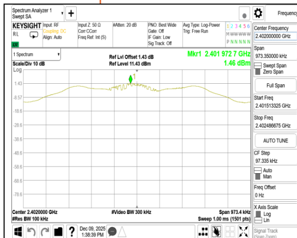
Reference Level_BLE 125k_LowCH00-2402MHz
