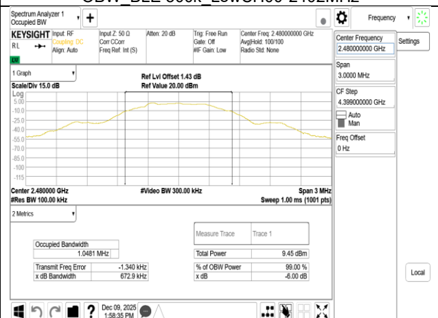
OBW_BLE 500k_HighCH39-2480MHz
