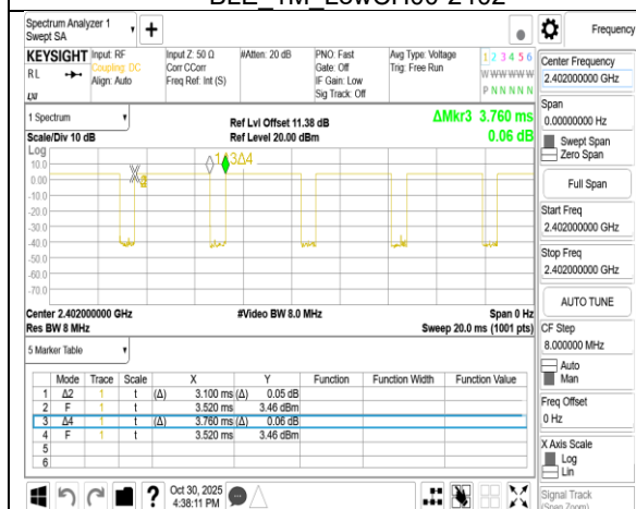
BLE_125k_LowCH00-2402
