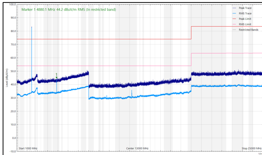
Figure 22 - CH17_LE1M_Y Plane, 2440 MHz, 1 GHz to 25 GHz, Horizontal
