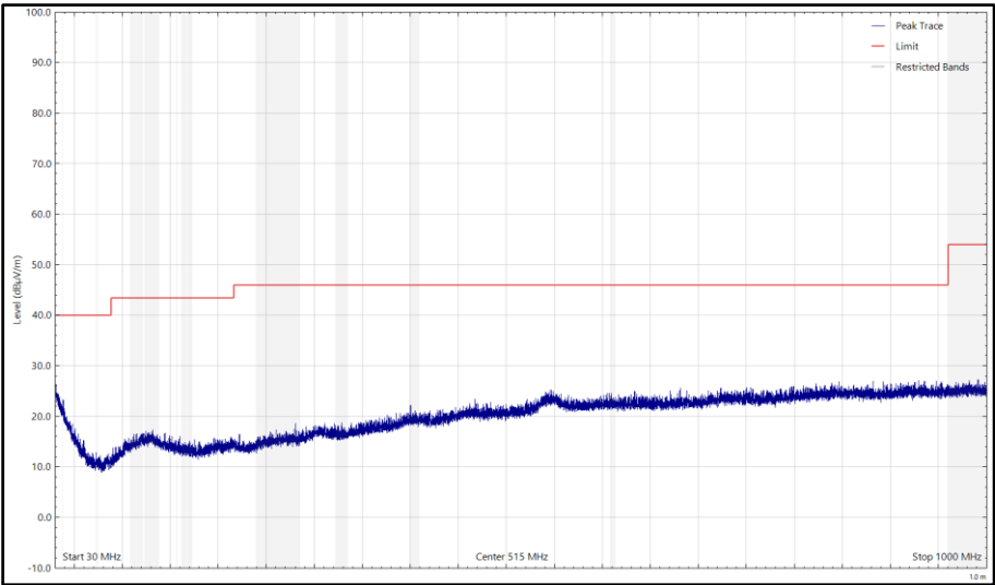
Figure 35 - CH39_LE1M_Y Plane, 2480 MHz, 30 MHz to 1 GHz, Vertical (Peak)
