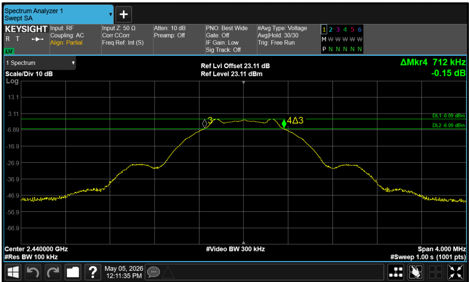
Figure 45 - SMA Pigtail (A) 2440 MHz (CH17) 6 dB Bandwidth
