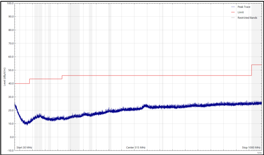
Figure 27 - CH17_LE1M_Z Plane, 2440 MHz, 30 MHz to 1 GHz, Vertical (Peak)
