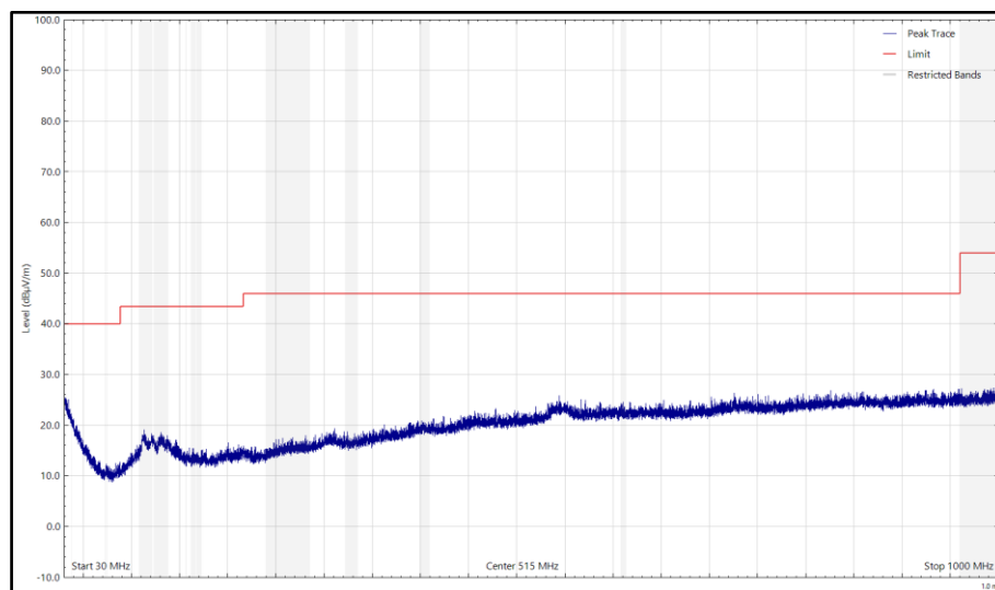
Figure 5 - CH37_LE1M_X Plane, 2402 MHz, 30 MHz to 1 GHz, Horizontal (Peak)
