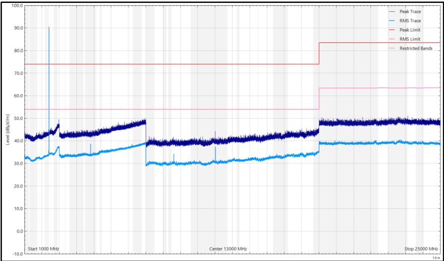
Figure 12 - CH37_LE1M_Y Plane, 2402 MHz, 1 GHz to 25 GHz, Vertical
