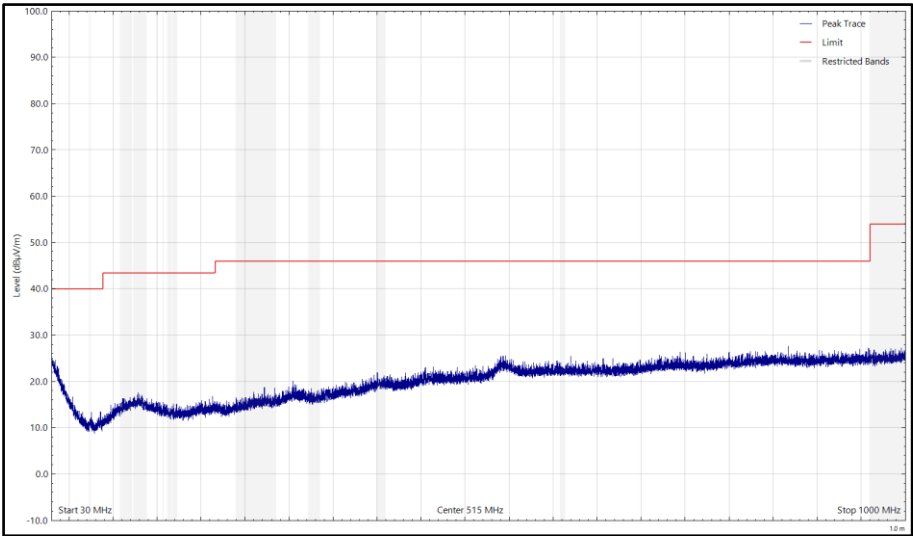
Figure 7 - CH37_LE1M_X Plane, 2402 MHz, 30 MHz to 1 GHz, Vertical (Peak)
