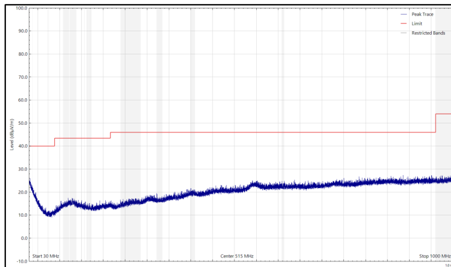
Figure 39 - CH39_LE1M_Z Plane, 2480 MHz, 30 MHz to 1 GHz, Vertical (Peak)
