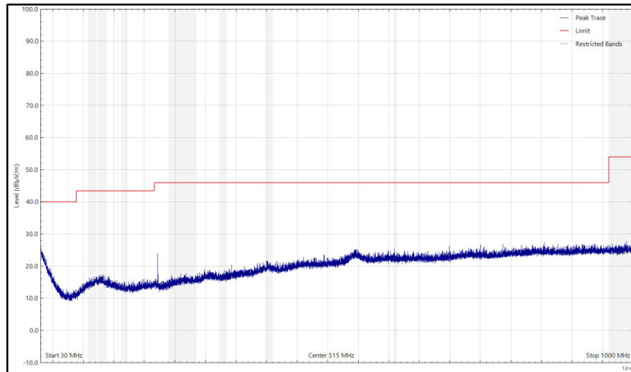
Figure 15 - CH37_LE1M_Z Plane, 2402 MHz, 30 MHz to 1 GHz, Vertical (Peak)
