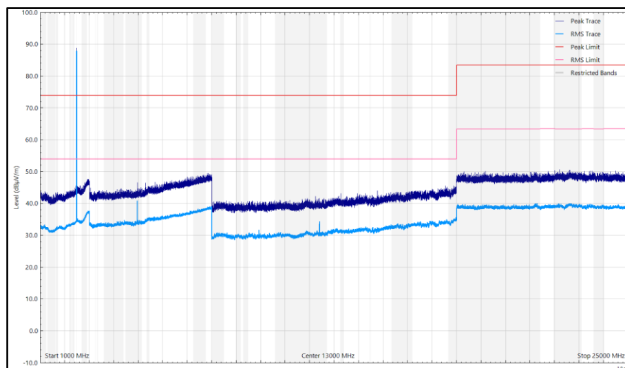
Figure 40 - CH39_LE1M_Z Plane, 2480 MHz, 1 GHz to 25 GHz, Vertical
