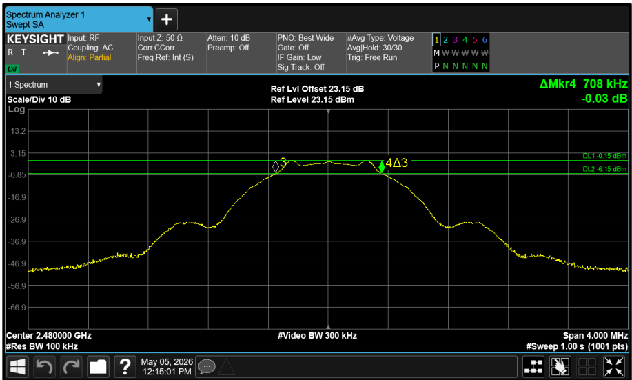
Figure 47 - SMA Pigtail (A) 2480 MHz (CH39) 6 dB Bandwidth
