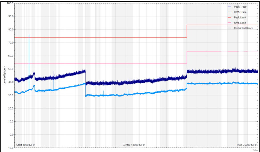
Figure 20 - CH17_LE1M_X Plane, 2440 MHz, 1 GHz to 25 GHz, Vertical
