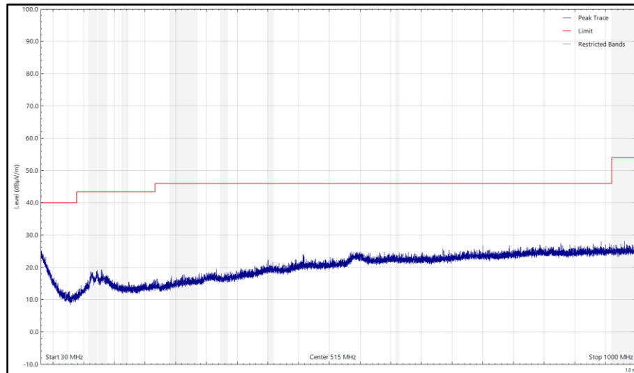
Figure 33 - CH39_LE1M_Y Plane, 2480 MHz, 30 MHz to 1 GHz, Horizontal (Peak)
