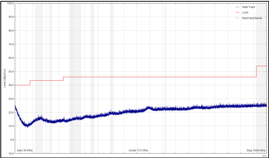
Figure 31 - CH39_LE1M_X Plane, 2480 MHz, 30 MHz to 1 GHz, Vertical (Peak)
