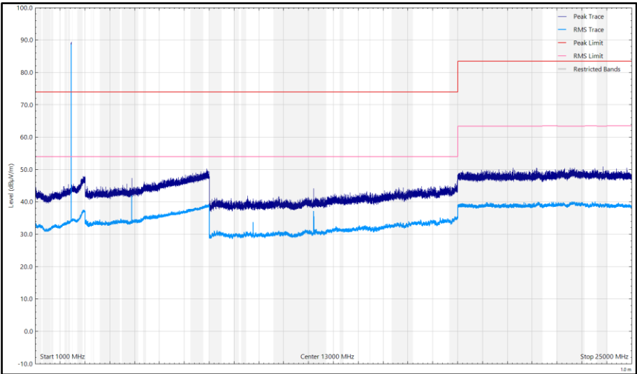
Figure 24 - CH17_LE1M_Y Plane, 2440 MHz, 1 GHz to 25 GHz, Vertical
