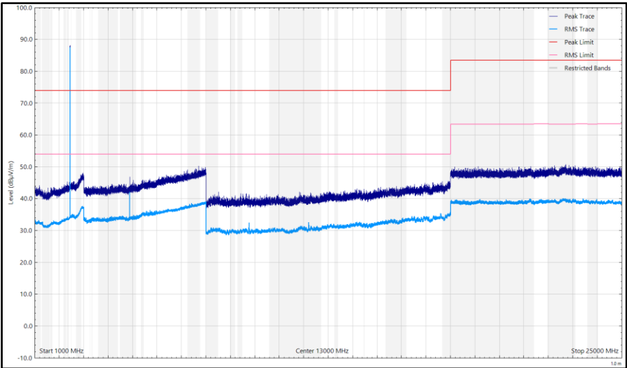
Figure 28 - CH17_LE1M_Z Plane, 2440 MHz, 1 GHz to 25 GHz, Vertical
