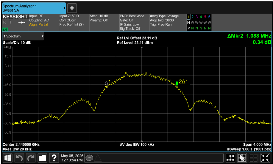
Figure 44 - SMA Pigtail (A) 2440 MHz (CH17) 99% Bandwidth
