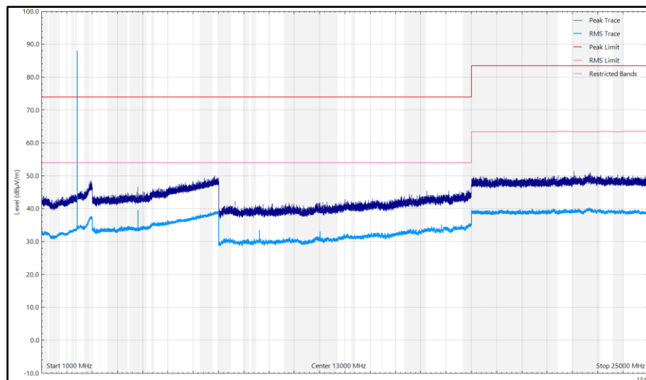
Figure 16 - CH37_LE1M_Z Plane, 2402 MHz, 1 GHz to 25 GHz, Vertical
