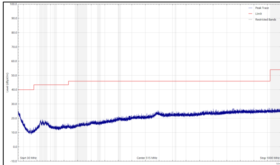
Figure 21 - CH17_LE1M_Y Plane, 2440 MHz, 30 MHz to 1 GHz, Horizontal (Peak)
