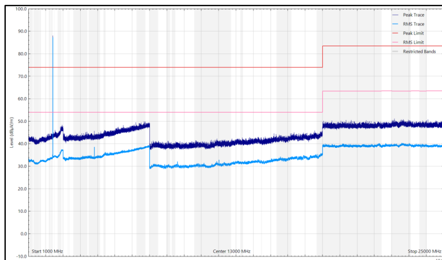
Figure 6 - CH37_LE1M_X Plane, 2402 MHz, 1 GHz to 25 GHz, Horizontal
