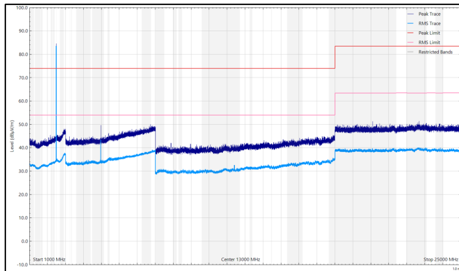
Figure 38 - CH39_LE1M_Z Plane, 2480 MHz, 1 GHz to 25 GHz, Horizontal
