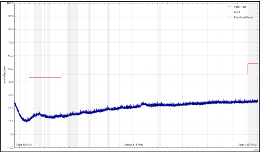
Figure 23 - CH17_LE1M_Y Plane, 2440 MHz, 30 MHz to 1 GHz, Vertical (Peak)
