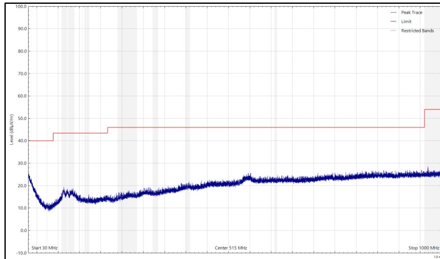
Figure 13 - CH37_LE1M_Z Plane, 2402 MHz, 30 MHz to 1 GHz, Horizontal (Peak)
