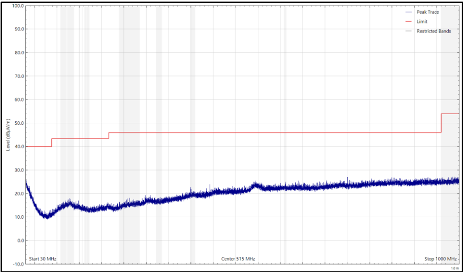
Figure 19 - CH17_LE1M_X Plane, 2440 MHz, 30 MHz to 1 GHz, Vertical (Peak)
