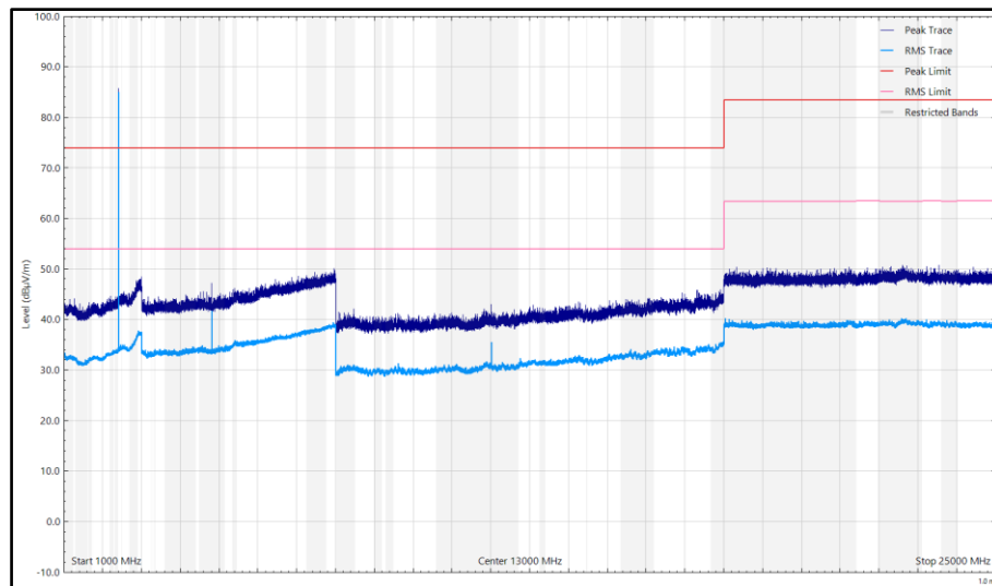
Figure 14 - CH37_LE1M_Z Plane, 2402 MHz, 1 GHz to 25 GHz, Horizontal
