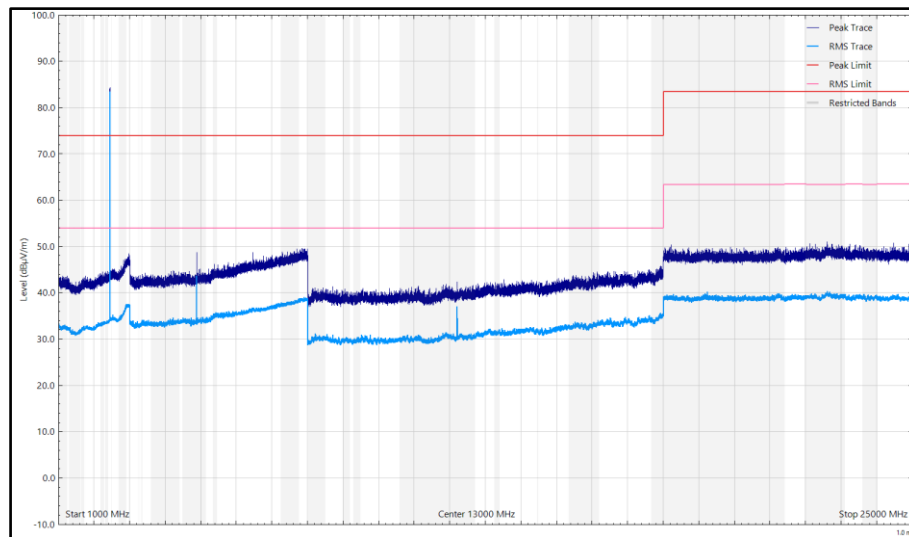
Figure 26 - CH17_LE1M_Z Plane, 2440 MHz, 1 GHz to 25 GHz, Horizontal
