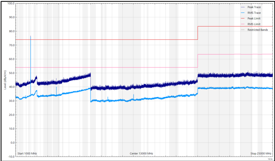
Figure 8 - CH37_LE1M_X Plane, 2402 MHz, 1 GHz to 25 GHz, Vertical
