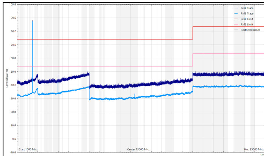
Figure 30 - CH39_LE1M_X Plane, 2480 MHz, 1 GHz to 25 GHz, Horizontal
