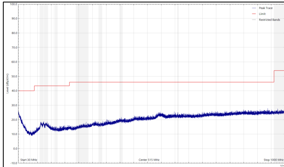
Figure 37 - CH39_LE1M_Z Plane, 2480 MHz, 30 MHz to 1 GHz, Horizontal (Peak)
