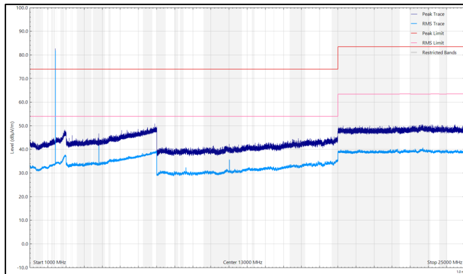
Figure 10 - CH37_LE1M_Y Plane, 2402 MHz, 1 GHz to 25 GHz, Horizontal
