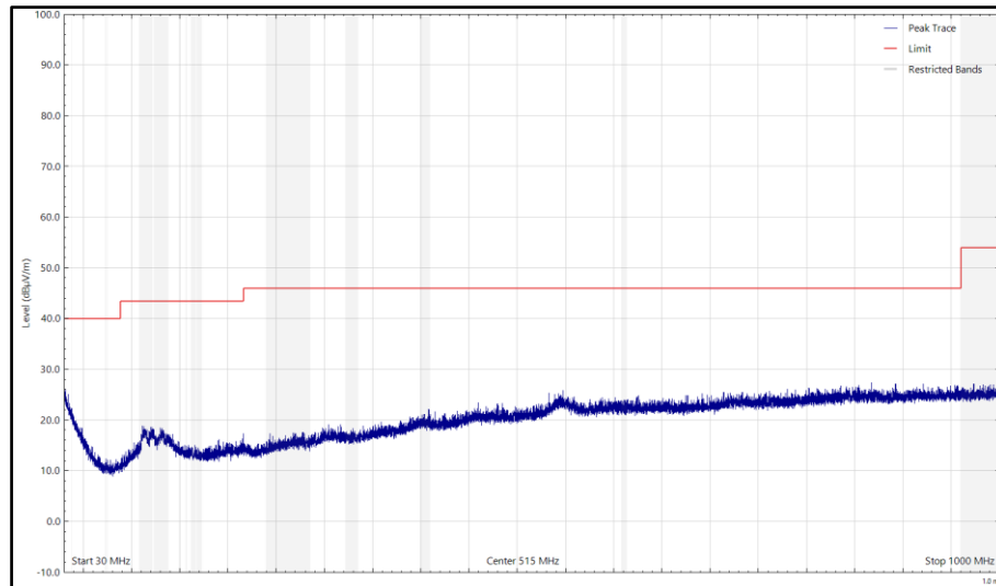
Figure 17 - CH17_LE1M_X Plane, 2440 MHz, 30 MHz to 1 GHz, Horizontal (Peak)
