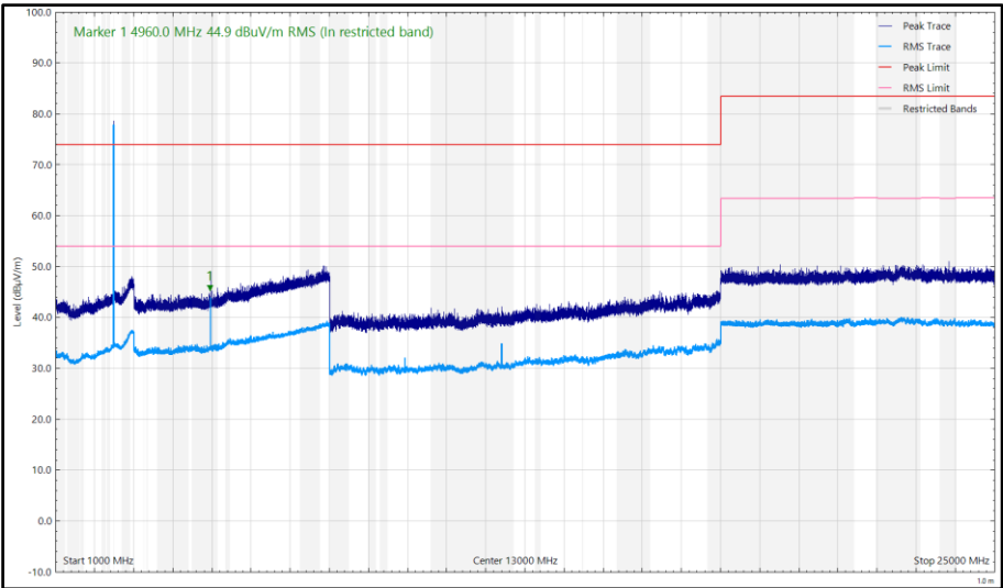
Figure 32 - CH39_LE1M_X Plane, 2480 MHz, 1 GHz to 25 GHz, Vertical
