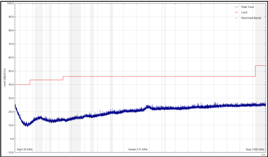
Figure 11 - CH37_LE1M_Y Plane, 2402 MHz, 30 MHz to 1 GHz, Vertical (Peak)
