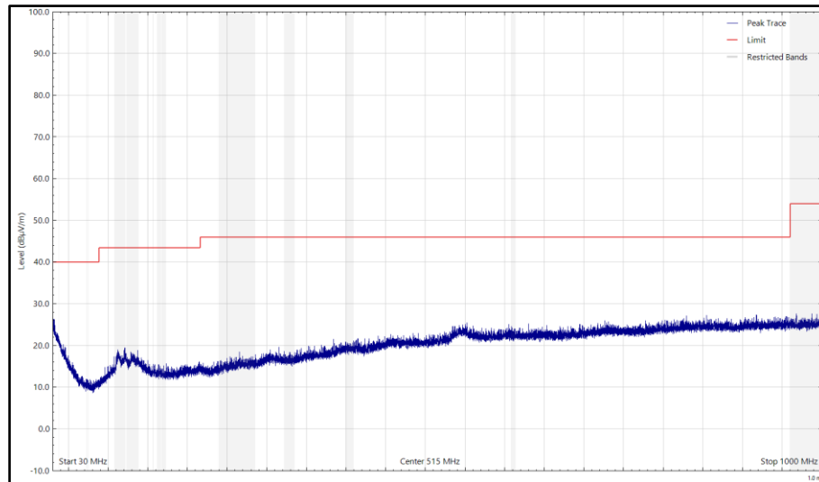
Figure 29 - CH39_LE1M_X Plane, 2480 MHz, 30 MHz to 1 GHz, Horizontal (Peak)
