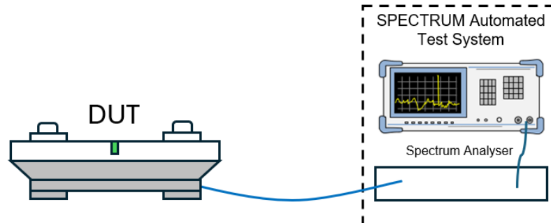
Figure 52 – Test Setup for Power Spectral Density
