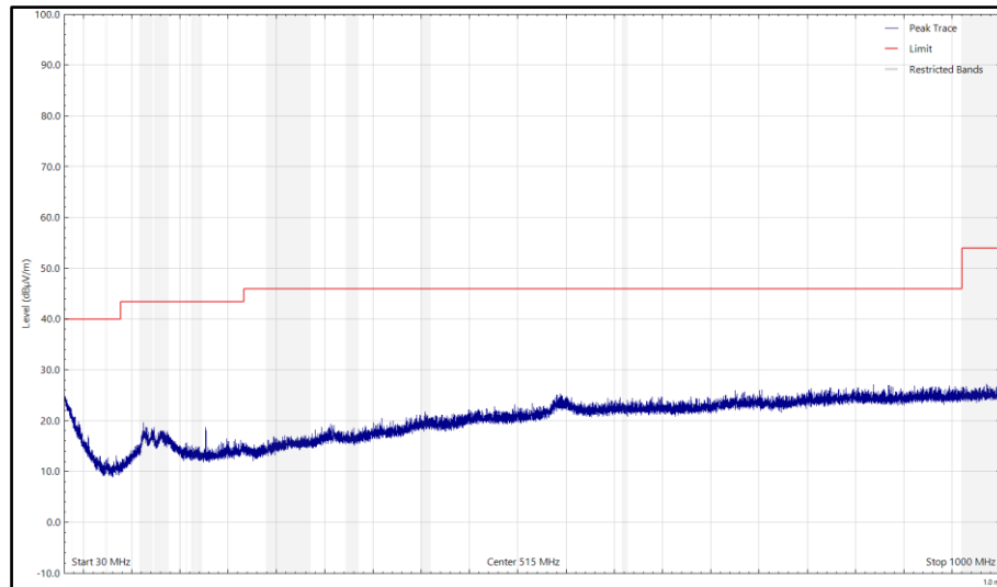
Figure 9 - CH37_LE1M_Y Plane, 2402 MHz, 30 MHz to 1 GHz, Horizontal (Peak)
