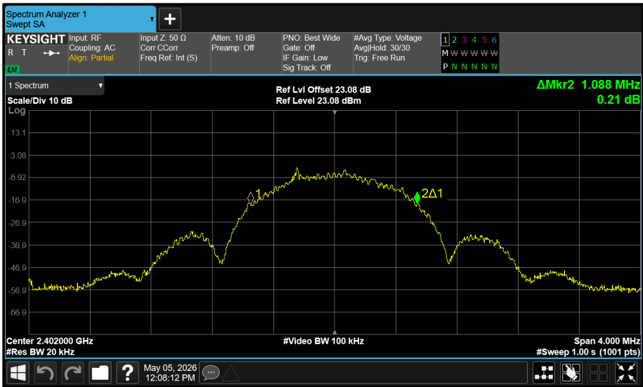
Figure 42 - SMA Pigtail (A) 2402 MHz (CH37) 99% Bandwidth
