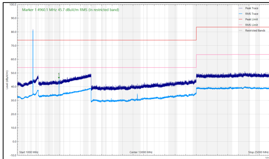
Figure 34 - CH39_LE1M_Y Plane, 2480 MHz, 1 GHz to 25 GHz, Horizontal
