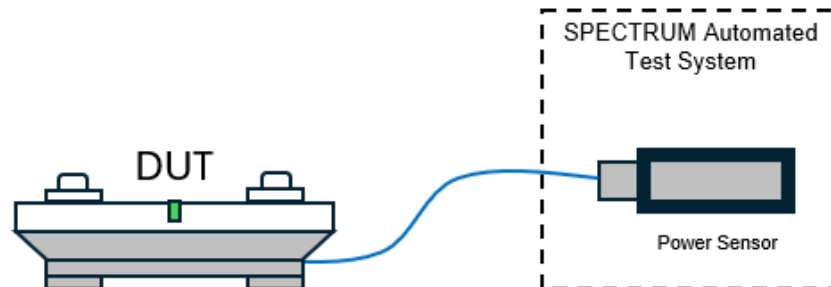
Figure 48 – Test Setup for Maximum Conducted Output Power
