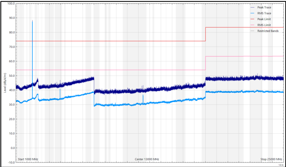
Figure 36 - CH39_LE1M_Y Plane, 2480 MHz, 1 GHz to 25 GHz, Vertical
