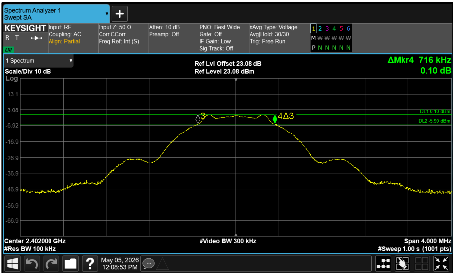
Figure 43 - SMA Pigtail (A) 2402 MHz (CH37) 6 dB Bandwidth
