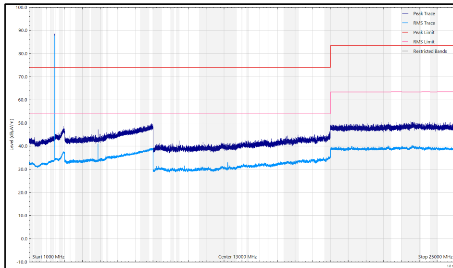
Figure 18 - CH17_LE1M_X Plane, 2440 MHz, 1 GHz to 25 GHz, Horizontal
