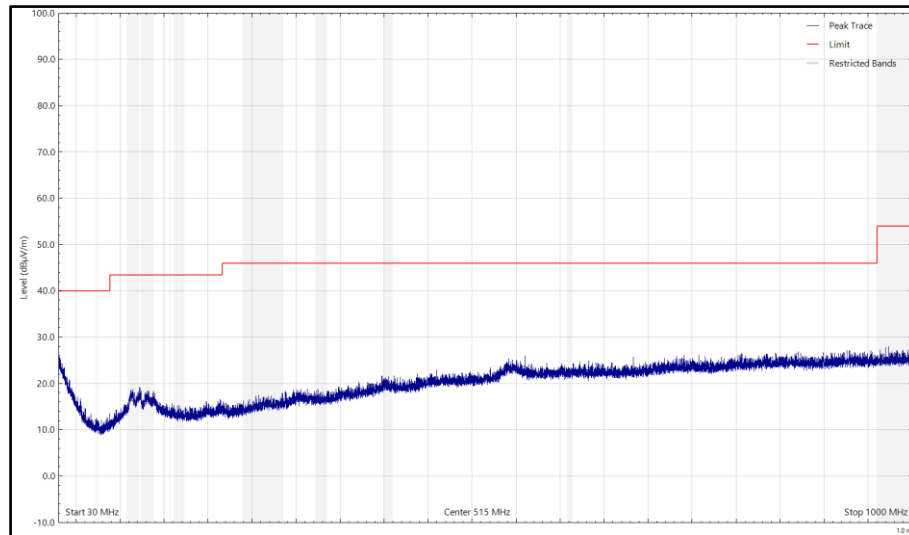
Figure 25 - CH17_LE1M_Z Plane, 2440 MHz, 30 MHz to 1 GHz, Horizontal (Peak)
