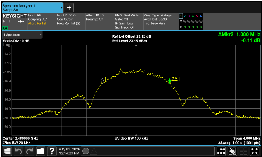
Figure 46 - SMA Pigtail (A) 2480 MHz (CH39) 99% Bandwidth
