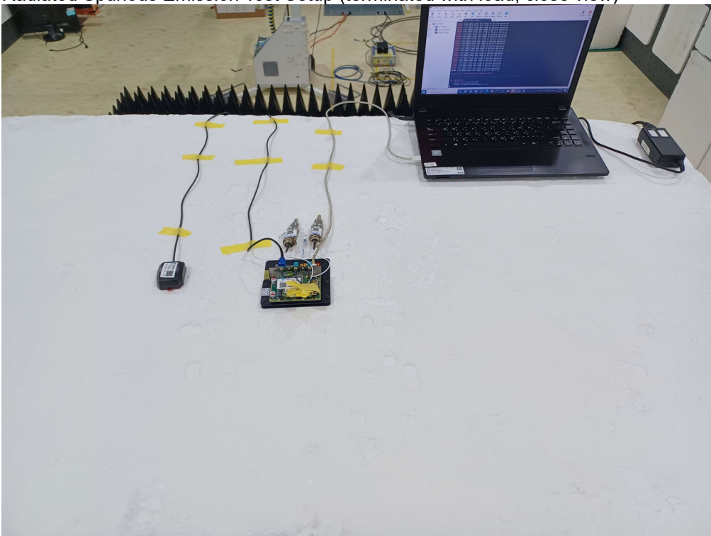
Radiated Spurious Emission Test Setup (terminated with load, close view)
