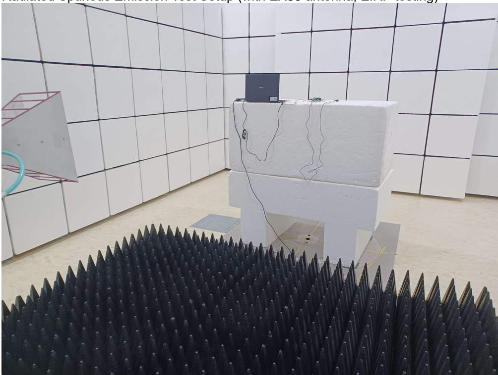
Radiated Spurious Emission Test Setup (with EX55 antenna, EIRP testing)
