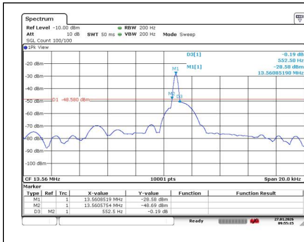
20 dB Bandwidth
