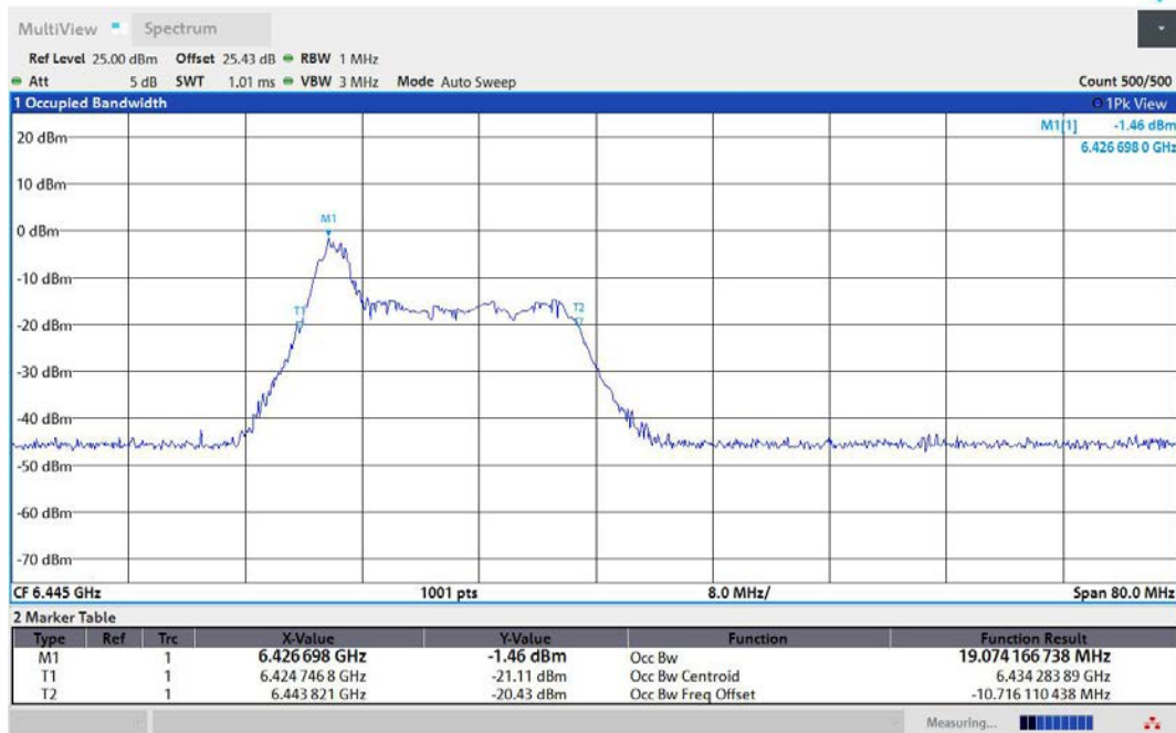
11AX40MIMO-Ant2-6445-26Tone-RU0-PASS
