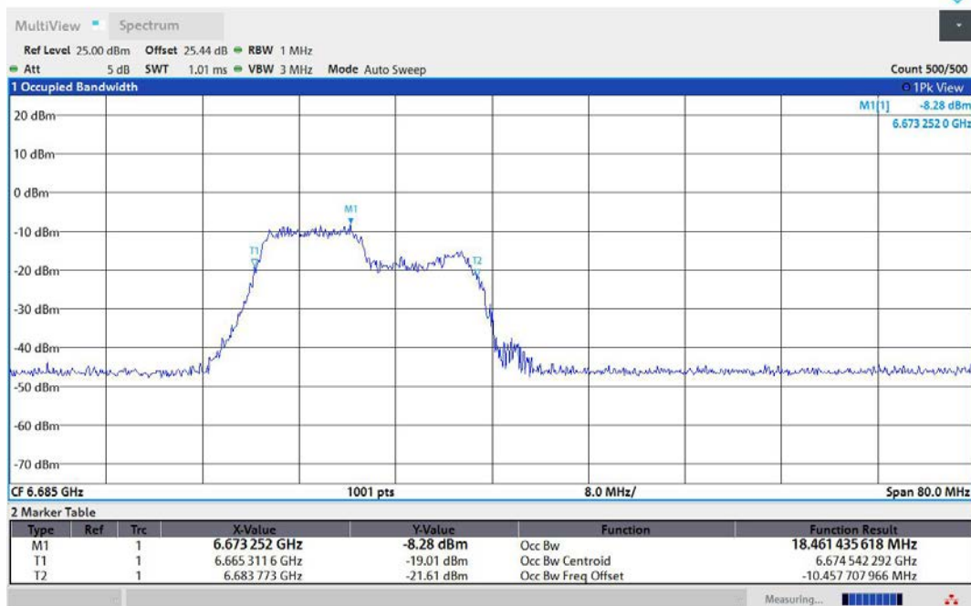
11AX40MIMO-Ant1-6685-106Tone-RU53-PASS
