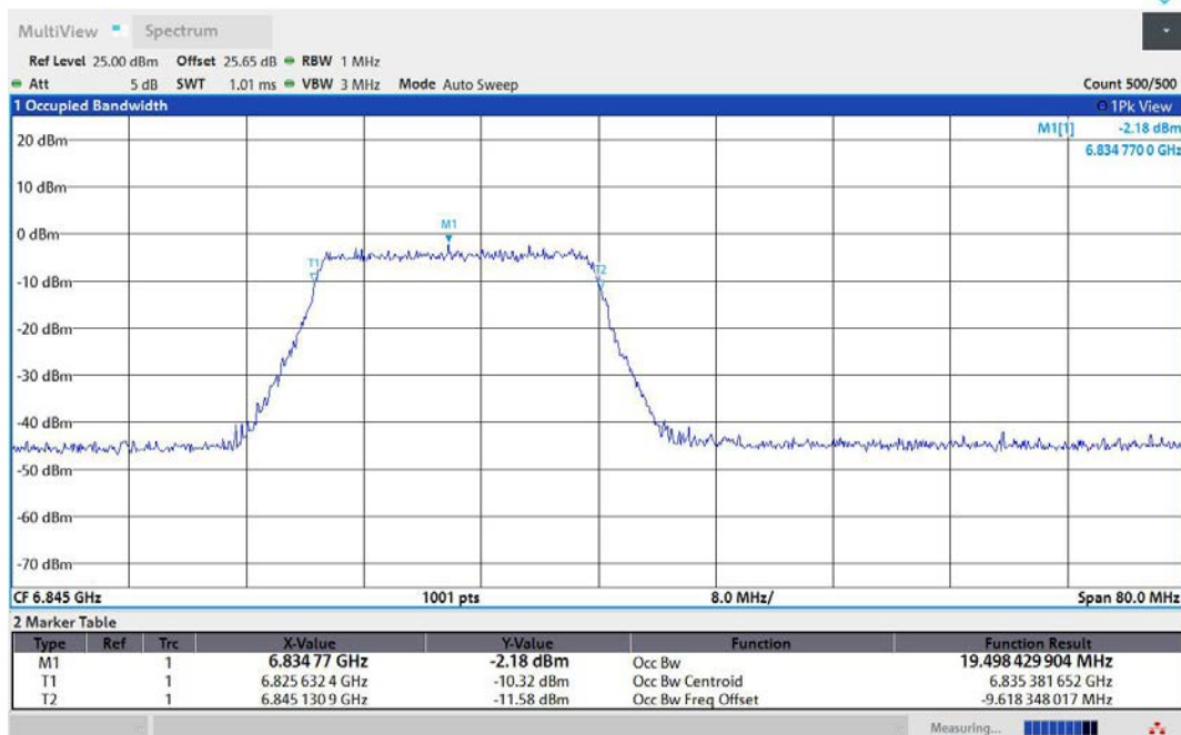
11AX40MIMO-Ant2-6845-242Tone-RU61-PASS
