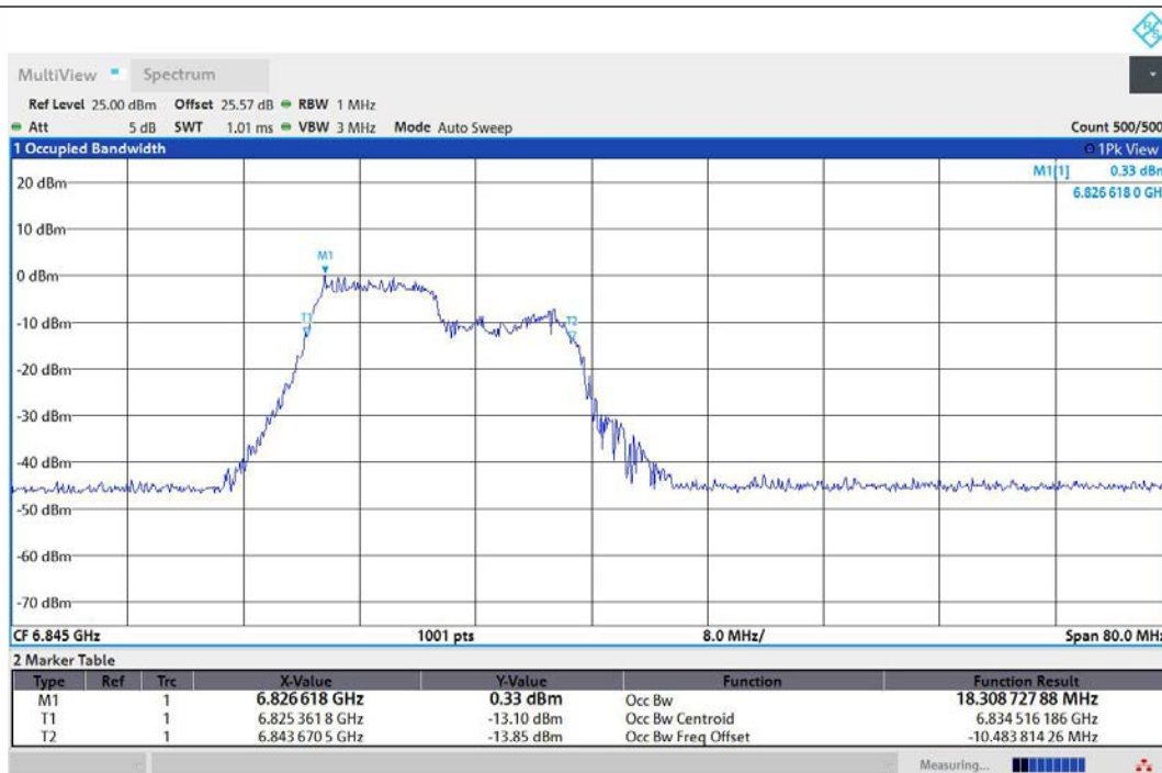
11AX40MIMO-Ant1-6845-106Tone-RU53-PASS
