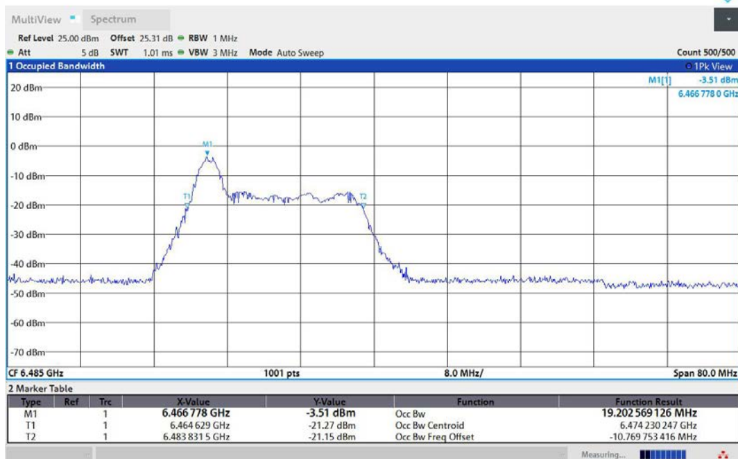
11AX40MIMO-Ant2-6485-26Tone-RU0-PASS
