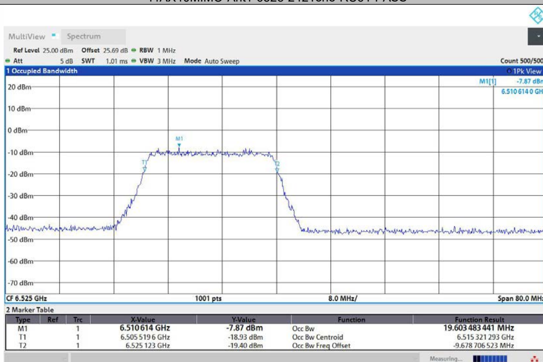
11AX40MIMO-Ant2-6525-242Tone-RU61-PASS
