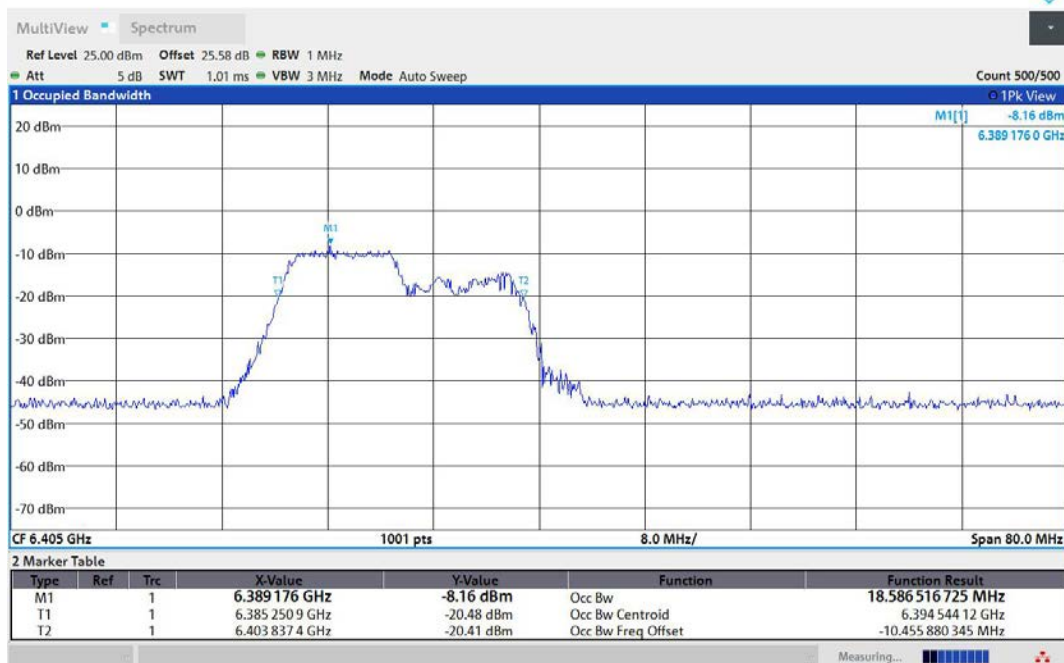
11AX40MIMO-Ant2-6405-106Tone-RU53-PASS
