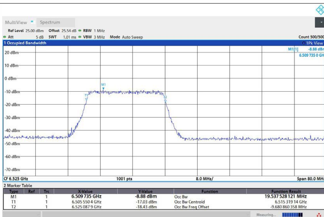
11AX40MIMO-Ant1-6525-242Tone-RU61-PASS
