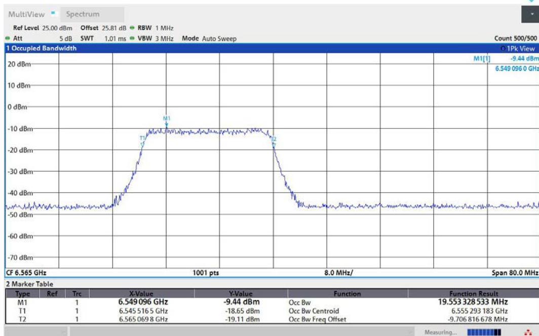
11AX40MIMO-Ant1-6565-242Tone-RU61-PASS
