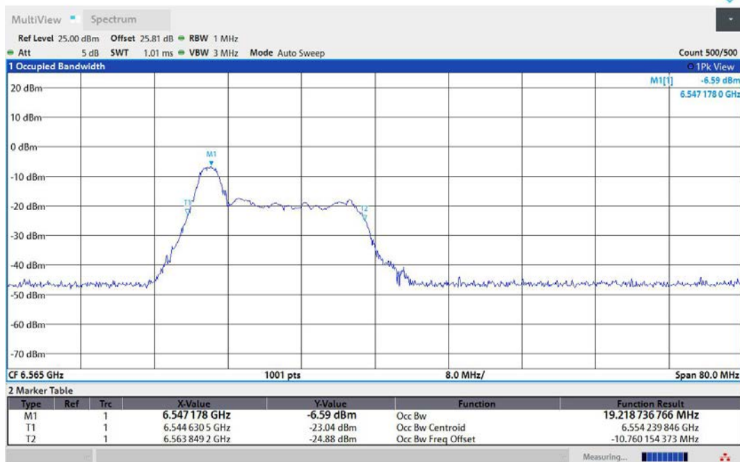
11AX40MIMO-Ant1-6565-26Tone-RU0-PASS
