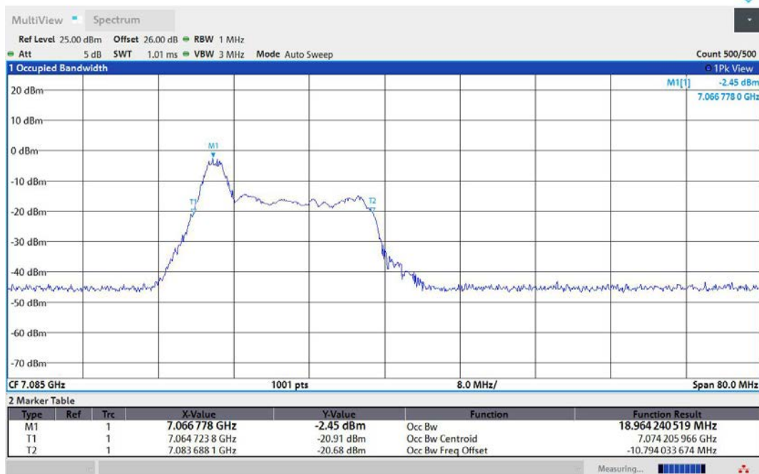
11AX40MIMO-Ant1-7085-26Tone-RU0-PASS
