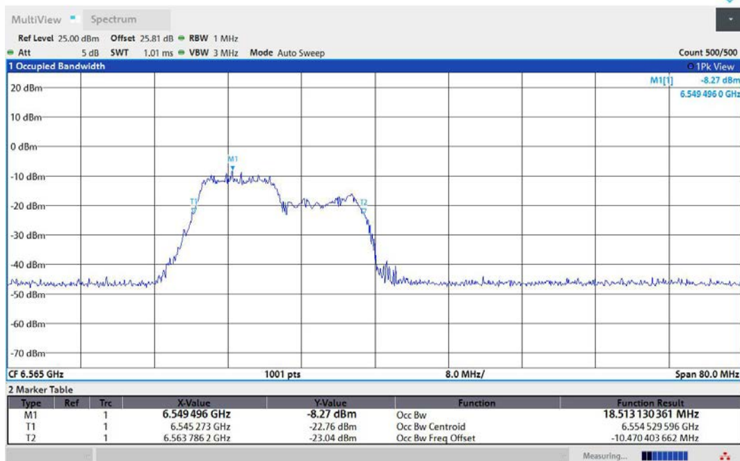
11AX40MIMO-Ant1-6565-106Tone-RU53-PASS
