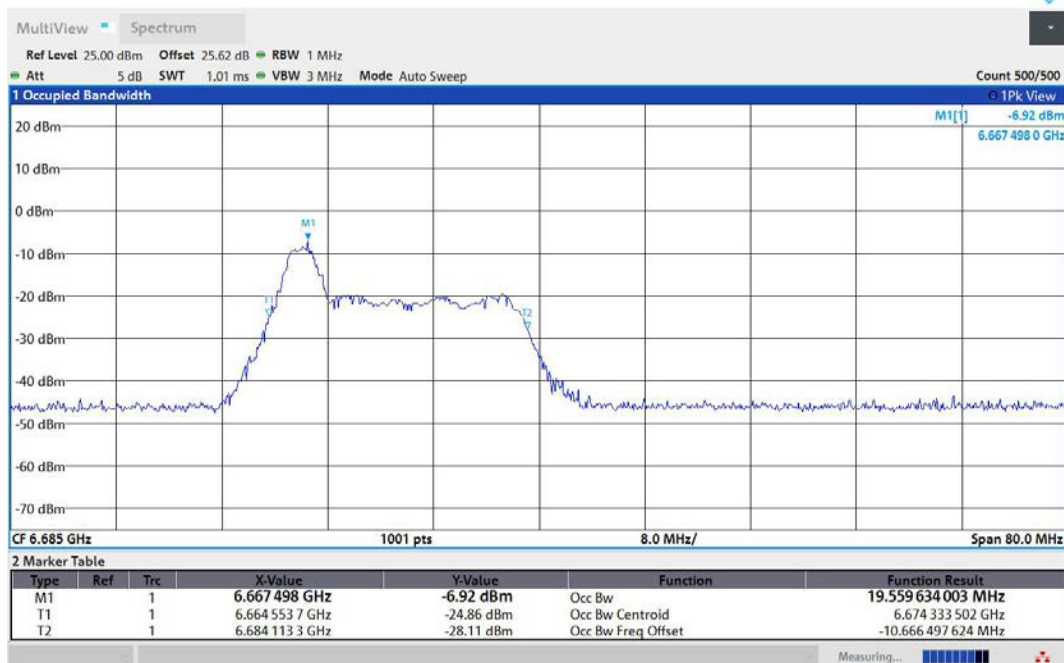
11AX40MIMO-Ant2-6685-26Tone-RU0-PASS
