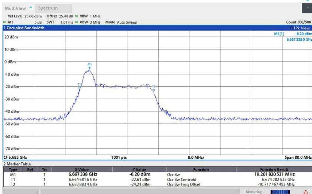
11AX40MIMO-Ant1-6685-26Tone-RU0-PASS
