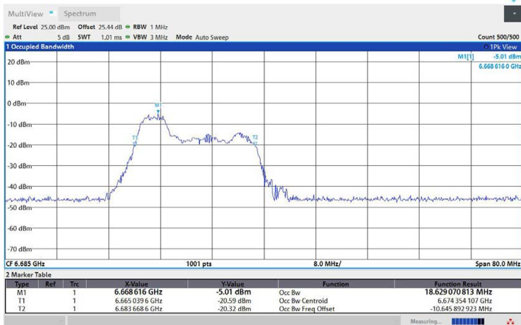
11AX40MIMO-Ant1-6685-52Tone-RU37-PASS
