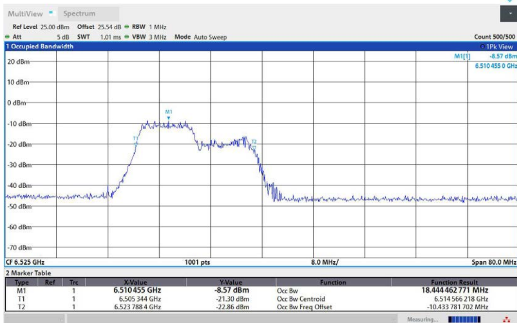
11AX40MIMO-Ant1-6525-106Tone-RU53-PASS
