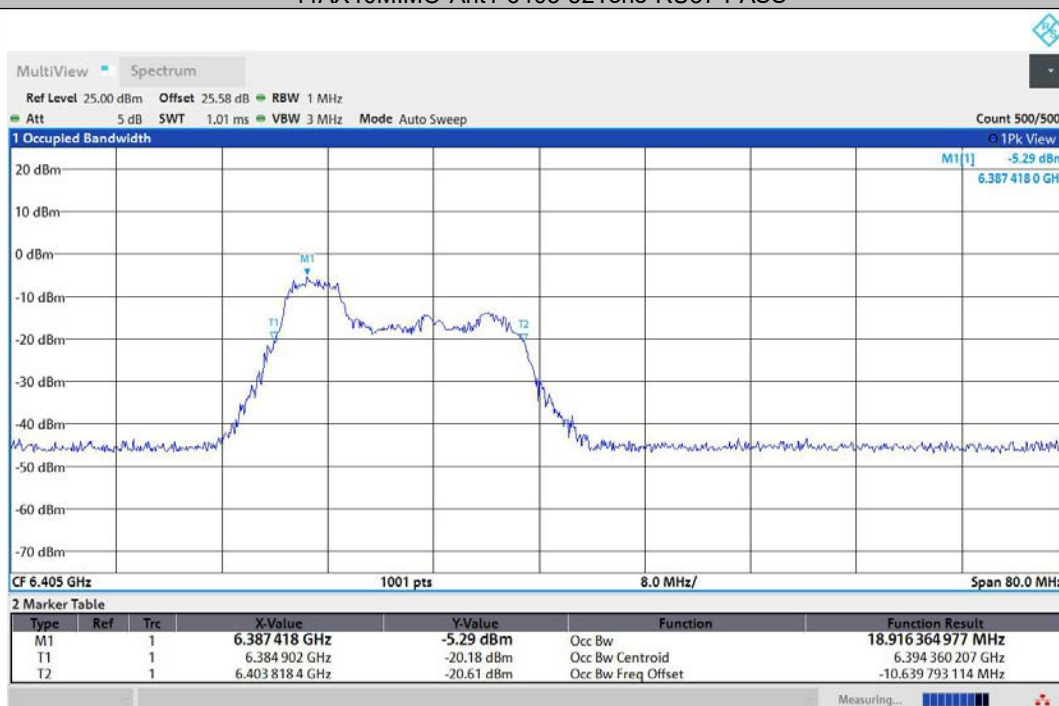
11AX40MIMO-Ant2-6405-52Tone-RU37-PASS
