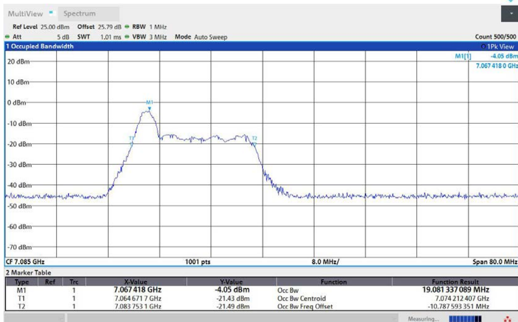
11AX40MIMO-Ant2-7085-26Tone-RU0-PASS
