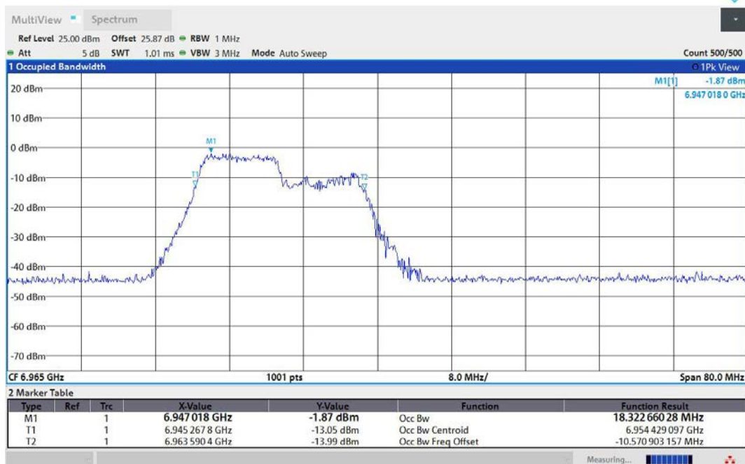
11AX40MIMO-Ant2-6965-106Tone-RU53-PASS
