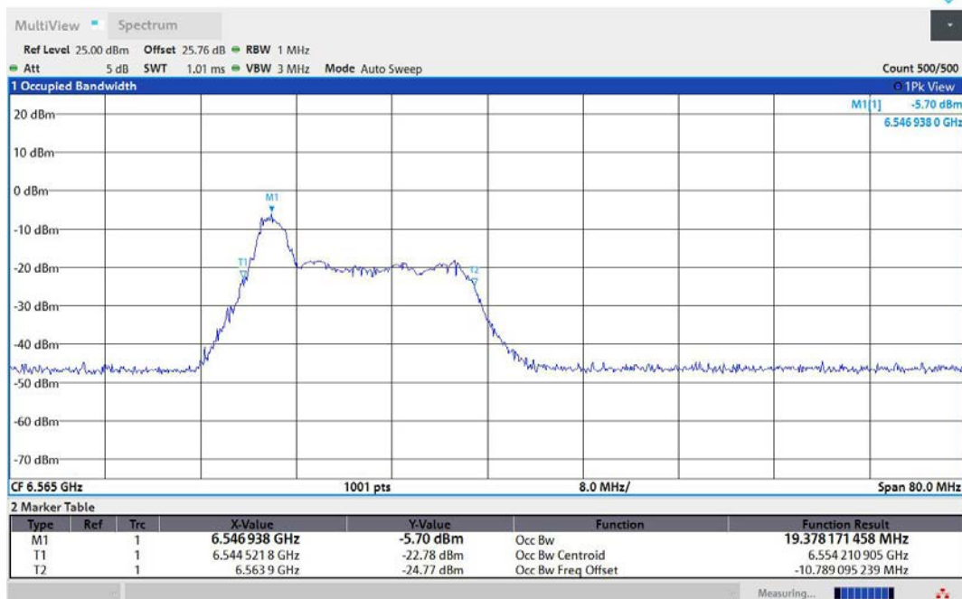
11AX40MIMO-Ant2-6565-26Tone-RU0-PASS
