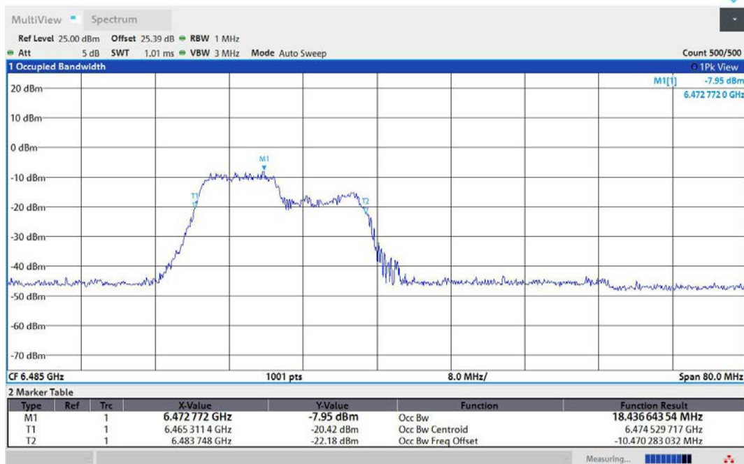
11AX40MIMO-Ant1-6485-106Tone-RU53-PASS
