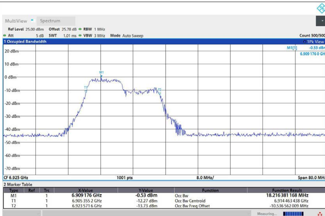
11AX40MIMO-Ant1-6925-106Tone-RU53-PASS
