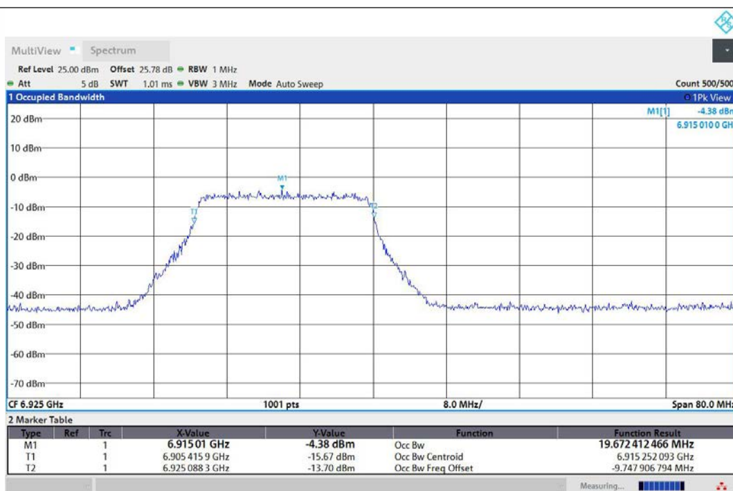
11AX40MIMO-Ant1-6925-242Tone-RU61-PASS
