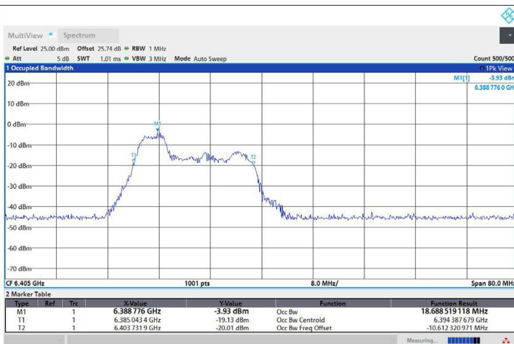
11AX40MIMO-Ant1-6405-52Tone-RU37-PASS
