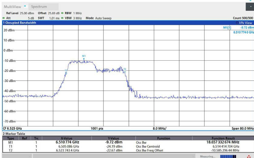
11AX40MIMO-Ant2-6525-106Tone-RU53-PASS
