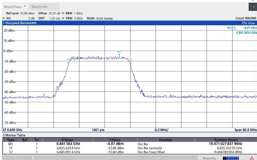
11AX40MIMO-Ant1-6845-242Tone-RU61-PASS
