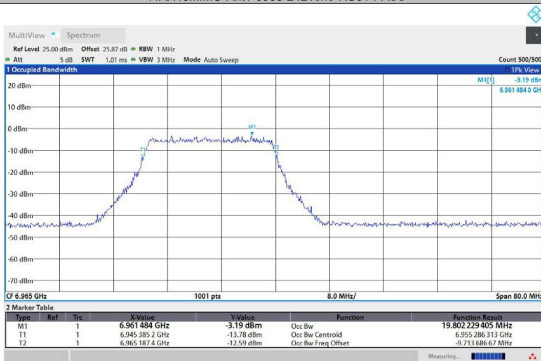
11AX40MIMO-Ant2-6965-242Tone-RU61-PASS
