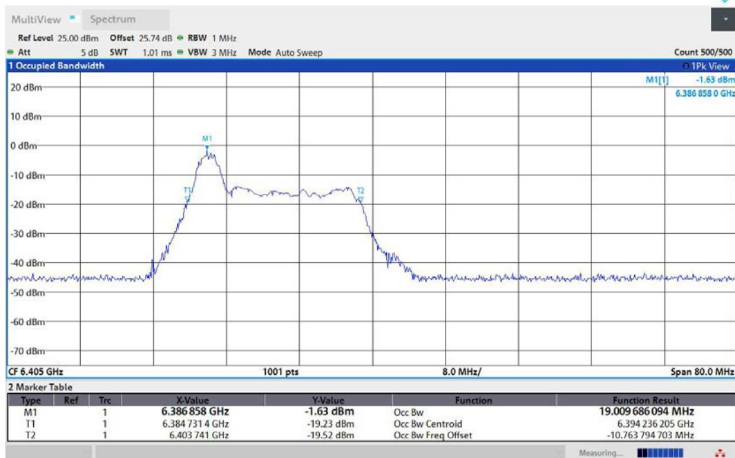
11AX40MIMO-Ant1-6405-26Tone-RU0-PASS
