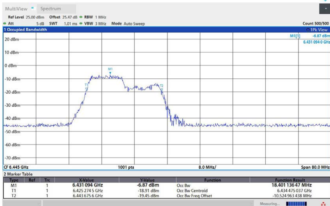
11AX40MIMO-Ant1-6445-106Tone-RU53-PASS
