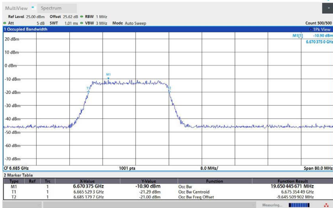
11AX40MIMO-Ant2-6685-242Tone-RU61-PASS
