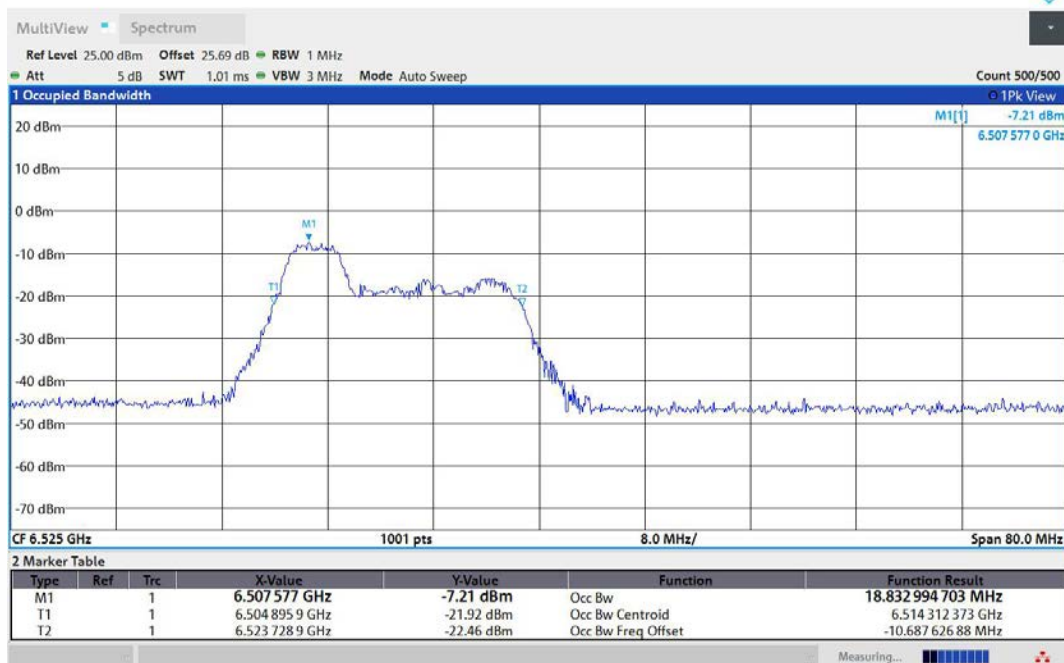
11AX40MIMO-Ant2-6525-52Tone-RU37-PASS
