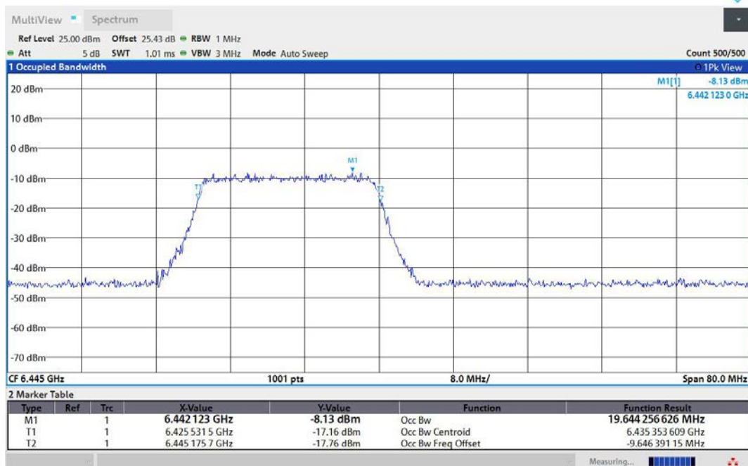
11AX40MIMO-Ant2-6445-242Tone-RU61-PASS
