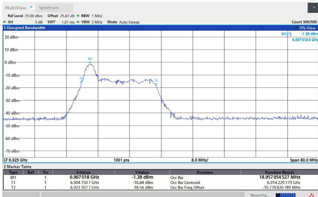
11AX40MIMO-Ant2-6925-26Tone-RU0-PASS
