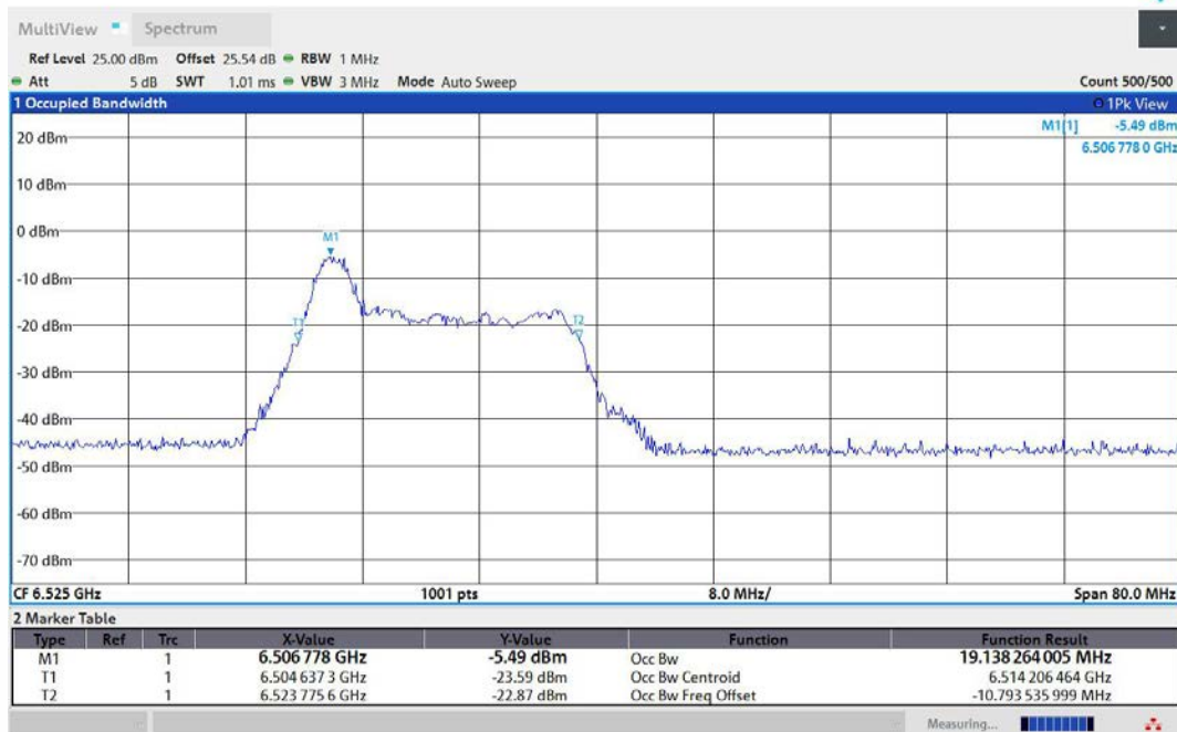
11AX40MIMO-Ant1-6525-26Tone-RU0-PASS
