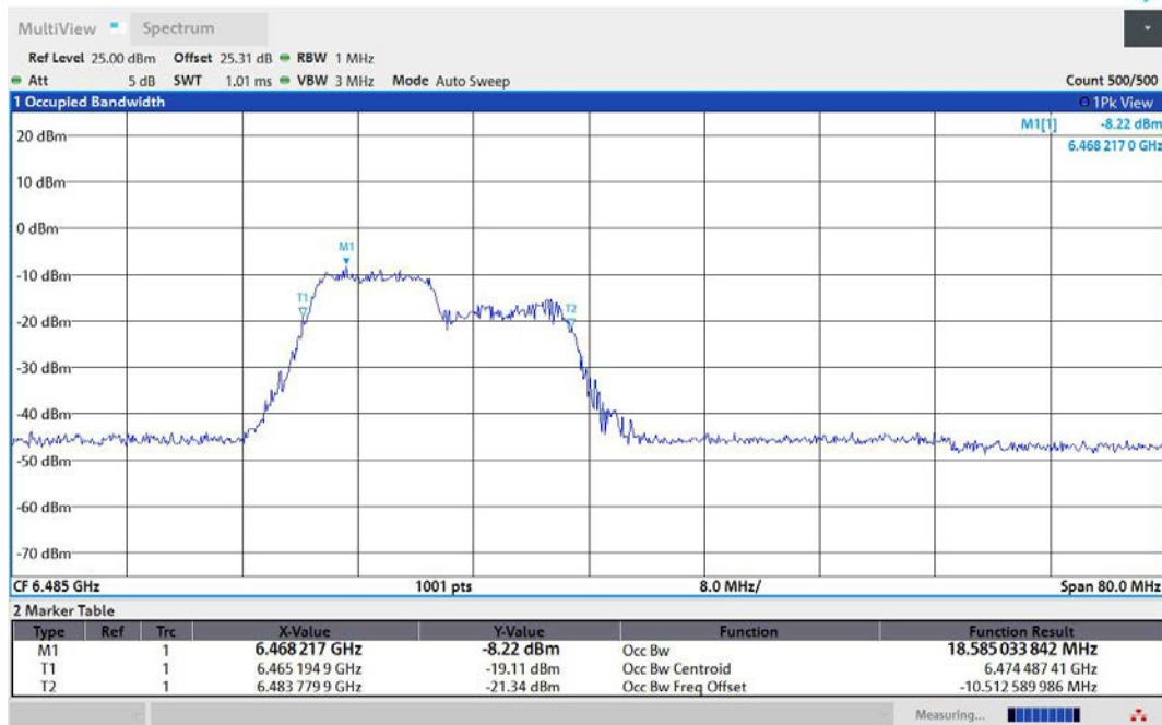
11AX40MIMO-Ant2-6485-106Tone-RU53-PASS
