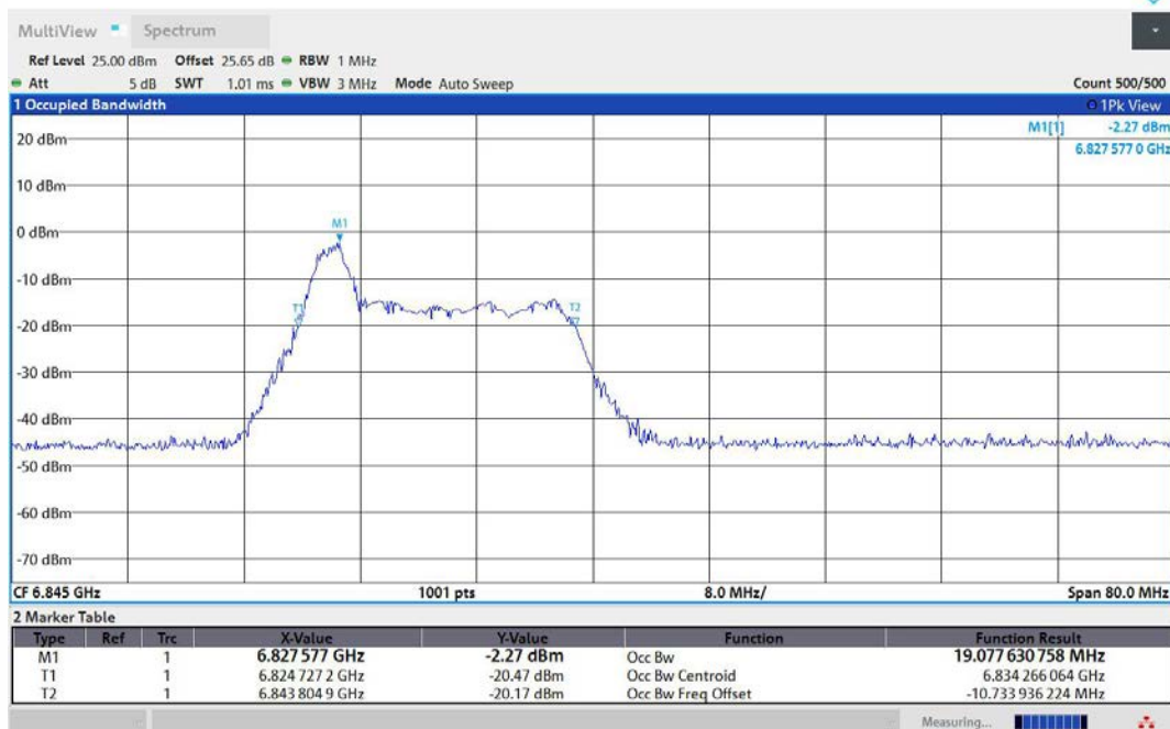
11AX40MIMO-Ant2-6845-26Tone-RU0-PASS
