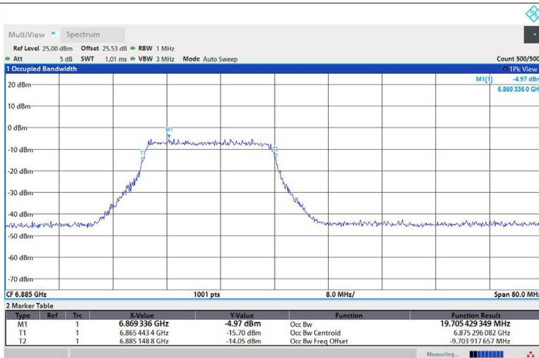
11AX40MIMO-Ant1-6885-242Tone-RU61-PASS
