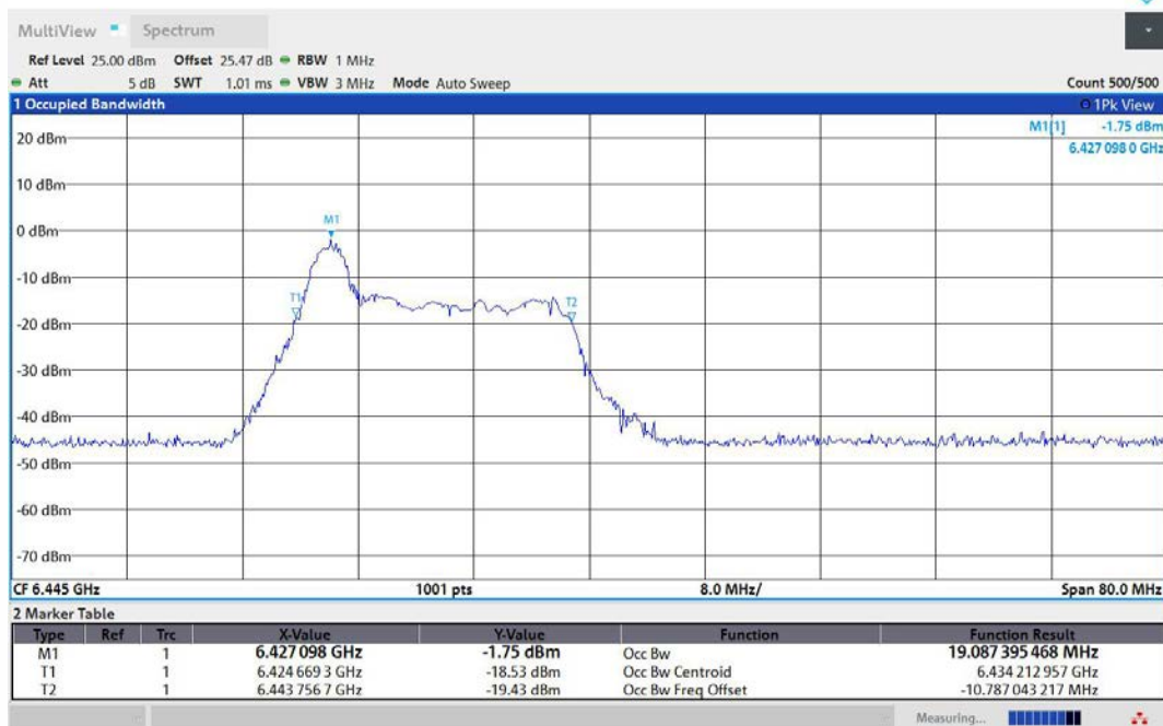
11AX40MIMO-Ant1-6445-26Tone-RU0-PASS
