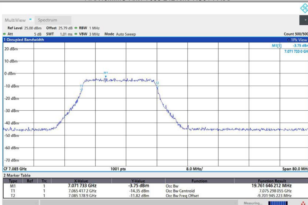
11AX40MIMO-Ant2-7085-242Tone-RU61-PASS
