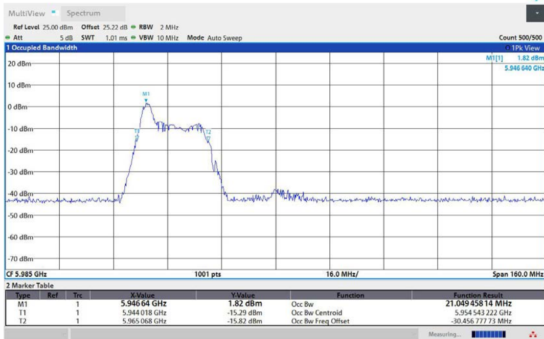
11AX80MIMO-Ant2-5985-26Tone-RU0-PASS
