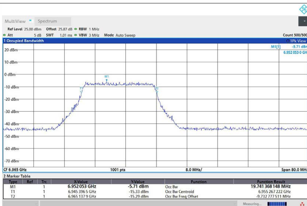
11AX40MIMO-Ant1-6965-242Tone-RU61-PASS
