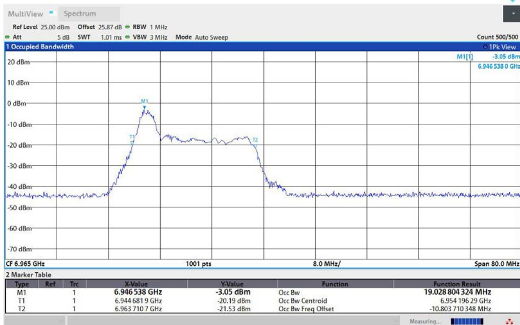
11AX40MIMO-Ant1-6965-26Tone-RU0-PASS
