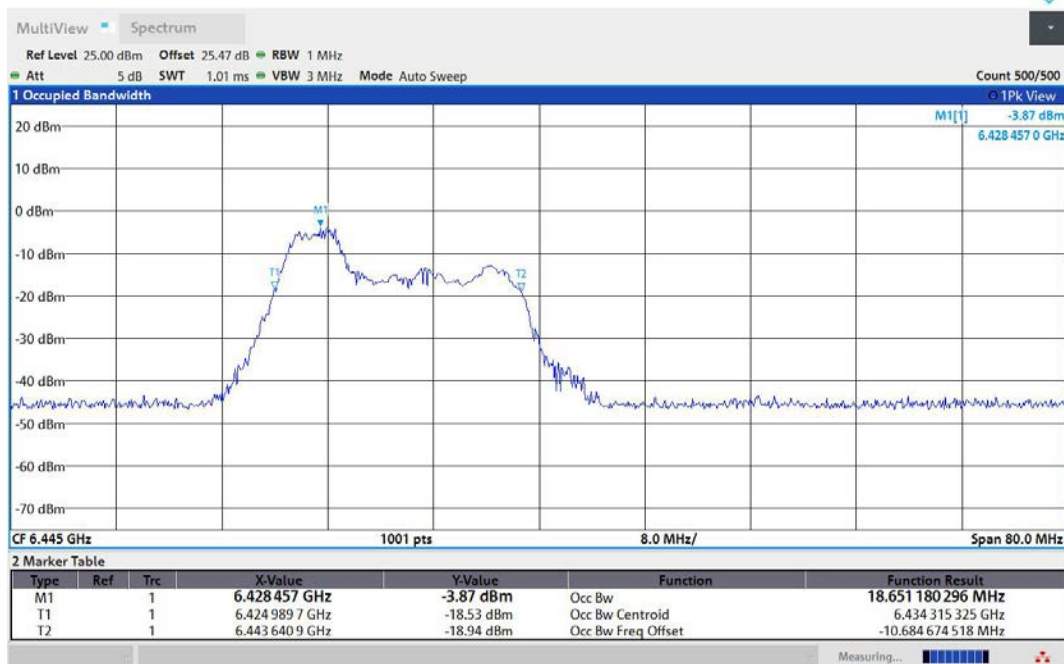
11AX40MIMO-Ant1-6445-52Tone-RU37-PASS
