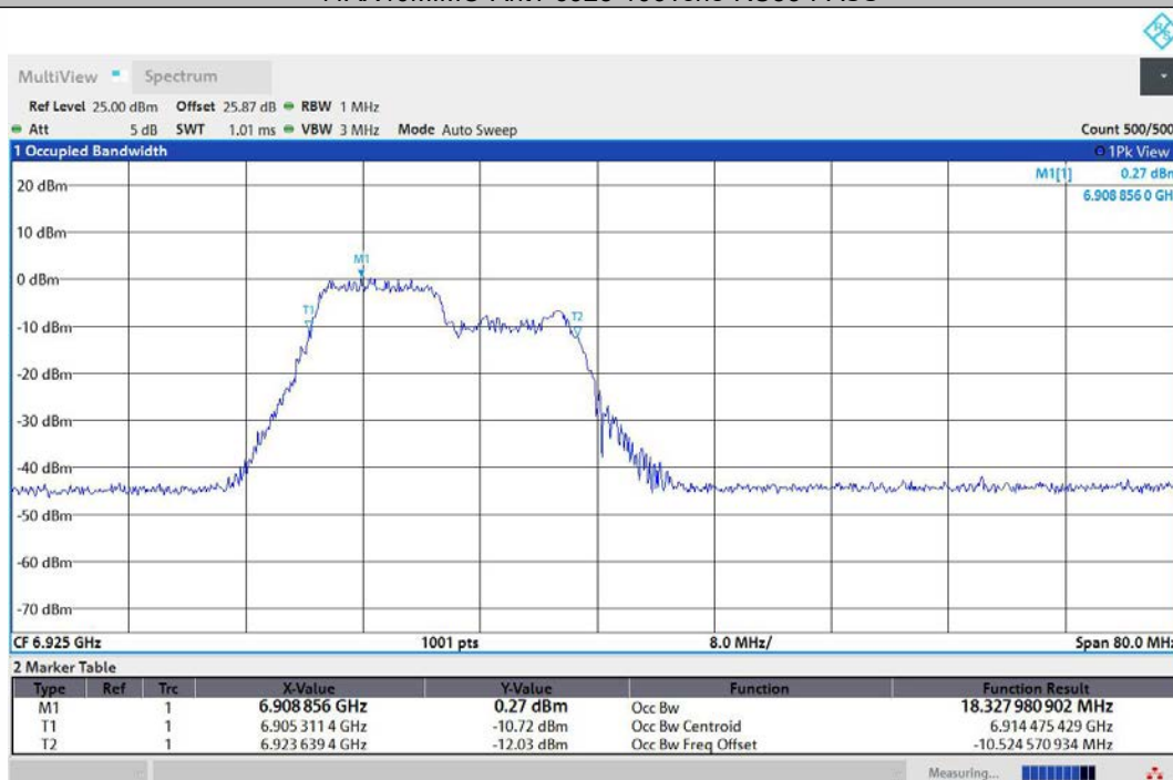
11AX40MIMO-Ant2-6925-106Tone-RU53-PASS
