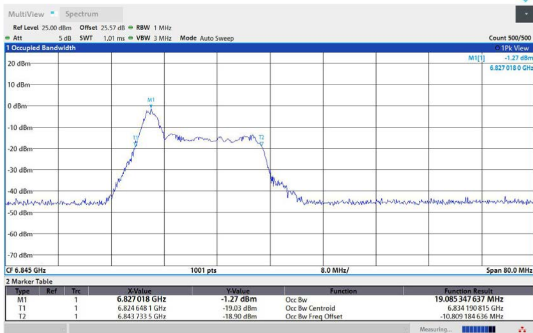
11AX40MIMO-Ant1-6845-26Tone-RU0-PASS
