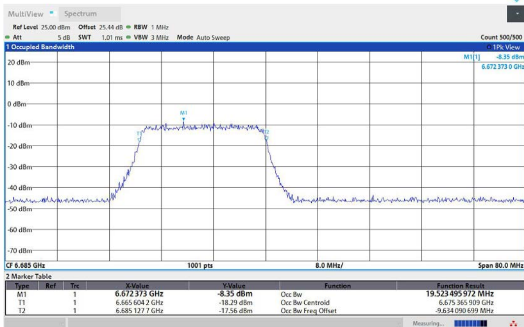
11AX40MIMO-Ant1-6685-242Tone-RU61-PASS
