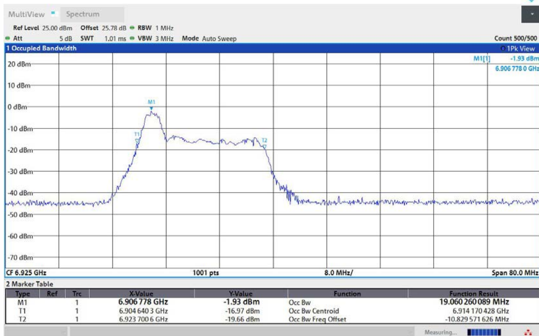
11AX40MIMO-Ant1-6925-26Tone-RU0-PASS
