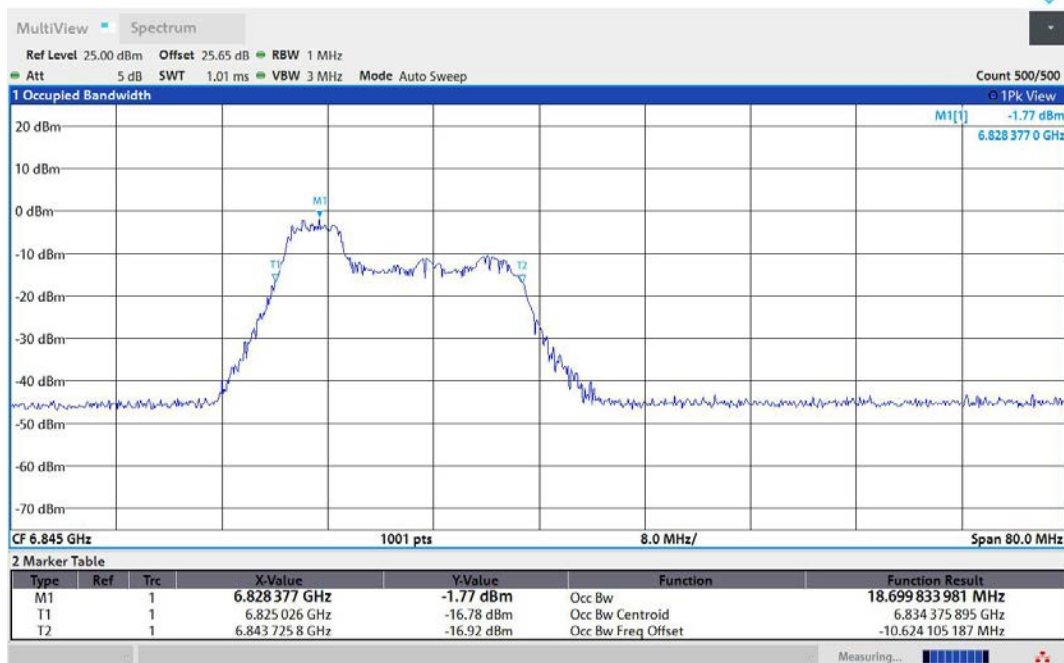
11AX40MIMO-Ant2-6845-52Tone-RU37-PASS
