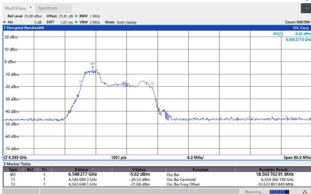
11AX40MIMO-Ant1-6565-52Tone-RU37-PASS
