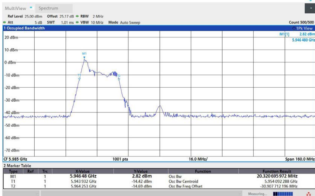
11AX80MIMO-Ant1-5985-26Tone-RU0-PASS
