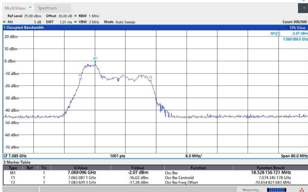
11AX40MIMO-Ant1-7085-52Tone-RU37-PASS
