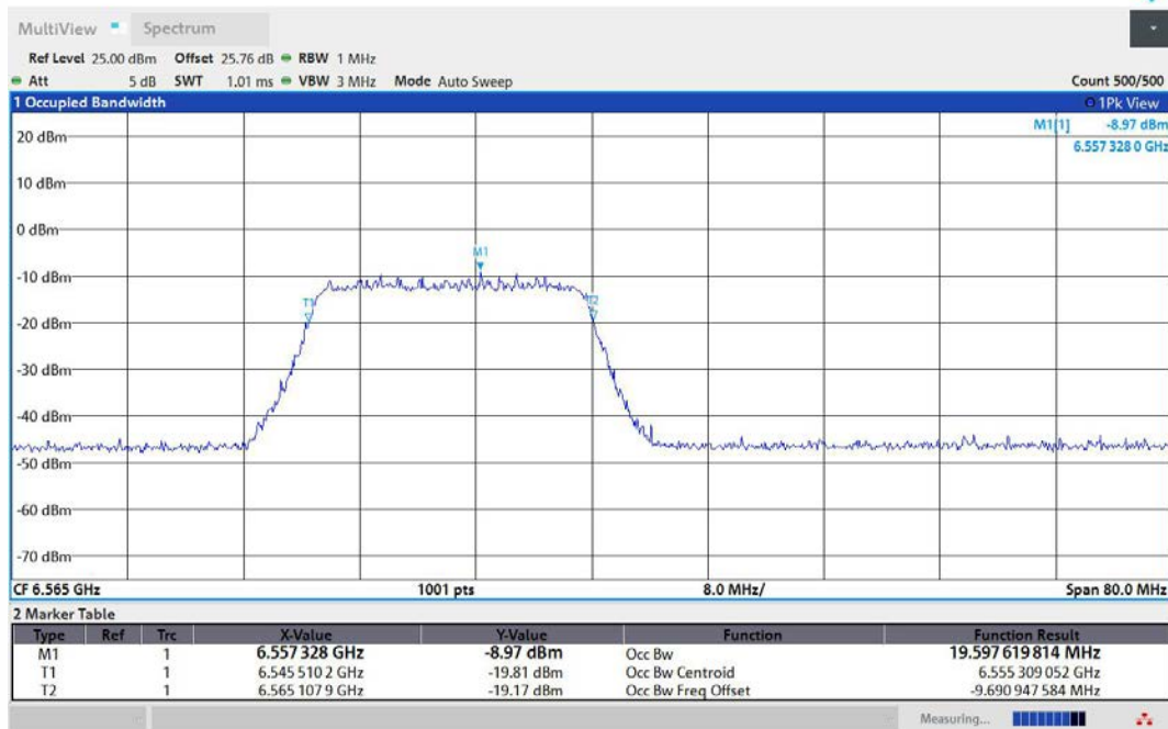
11AX40MIMO-Ant2-6565-242Tone-RU61-PASS
