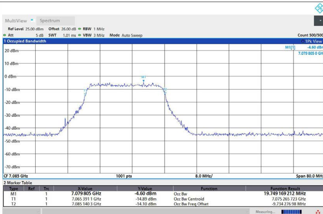
11AX40MIMO-Ant1-7085-242Tone-RU61-PASS
