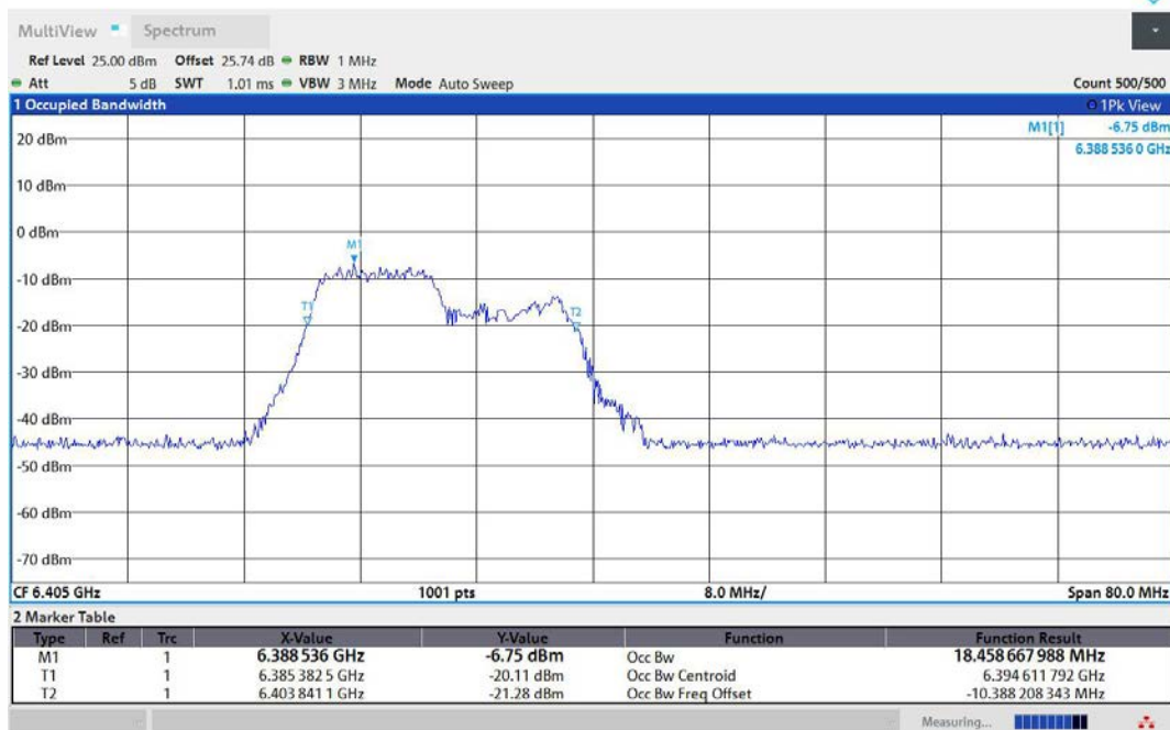
11AX40MIMO-Ant1-6405-106Tone-RU53-PASS
