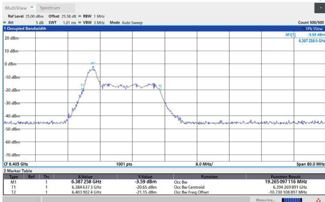
11AX40MIMO-Ant2-6405-26Tone-RU0-PASS
