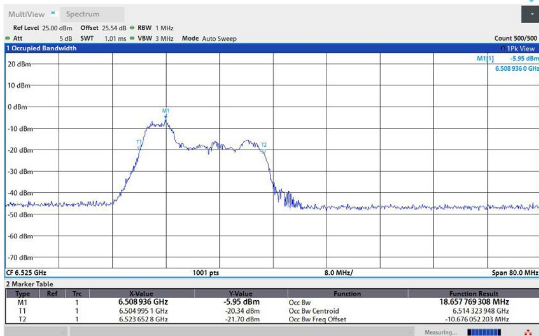
11AX40MIMO-Ant1-6525-52Tone-RU37-PASS
