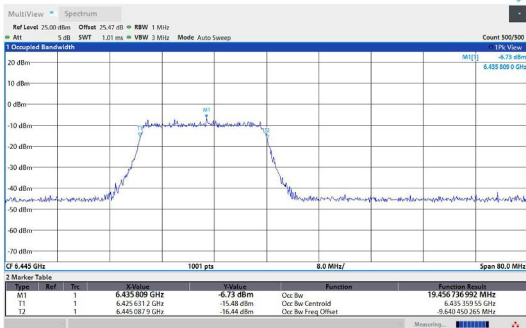
11AX40MIMO-Ant1-6445-242Tone-RU61-PASS
