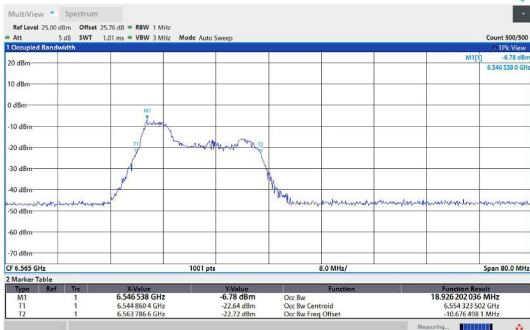
11AX40MIMO-Ant2-6565-52Tone-RU37-PASS
