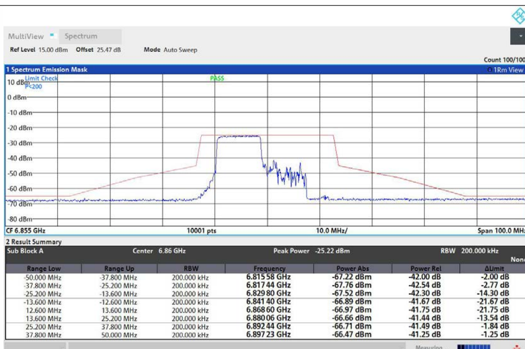
NTNV-11AX20MIMO-Ant1-6855-106Tone-RU53-PASS
