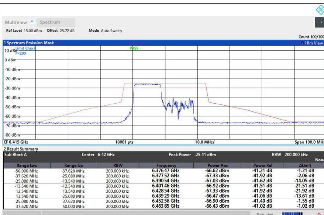
NTNV-11AX20MIMO-Ant1-6415-106Tone-RU53-PASS
