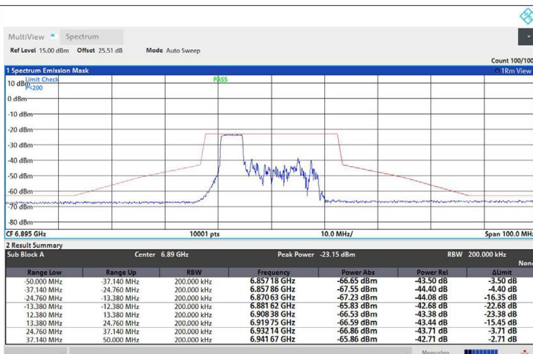
NTNV-11AX20MIMO-Ant1-6895-52Tone-RU37-PASS
