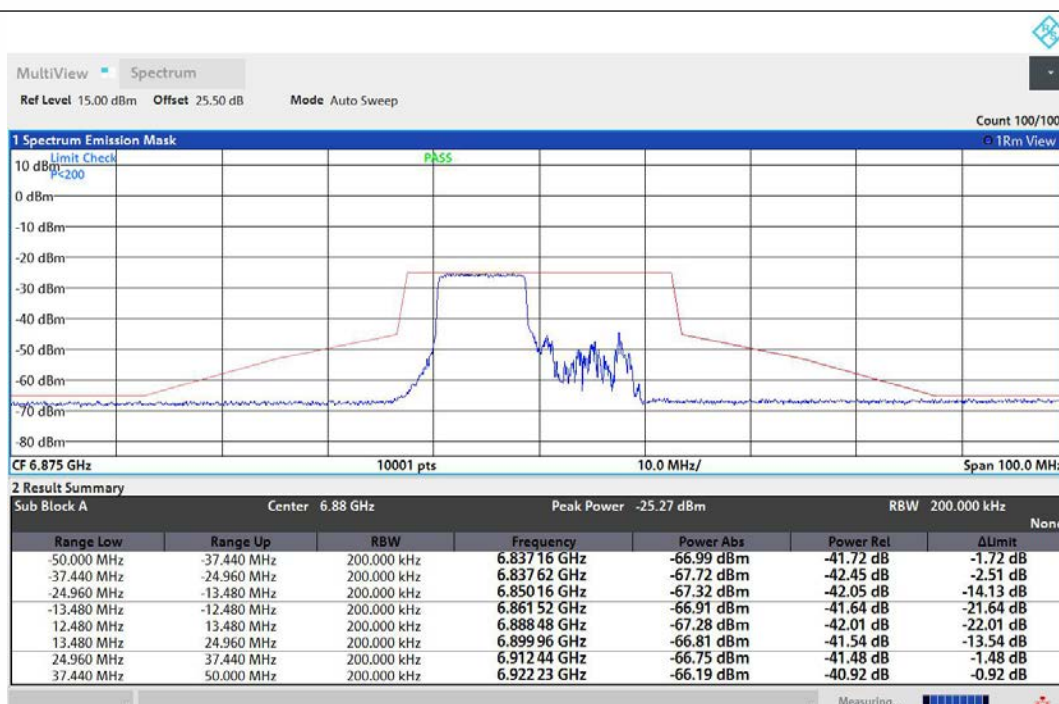
NTNV-11AX20MIMO-Ant1-6875-106Tone-RU53-PASS
