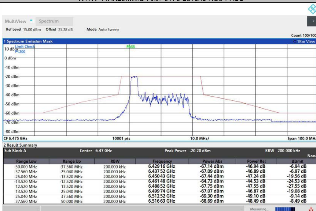
NTNV-11AX20MIMO-Ant2-6475-26Tone-RU0-PASS
