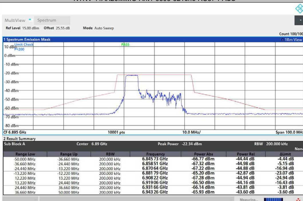
NTNV-11AX20MIMO-Ant2-6895-52Tone-RU37-PASS
