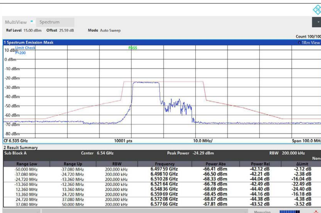
NTNV-11AX20MIMO-Ant1-6535-106Tone-RU53-PASS
