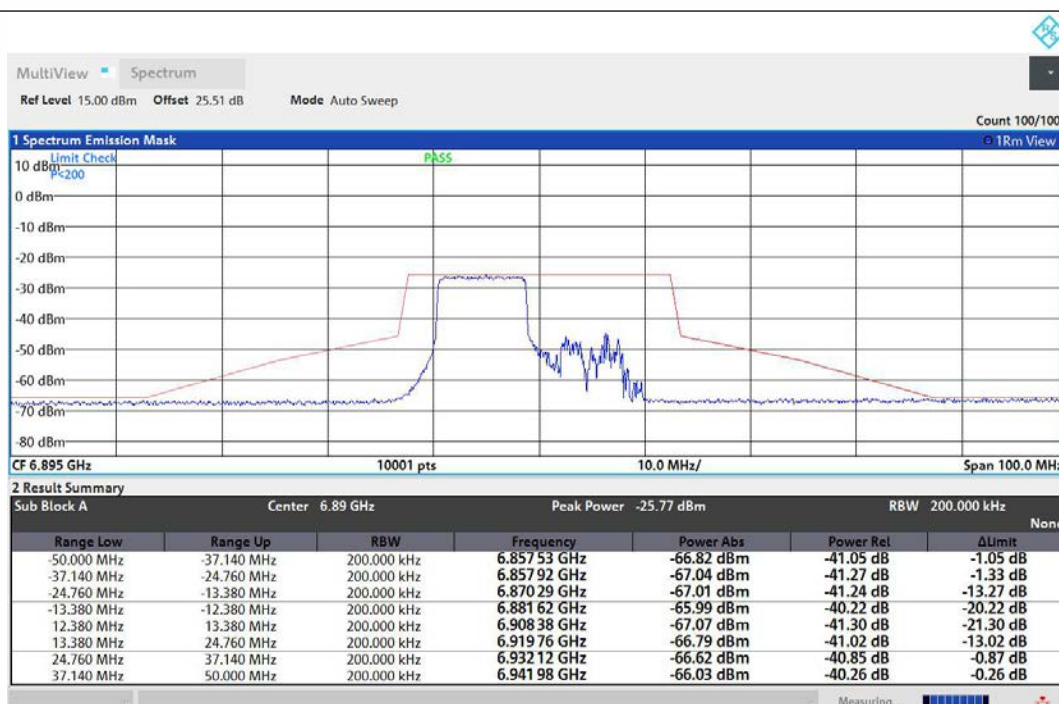
NTNV-11AX20MIMO-Ant1-6895-106Tone-RU53-PASS
