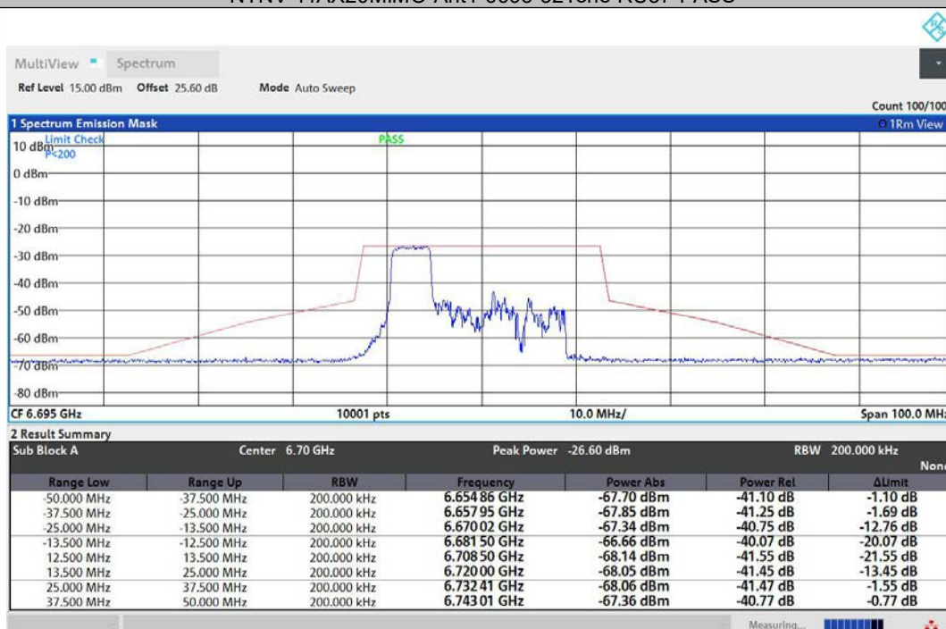
NTNV-11AX20MIMO-Ant2-6695-52Tone-RU37-PASS
