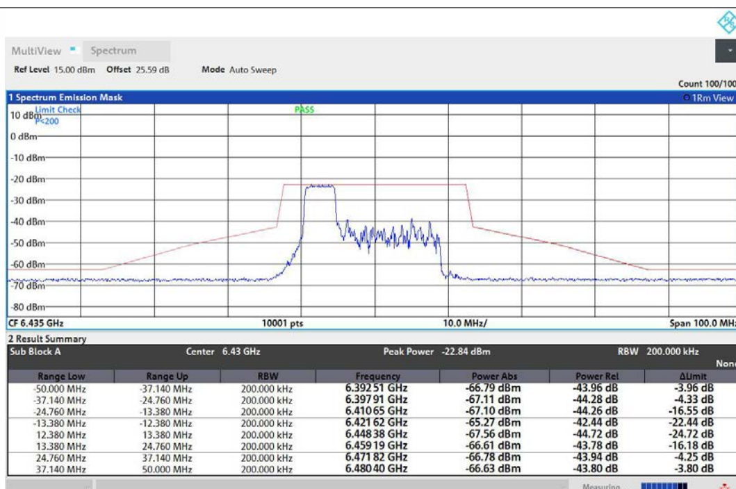
NTNV-11AX20MIMO-Ant1-6435-52Tone-RU37-PASS
