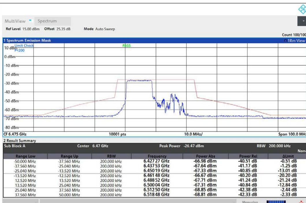
NTNV-11AX20MIMO-Ant1-6475-106Tone-RU53-PASS
