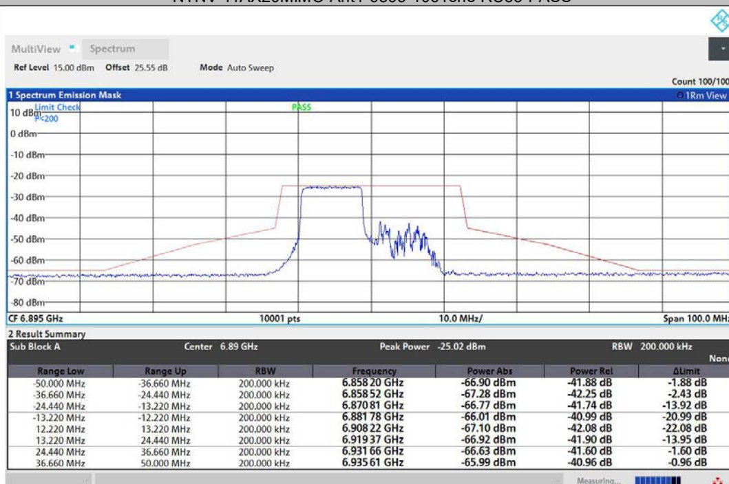
NTNV-11AX20MIMO-Ant2-6895-106Tone-RU53-PASS
