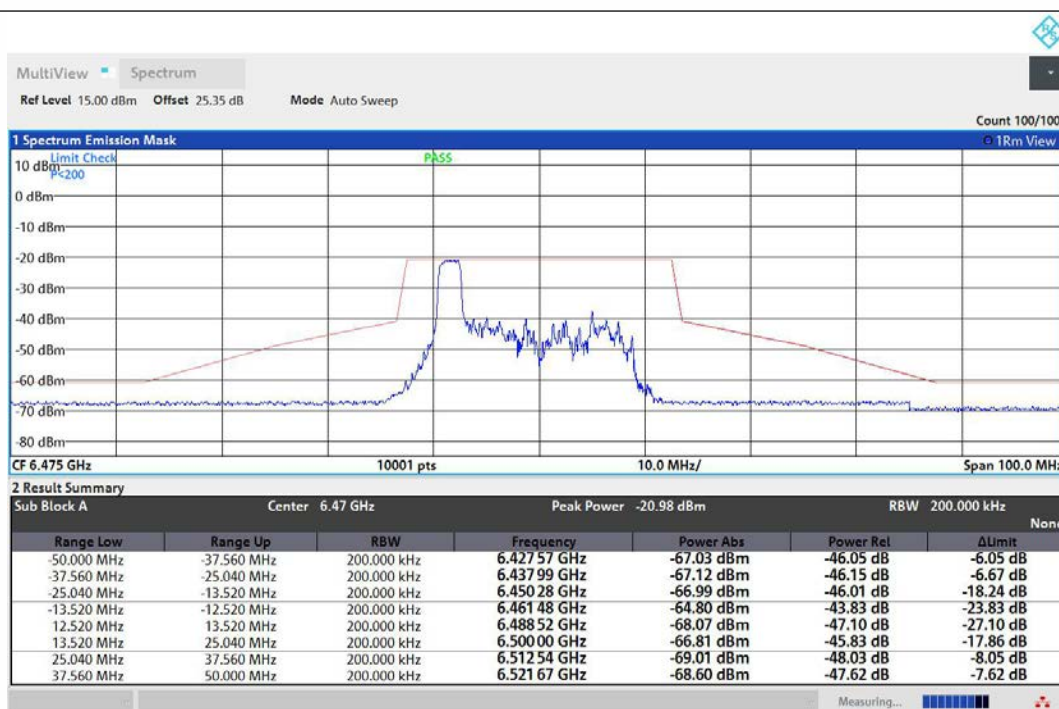
NTNV-11AX20MIMO-Ant1-6475-26Tone-RU0-PASS
