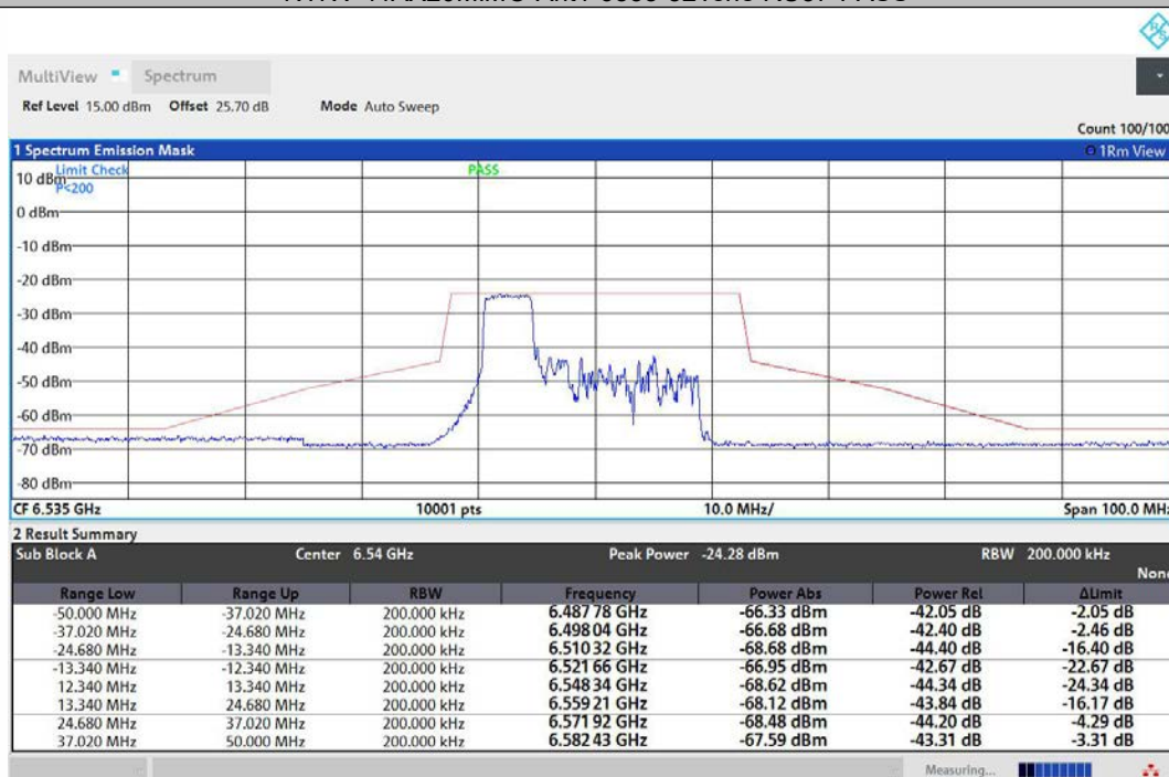
NTNV-11AX20MIMO-Ant2-6535-52Tone-RU37-PASS
