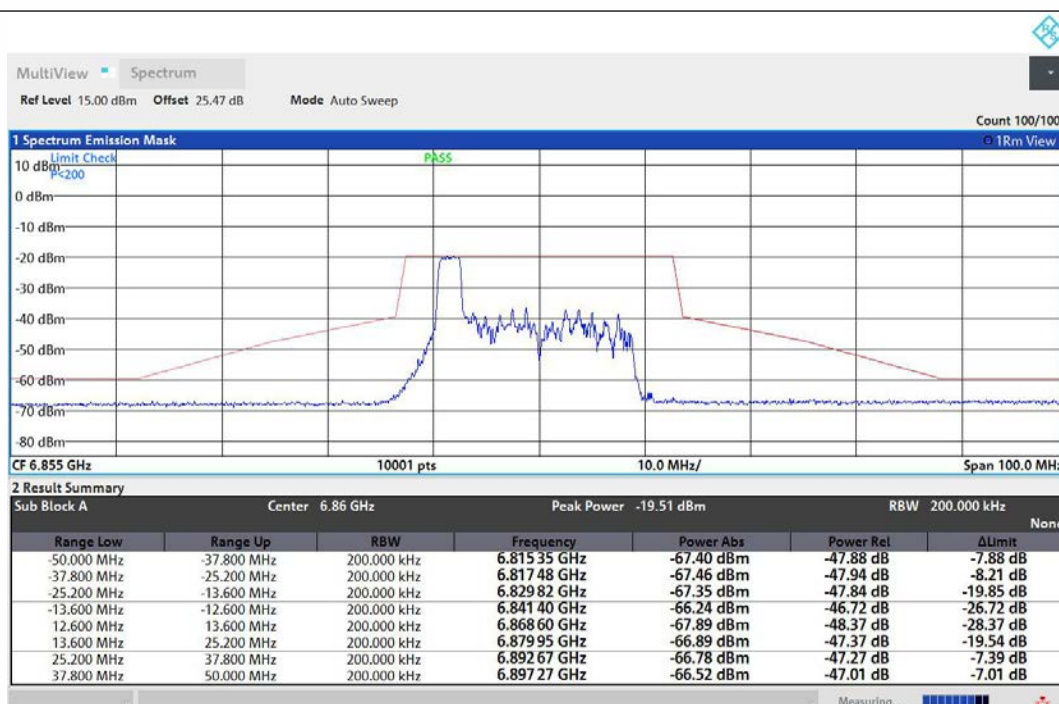
NTNV-11AX20MIMO-Ant1-6855-26Tone-RU0-PASS
