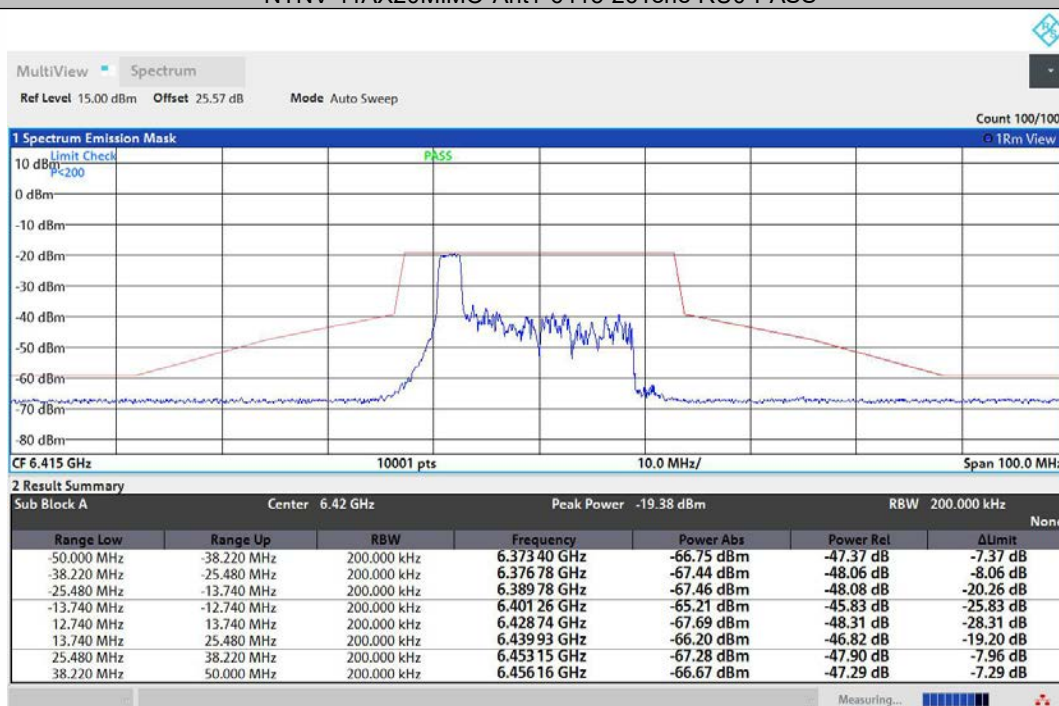
NTNV-11AX20MIMO-Ant2-6415-26Tone-RU0-PASS
