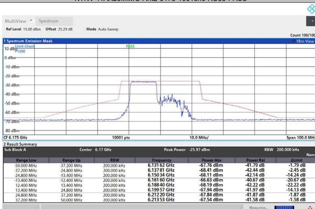
NTNV-11AX20MIMO-Ant1-6175-106Tone-RU53-PASS
