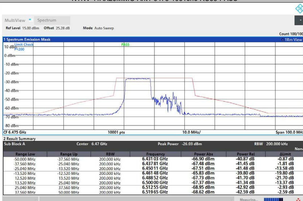
NTNV-11AX20MIMO-Ant2-6475-106Tone-RU53-PASS
