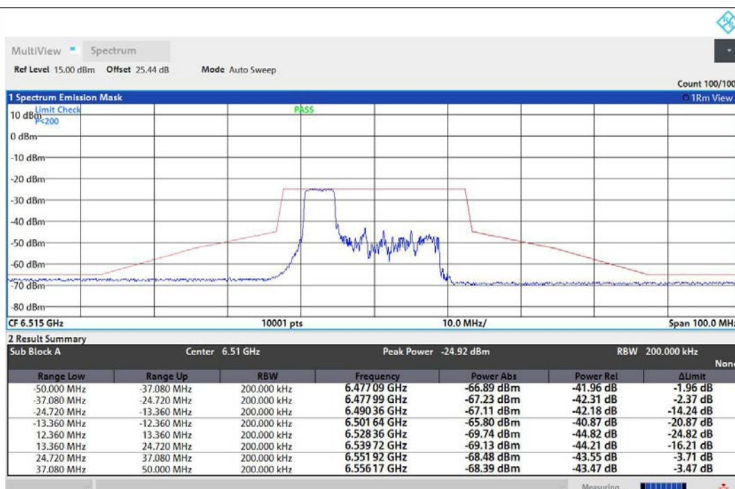
NTNV-11AX20MIMO-Ant1-6515-52Tone-RU37-PASS
