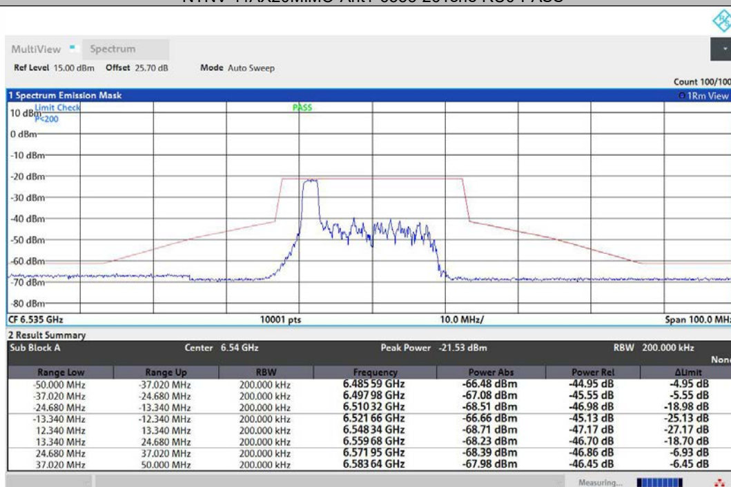
NTNV-11AX20MIMO-Ant2-6535-26Tone-RU0-PASS
