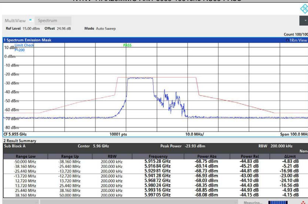
NTNV-11AX20MIMO-Ant2-5955-106Tone-RU53-PASS
