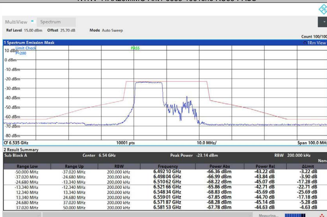
NTNV-11AX20MIMO-Ant2-6535-106Tone-RU53-PASS
