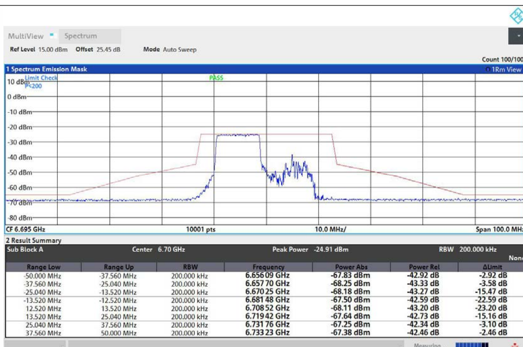
NTNV-11AX20MIMO-Ant1-6695-106Tone-RU53-PASS
