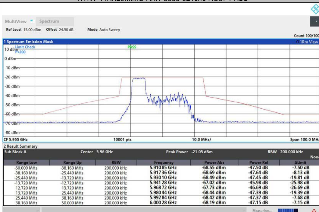
NTNV-11AX20MIMO-Ant2-5955-52Tone-RU37-PASS
