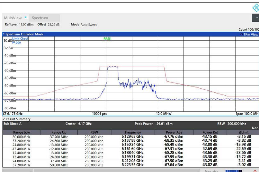
NTNV-11AX20MIMO-Ant1-6175-52Tone-RU37-PASS
