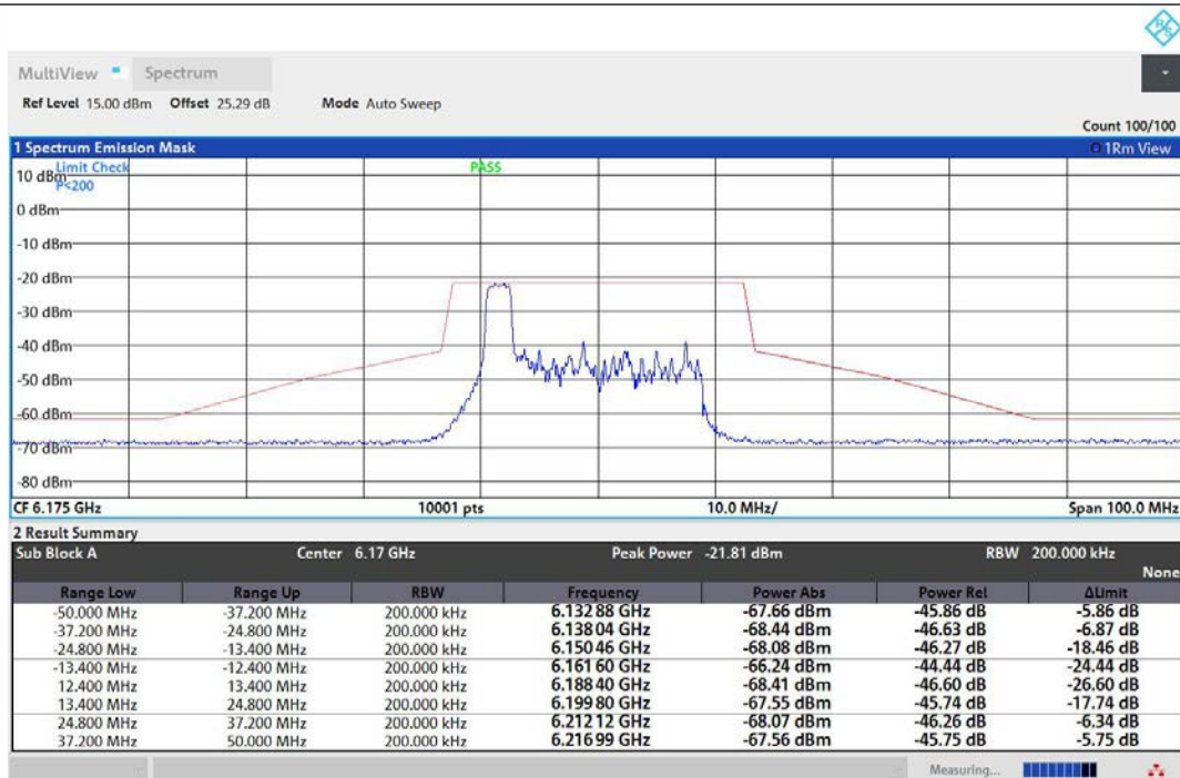
NTNV-11AX20MIMO-Ant1-6175-26Tone-RU0-PASS
