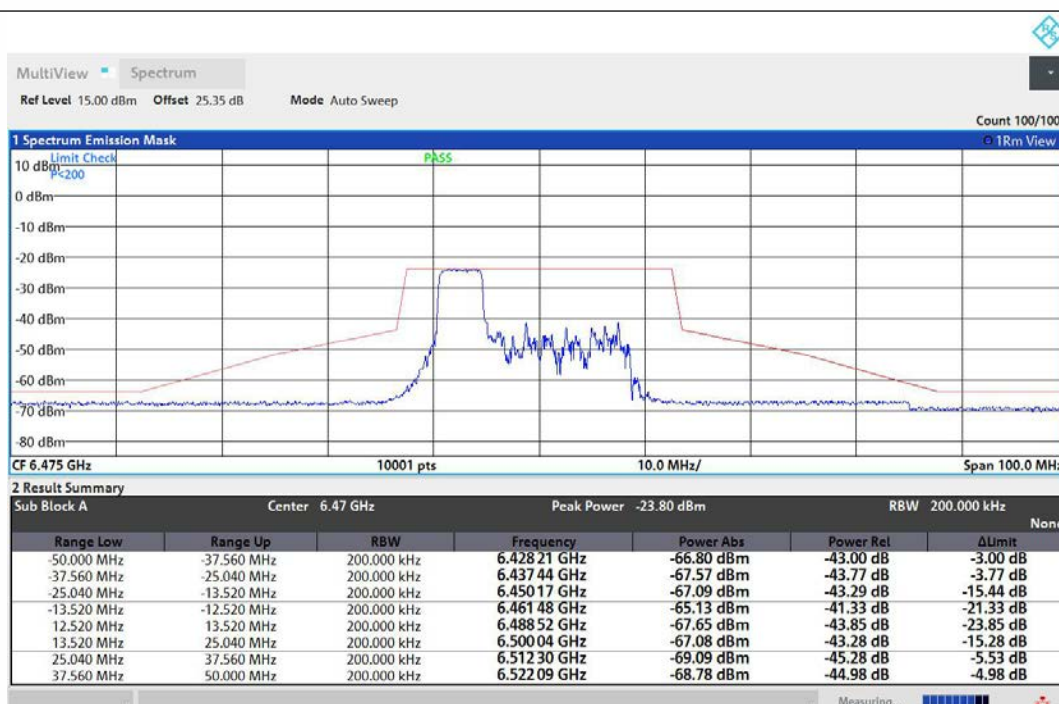
NTNV-11AX20MIMO-Ant1-6475-52Tone-RU37-PASS
