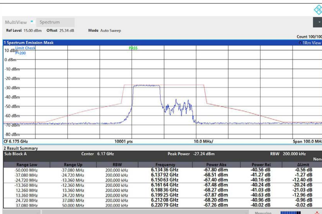
NTNV-11AX20MIMO-Ant2-6175-106Tone-RU53-PASS
