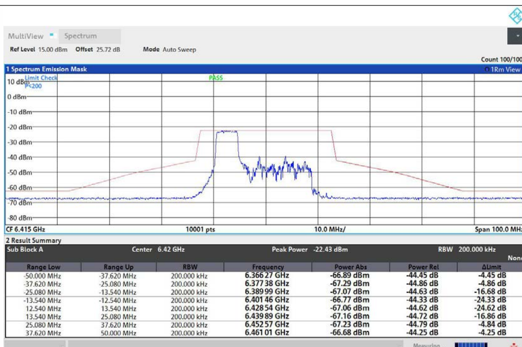
NTNV-11AX20MIMO-Ant1-6415-52Tone-RU37-PASS
