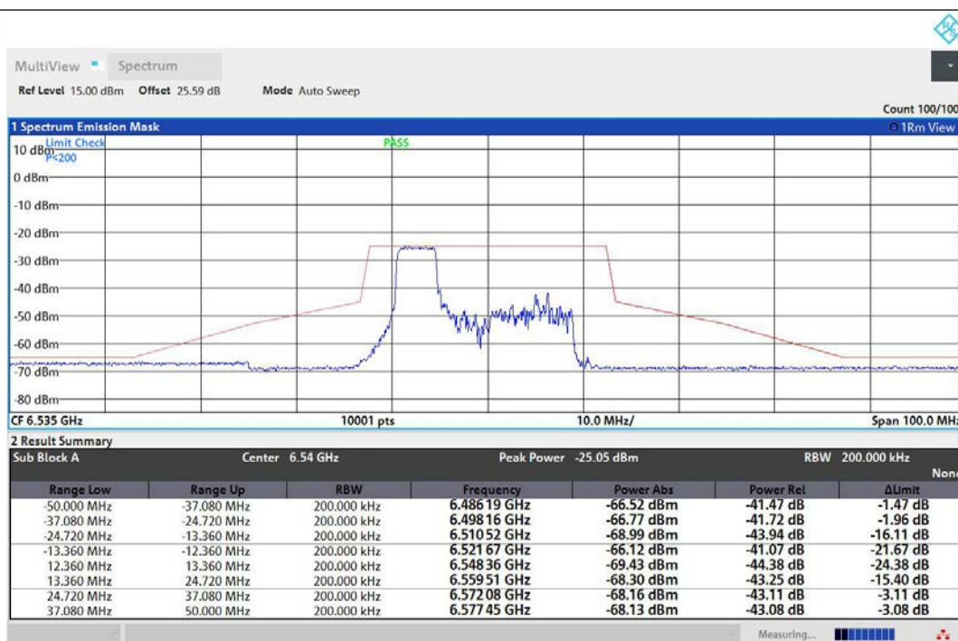
NTNV-11AX20MIMO-Ant1-6535-52Tone-RU37-PASS
