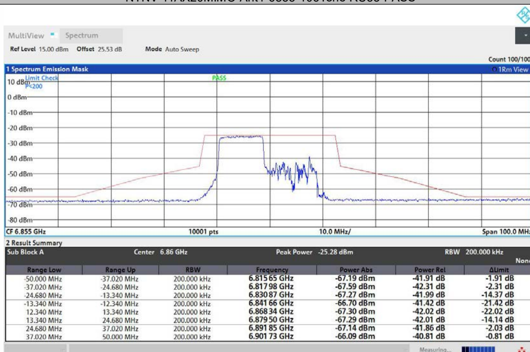
NTNV-11AX20MIMO-Ant2-6855-106Tone-RU53-PASS
