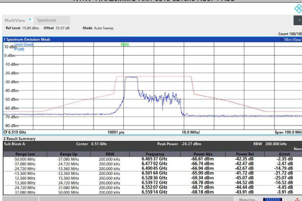
NTNV-11AX20MIMO-Ant2-6515-52Tone-RU37-PASS
