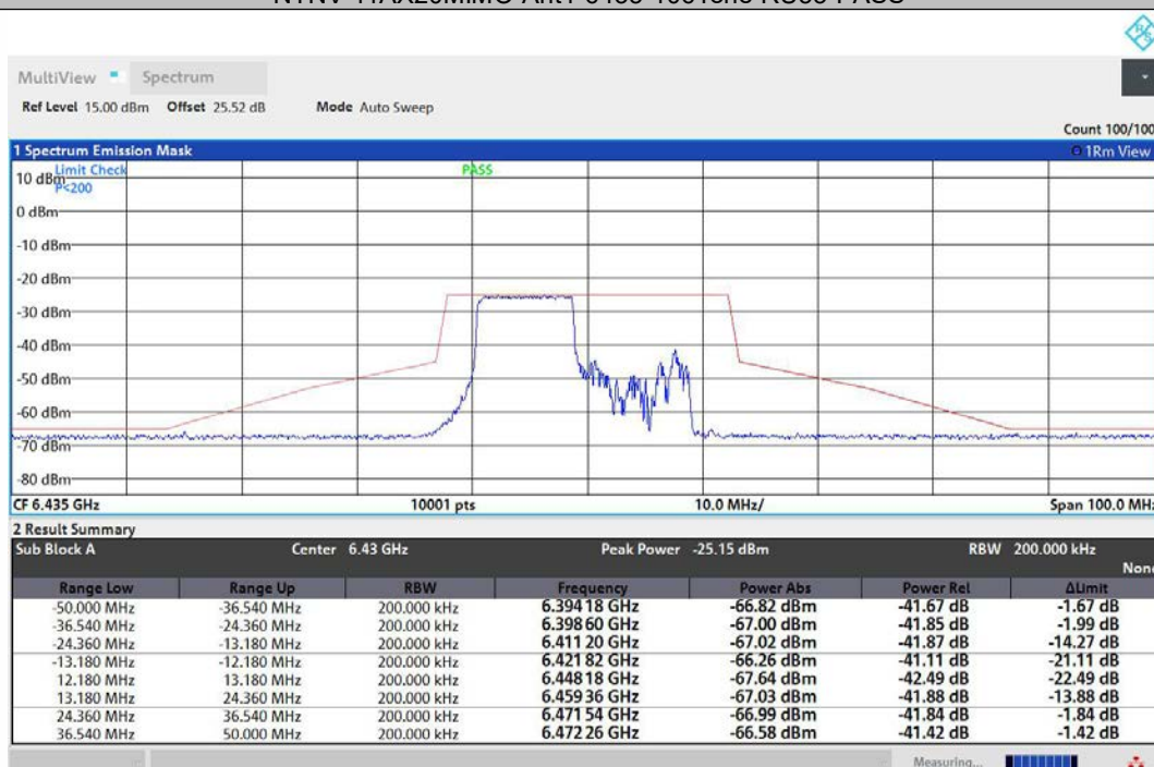
NTNV-11AX20MIMO-Ant2-6435-106Tone-RU53-PASS
