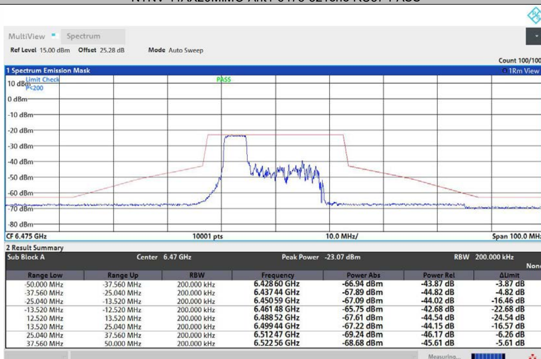
NTNV-11AX20MIMO-Ant2-6475-52Tone-RU37-PASS
