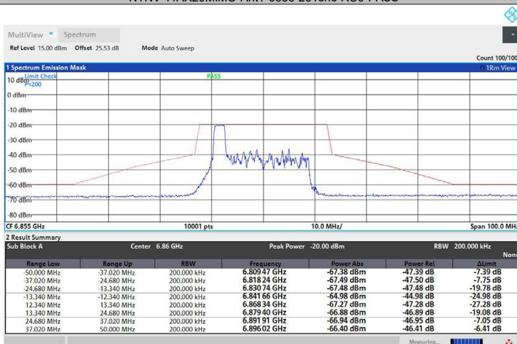
NTNV-11AX20MIMO-Ant2-6855-26Tone-RU0-PASS
