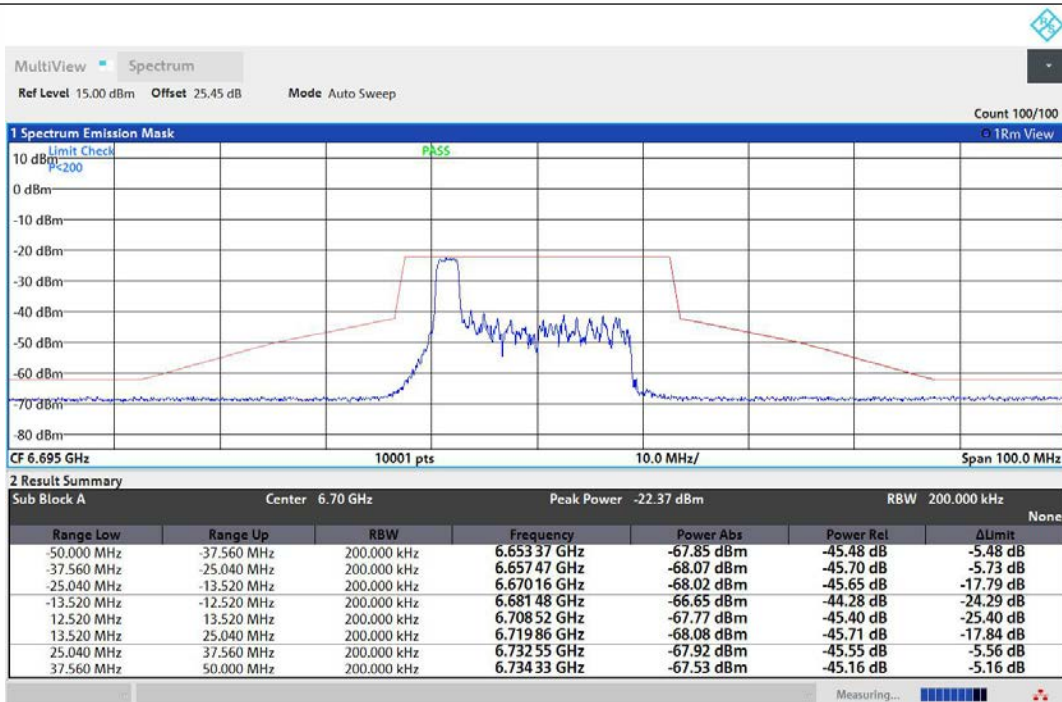
NTNV-11AX20MIMO-Ant1-6695-26Tone-RU0-PASS
