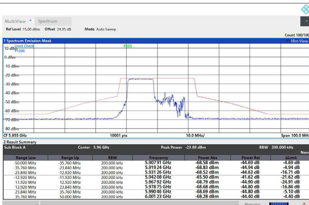
NTNV-11AX20MIMO-Ant1-5955-106Tone-RU53-PASS
