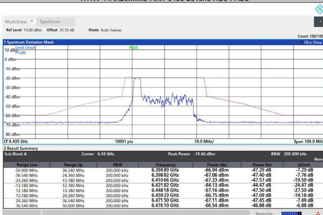
NTNV-11AX20MIMO-Ant2-6435-26Tone-RU0-PASS
