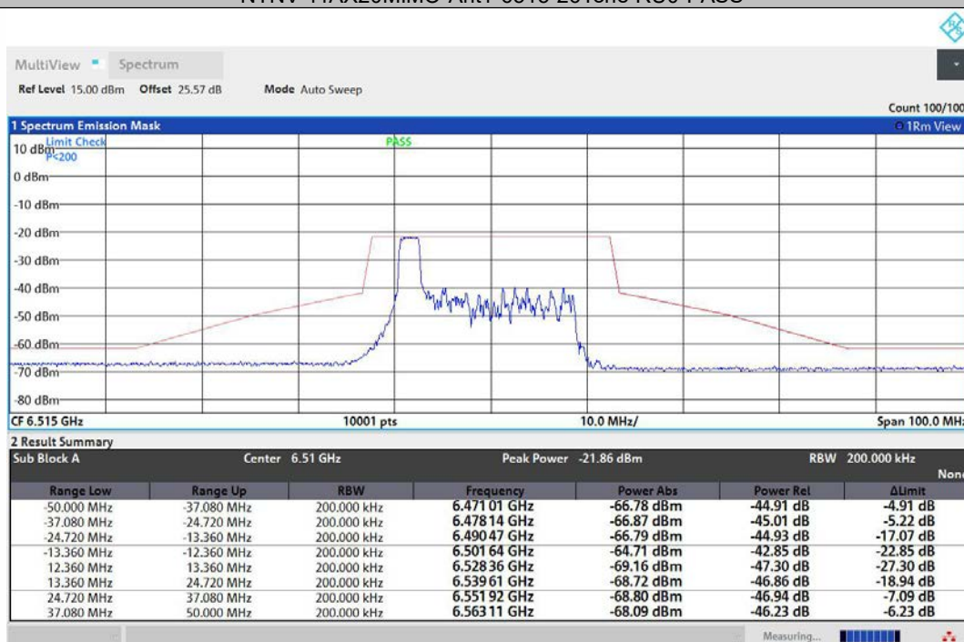
NTNV-11AX20MIMO-Ant2-6515-26Tone-RU0-PASS
