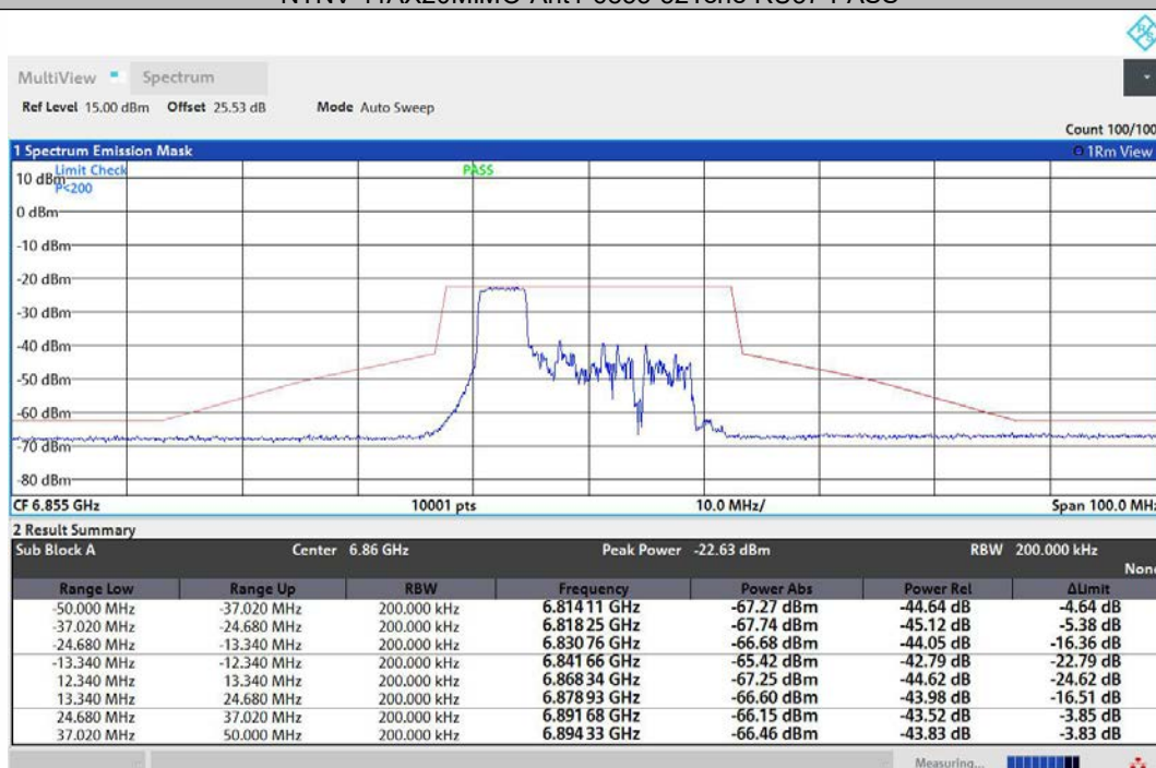
NTNV-11AX20MIMO-Ant2-6855-52Tone-RU37-PASS
