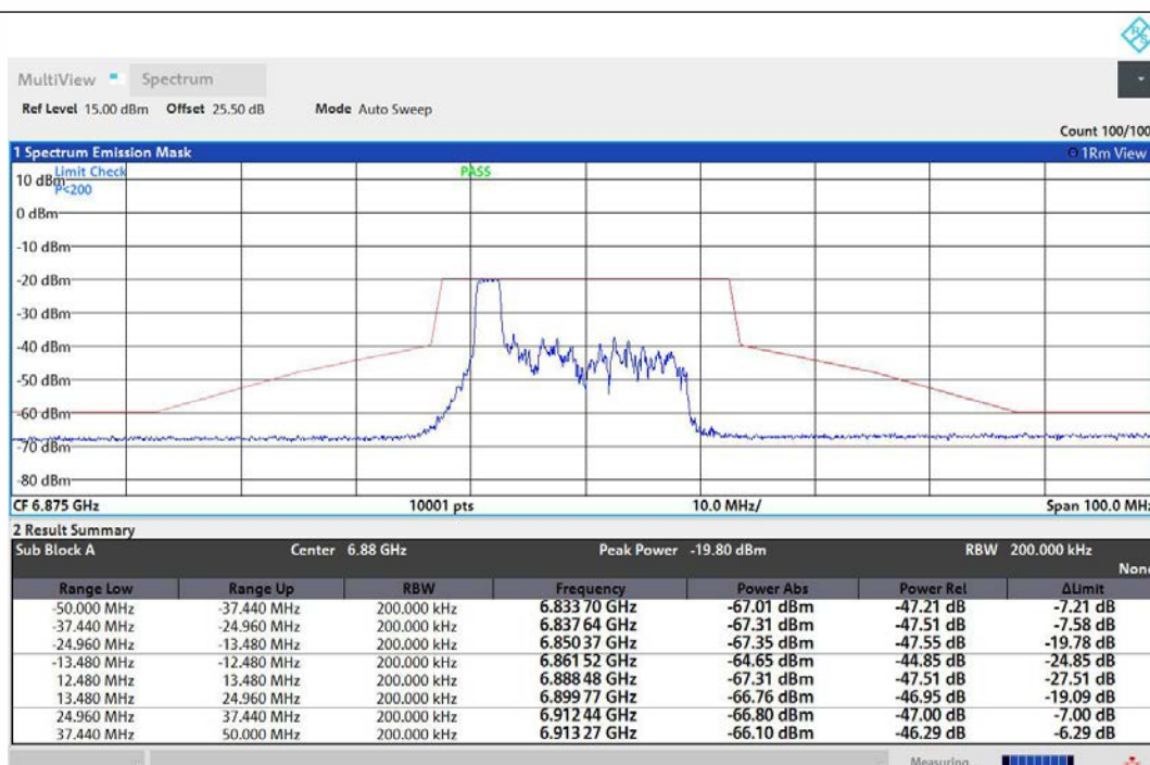
NTNV-11AX20MIMO-Ant1-6875-26Tone-RU0-PASS
