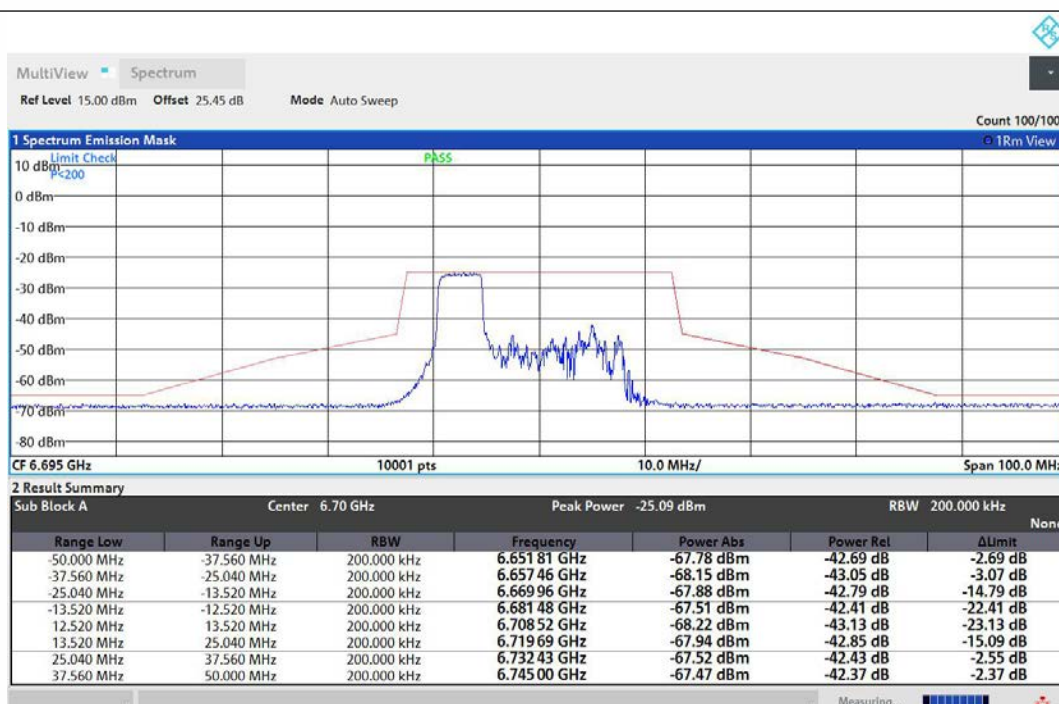
NTNV-11AX20MIMO-Ant1-6695-52Tone-RU37-PASS
