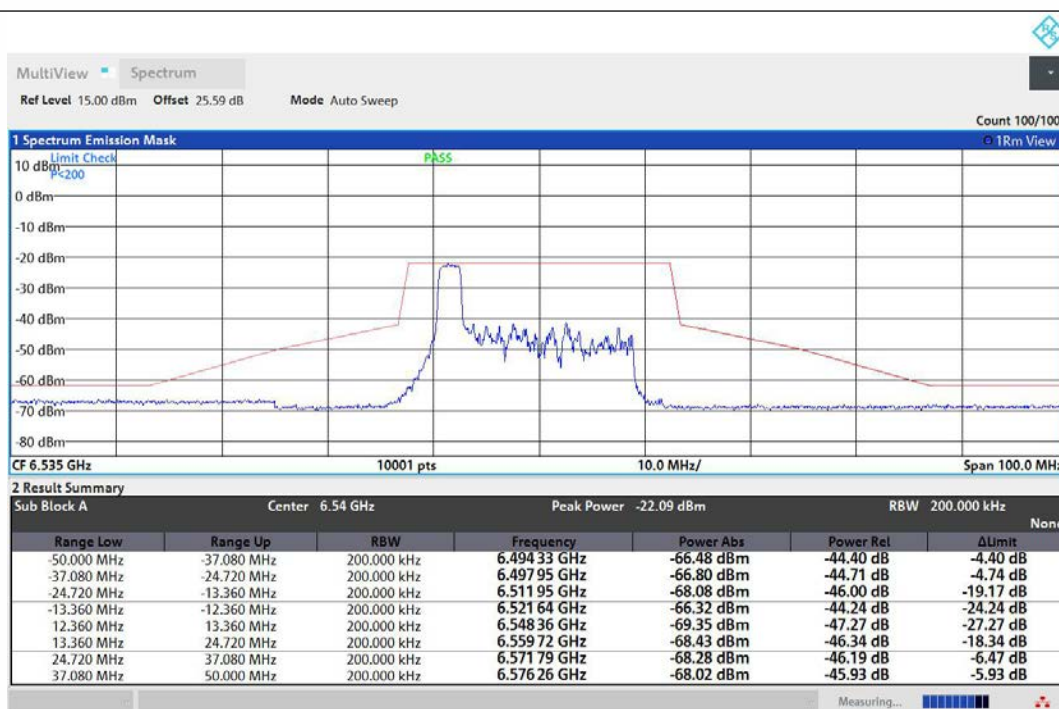
NTNV-11AX20MIMO-Ant1-6535-26Tone-RU0-PASS
