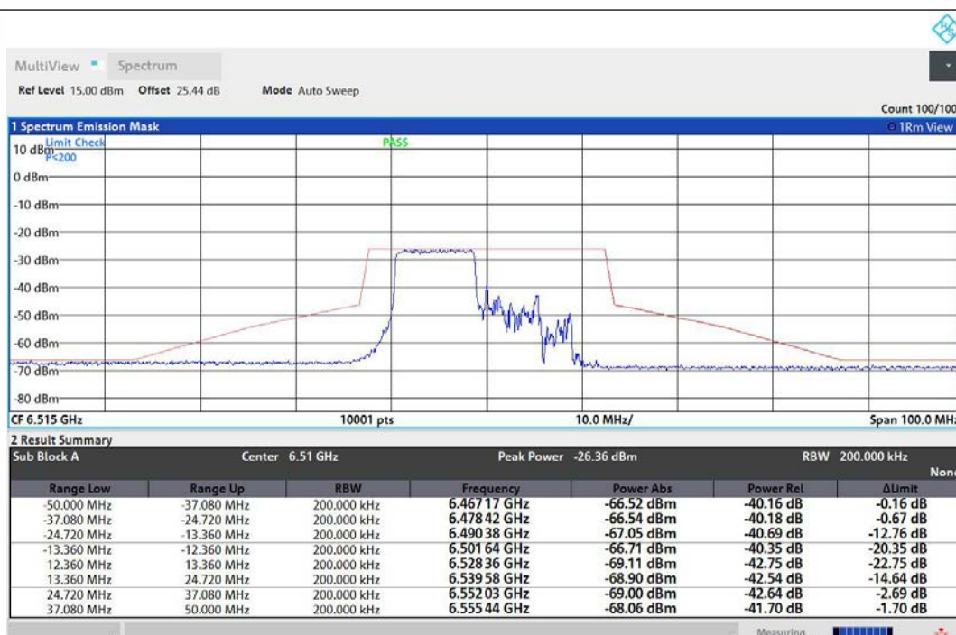
NTNV-11AX20MIMO-Ant1-6515-106Tone-RU53-PASS
