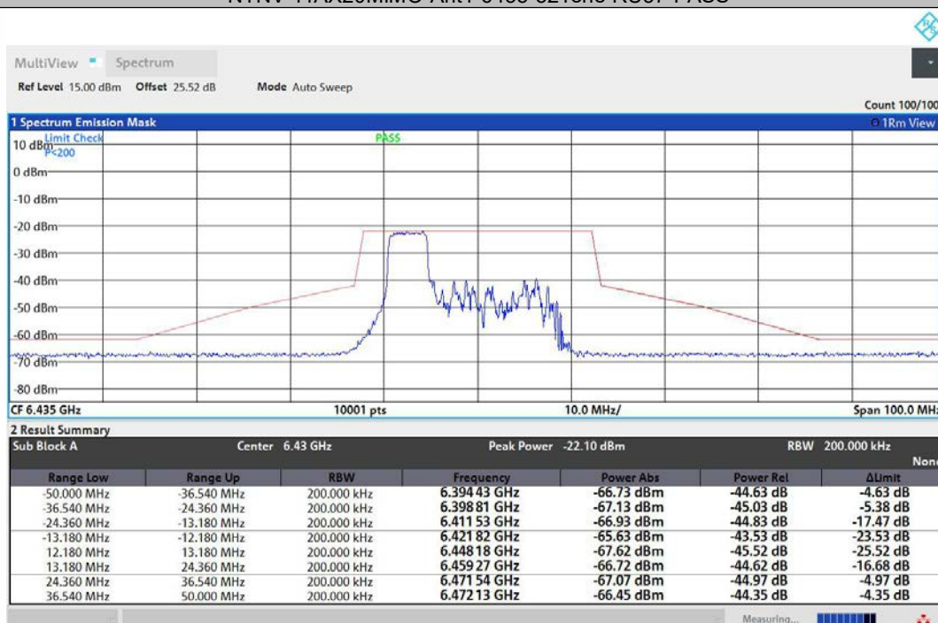
NTNV-11AX20MIMO-Ant2-6435-52Tone-RU37-PASS
