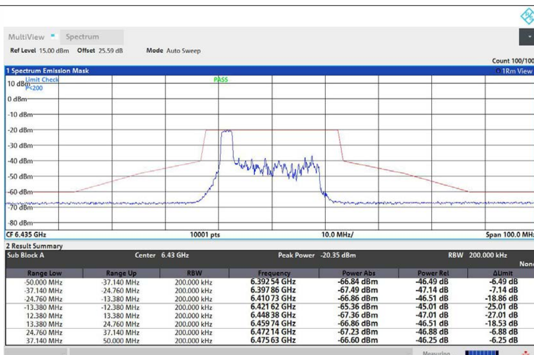
NTNV-11AX20MIMO-Ant1-6435-26Tone-RU0-PASS
