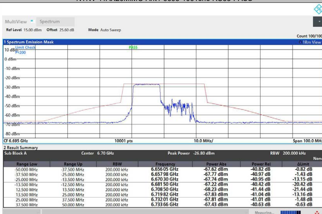
NTNV-11AX20MIMO-Ant2-6695-106Tone-RU53-PASS
