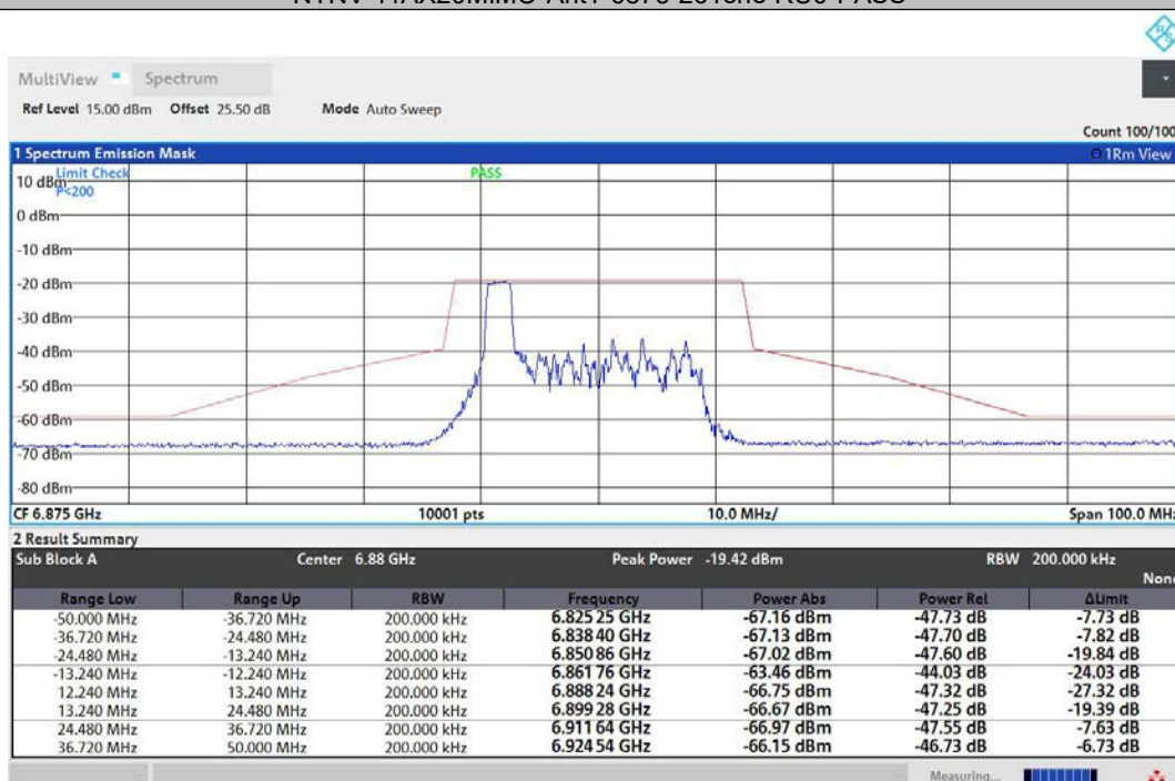
NTNV-11AX20MIMO-Ant2-6875-26Tone-RU0-PASS
