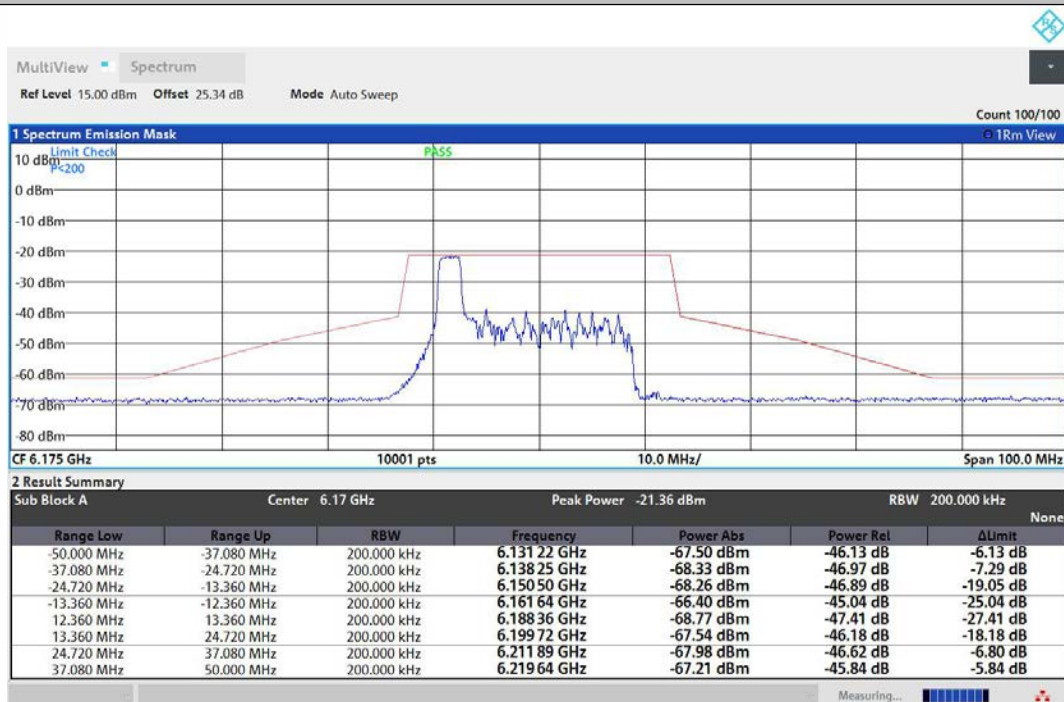
NTNV-11AX20MIMO-Ant2-6175-26Tone-RU0-PASS
