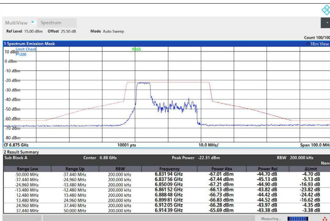
NTNV-11AX20MIMO-Ant1-6875-52Tone-RU37-PASS
