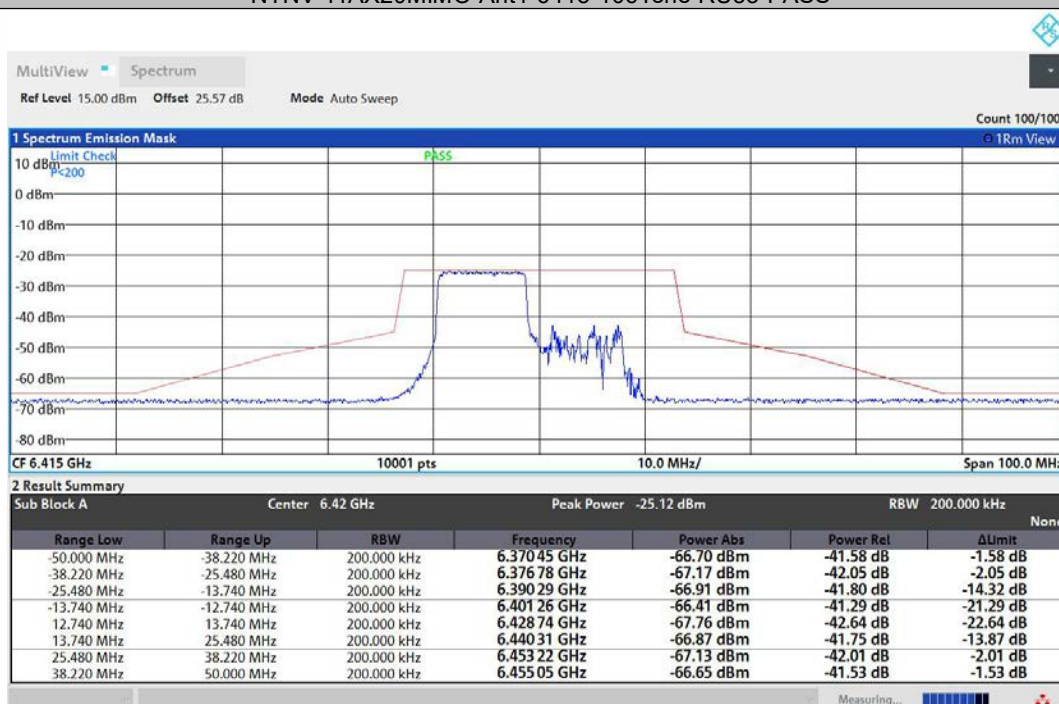
NTNV-11AX20MIMO-Ant2-6415-106Tone-RU53-PASS
