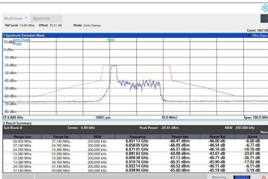
NTNV-11AX20MIMO-Ant1-6895-26Tone-RU0-PASS
