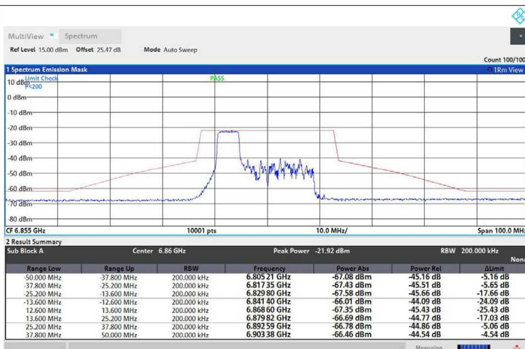
NTNV-11AX20MIMO-Ant1-6855-52Tone-RU37-PASS
