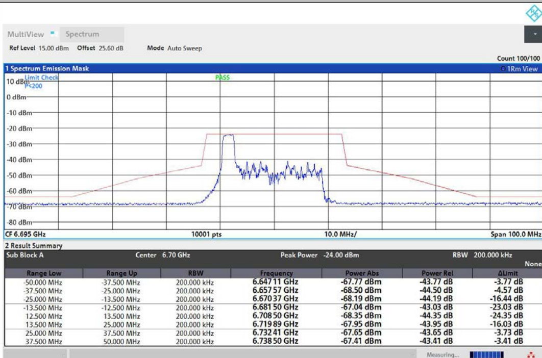
NTNV-11AX20MIMO-Ant2-6695-26Tone-RU0-PASS
