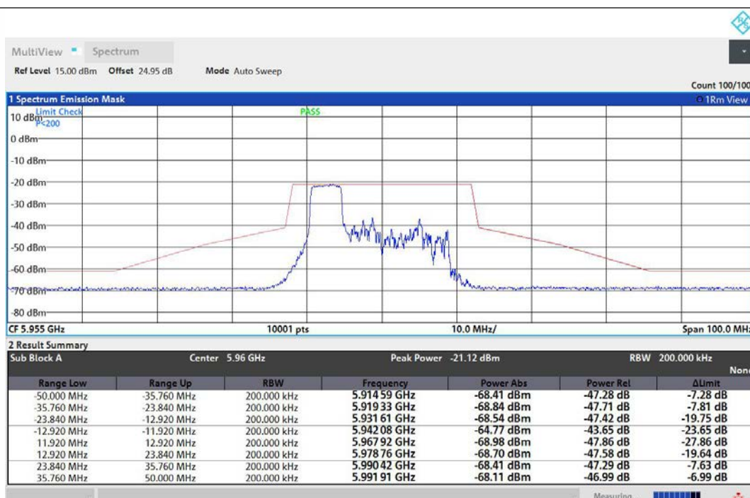
NTNV-11AX20MIMO-Ant1-5955-52Tone-RU37-PASS
