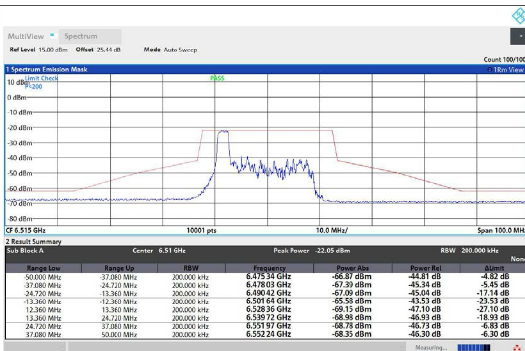
NTNV-11AX20MIMO-Ant1-6515-26Tone-RU0-PASS
