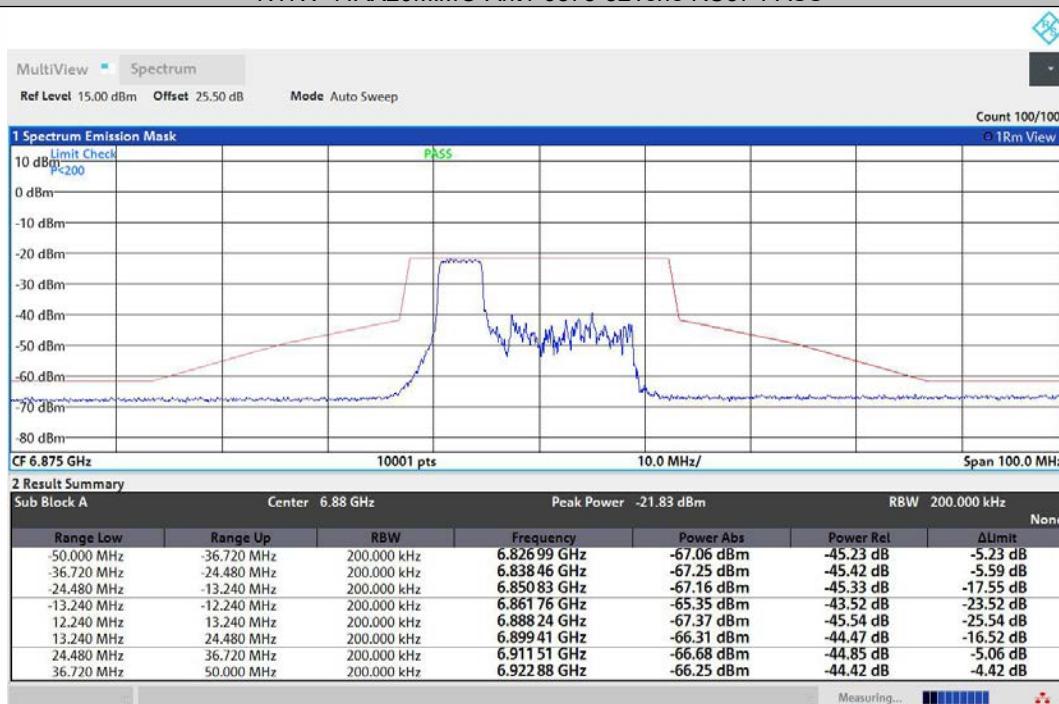
NTNV-11AX20MIMO-Ant2-6875-52Tone-RU37-PASS
