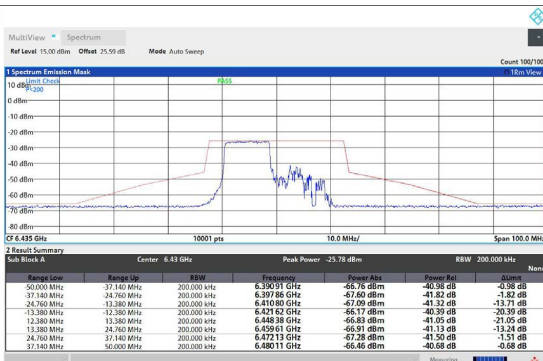
NTNV-11AX20MIMO-Ant1-6435-106Tone-RU53-PASS
