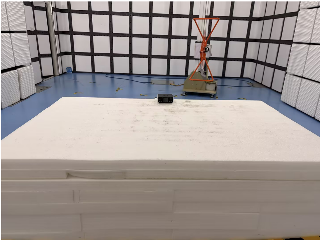
Radiation Emission - Front View (Below 1GHz)
