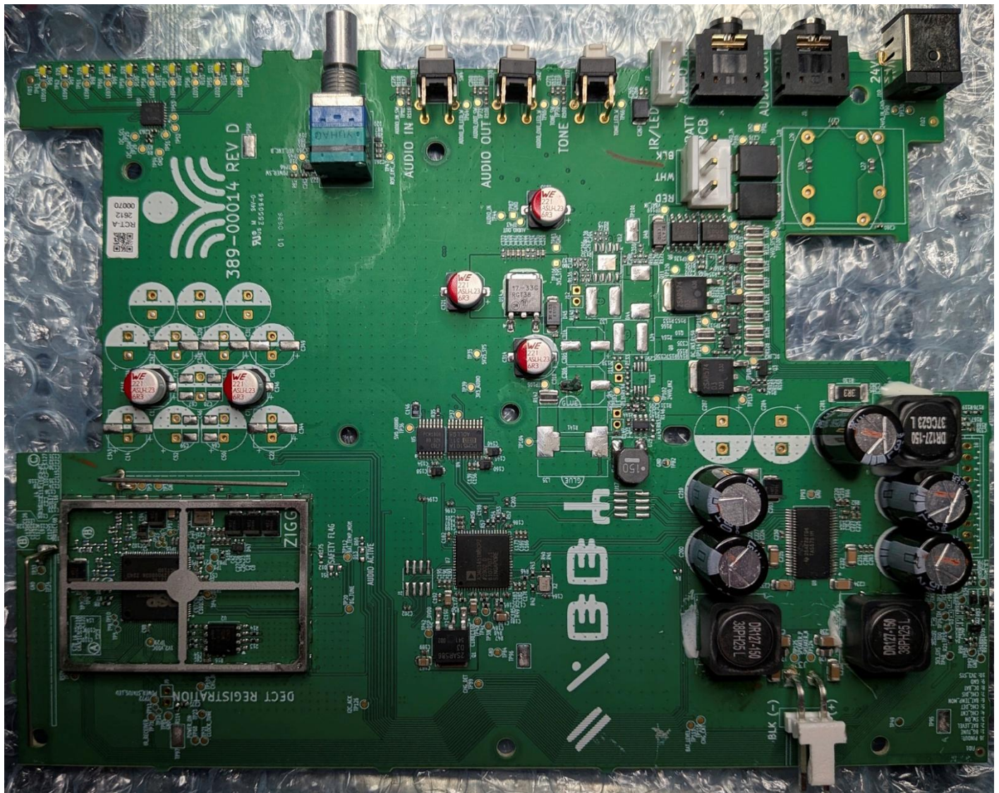
Metal shield removed to show DECT Radio
