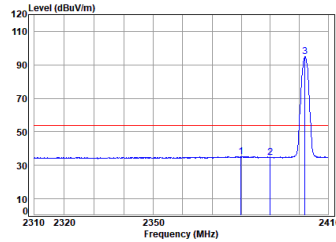
Dongle 2.4G SRD_1M_TX_CH_00_Vertical-Avg
