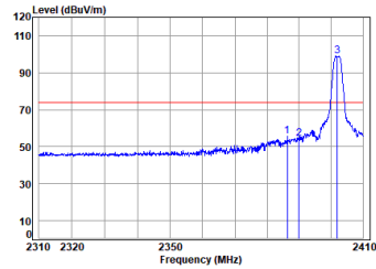
Dongle 2.4G SRD_2M_TX_CH_00_Horizontal-Peak
