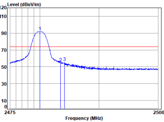
Dongle 2.4G SRD_1M_TX_CH_39_Vertical-Peak
