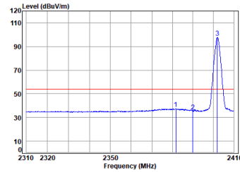
Dongle 2.4G SRD_2M_TX_CH_00_Horizontal-Avg
