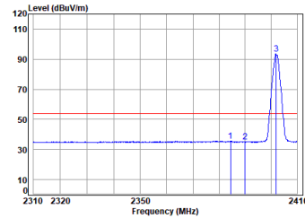
Dongle 2.4G SRD_2M_TX_CH_00_Vertical-Avg
