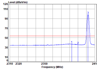
Dongle 2.4G SRD_1M_TX_CH_00_Horizontal-Avg
