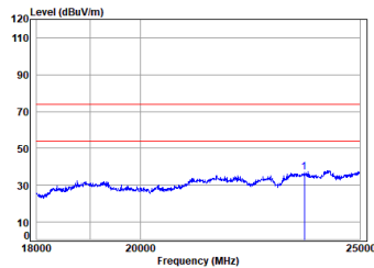
Dongle 2.4G SRD_1M_TX_CH_19_Horizontal-Peak
