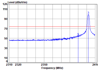
Dongle 2.4G SRD_1M_TX_CH_00_Horizontal-Peak
