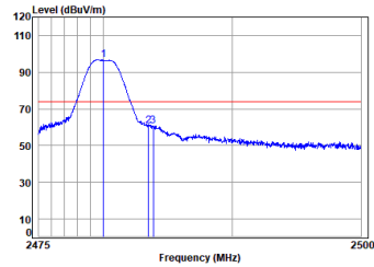
Dongle 2.4G SRD_2M_TX_CH_39_Horizontal-Peak
