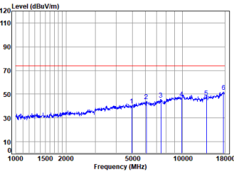
Dongle 2.4G SRD_2M_TX_CH_39_Vertical-Peak
