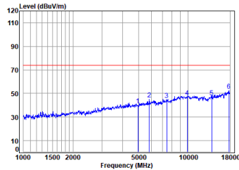
Dongle 2.4G SRD_2M_TX_CH_39_Horizontal-Peak
