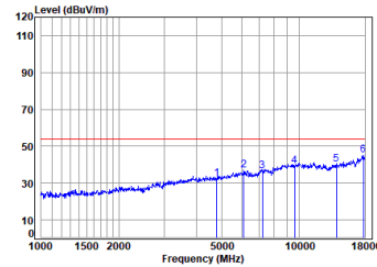
Dongle 2.4G SRD_2M_TX_CH_00_Vertical-Avg
