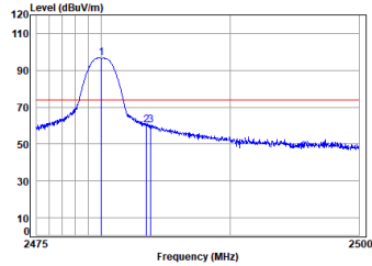
Dongle 2.4G SRD_1M_TX_CH_39_Horizontal-Peak
