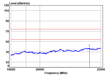
Dongle 2.4G SRD_1M_TX_CH_19_Vertical-Peak
