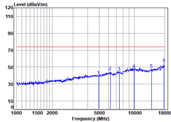
Dongle 2.4G SRD_1M_TX_CH_39_Horizontal-Peak
