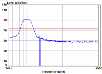
Dongle 2.4G SRD_2M_TX_CH_39_Vertical-Peak
