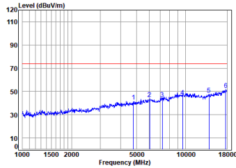
Dongle 2.4G SRD_1M_TX_CH_00_Vertical-Peak
