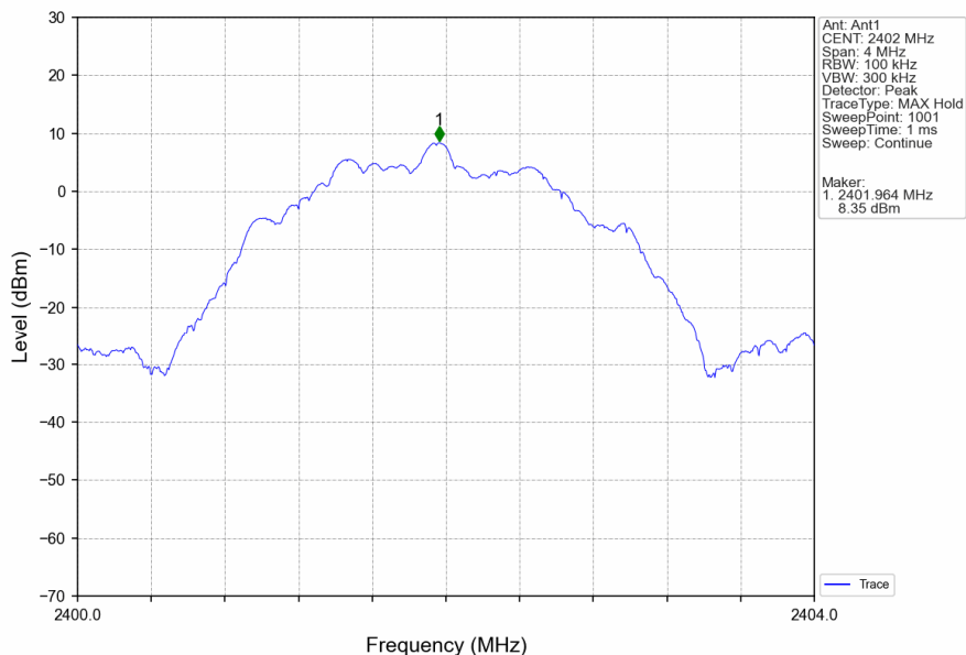
2.4G-2M_LCH_2402MHz_Ant1_NTNV
