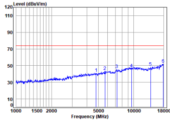
Dongle 2.4G SRD_1M_TX_CH_00_Horizontal-Peak
