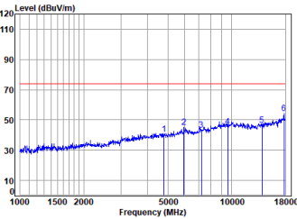
Dongle 2.4G SRD_2M_TX_CH_00_Vertical-Peak
