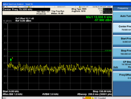
Band4-10MHz-16QAM-20350-1#5-0.009-0.15-PASS
