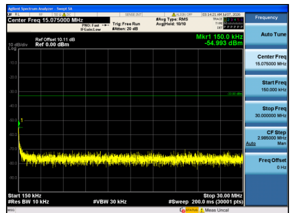
Band4-15MHz-16QAM-20325-1#5-0.15-30-PASS
