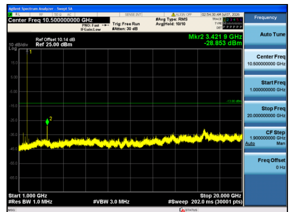
Band4-10MHz-QPSK-20000-1#0-1000-20000-PASS
