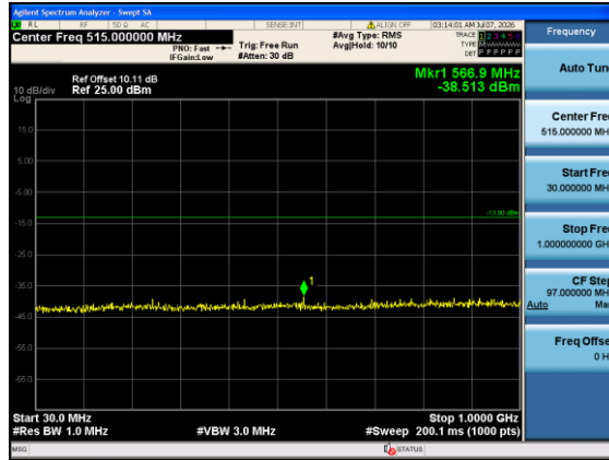
Band4-15MHz-QPSK-20325-1#5-30-1000-PASS
