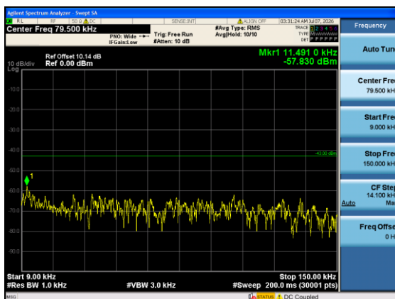
Band4-20MHz-16QAM-20050-1#0-0.009-0.15-PASS
