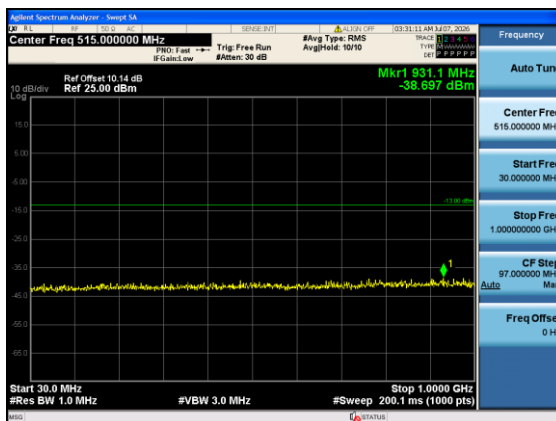
Band4-20MHz-QPSK-20050-1#0-30-1000-PASS
