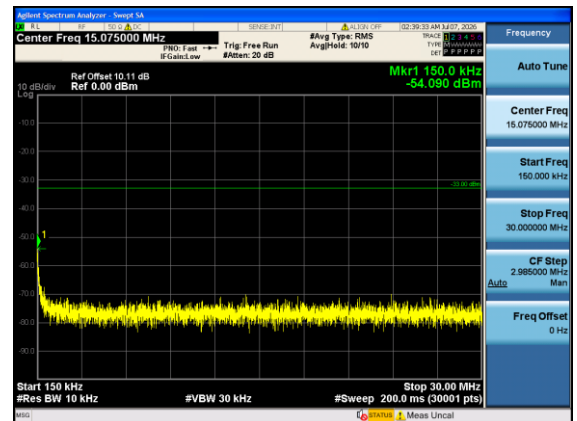
Band4-5MHz-16QAM-20375-1#5-0.15-30-PASS
