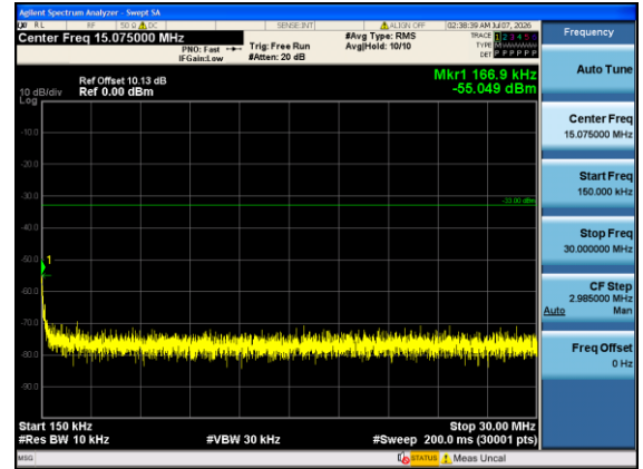
Band4-5MHz-16QAM-20175-1#0-0.15-30-PASS
