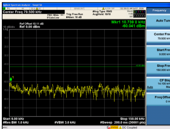
Band4-5MHz-QPSK-20375-1#5-0.009-0.15-PASS
