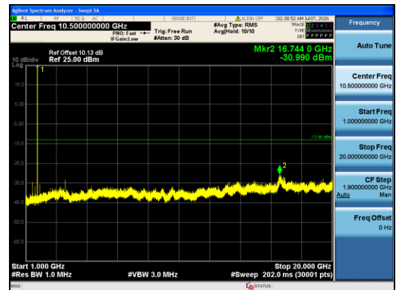
Band4-5MHz-16QAM-20175-1#0-1000-20000-PASS
