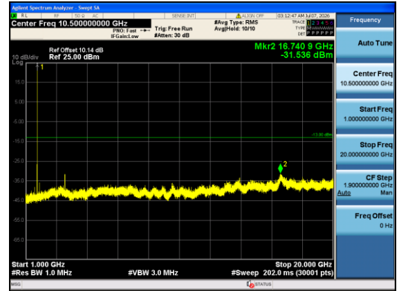
Band4-15MHz-16QAM-20025-1#0-1000-20000-PASS
