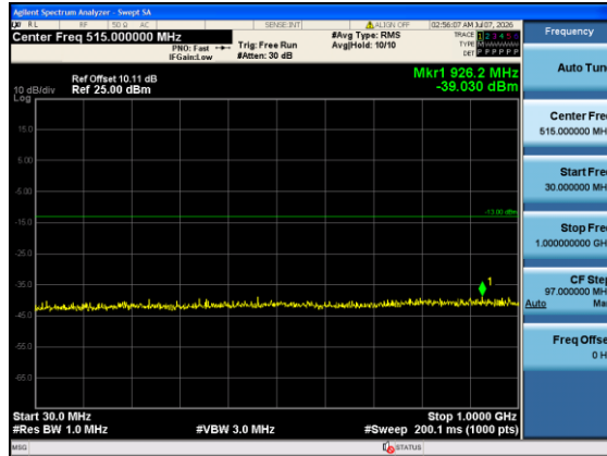
Band4-10MHz-QPSK-20350-1#5-30-1000-PASS
