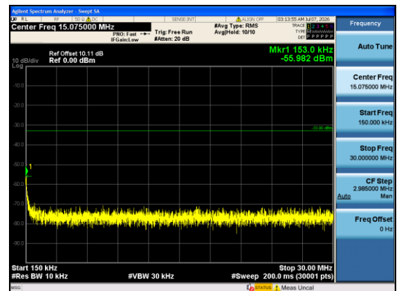
Band4-15MHz-QPSK-20325-1#5-0.15-30-PASS
