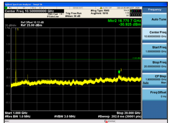
Band4-15MHz-16QAM-20175-1#0-1000-20000-PASS
