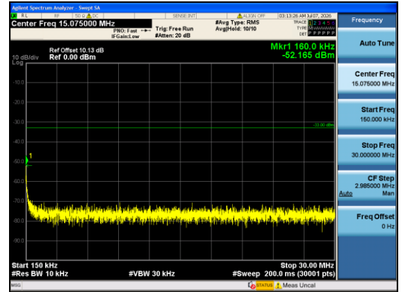
Band4-15MHz-16QAM-20175-1#0-0.15-30-PASS
