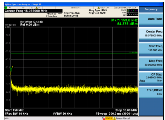
Band4-15MHz-QPSK-20175-1#0-0.15-30-PASS
