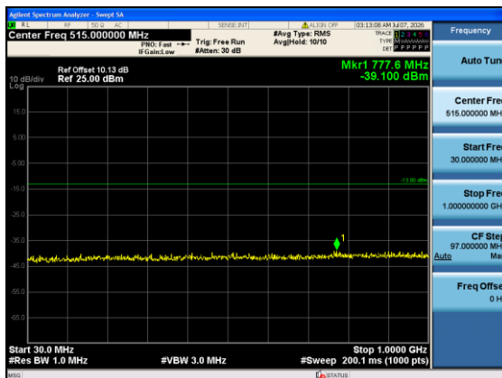
Band4-15MHz-QPSK-20175-1#0-30-1000-PASS
