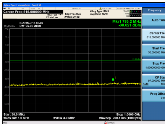
Band4-10MHz-16QAM-20175-1#0-30-1000-PASS
