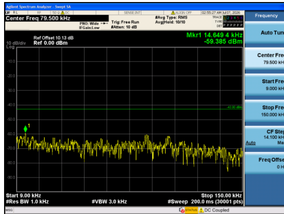
Band4-10MHz-16QAM-20175-1#0-0.009-0.15-PASS
