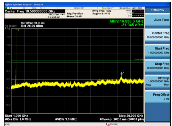
Band4-15MHz-QPSK-20025-1#0-1000-20000-PASS
