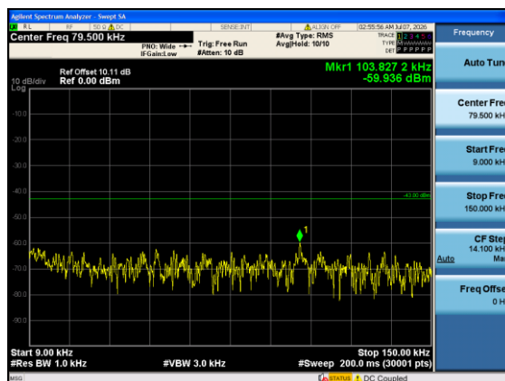
Band4-10MHz-QPSK-20350-1#5-0.009-0.15-PASS
