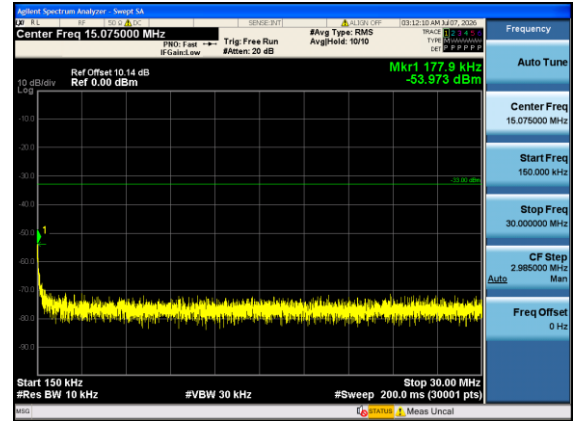
Band4-15MHz-QPSK-20025-1#0-0.15-30-PASS
