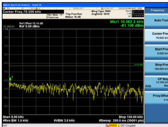
Band4-15MHz-16QAM-20025-1#0-0.009-0.15-PASS
