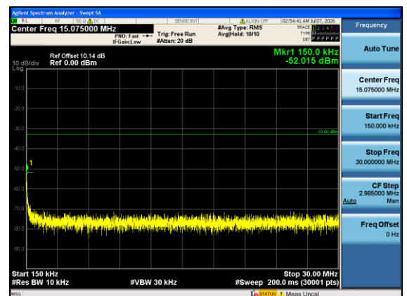
Band4-10MHz-16QAM-20000-1#0-0.15-30-PASS
