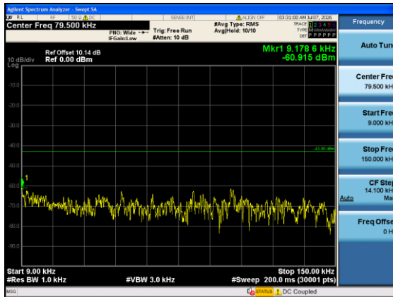
Band4-20MHz-QPSK-20050-1#0-0.009-0.15-PASS
