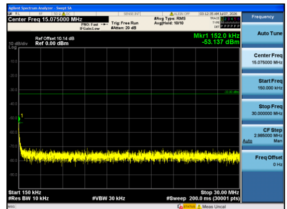
Band4-15MHz-16QAM-20025-1#0-0.15-30-PASS
