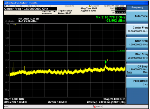
Band4-10MHz-16QAM-20000-1#0-1000-20000-PASS
