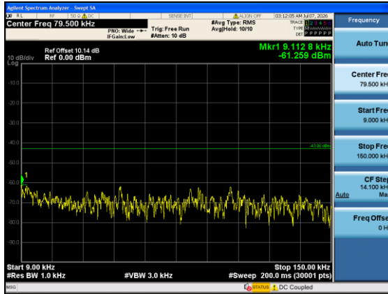
Band4-15MHz-QPSK-20025-1#0-0.009-0.15-PASS
