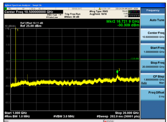
Band4-15MHz-16QAM-20325-1#5-1000-20000-PASS
