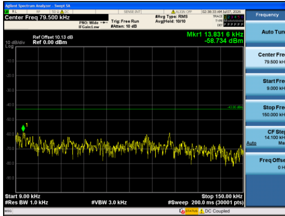
Band4-5MHz-16QAM-20175-1#0-0.009-0.15-PASS
