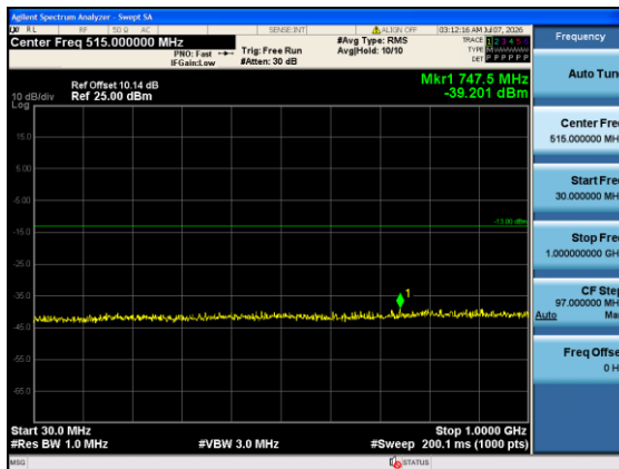
Band4-15MHz-QPSK-20025-1#0-30-1000-PASS
