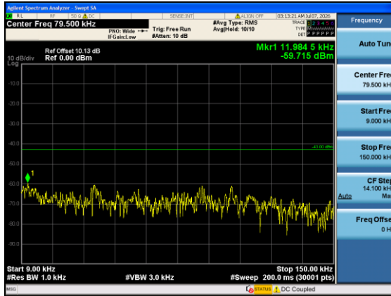
Band4-15MHz-16QAM-20175-1#0-0.009-0.15-PASS
