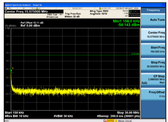
Band4-10MHz-16QAM-20350-1#5-0.15-30-PASS
