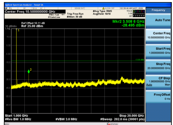
Band4-5MHz-16QAM-20375-1#5-1000-20000-PASS
