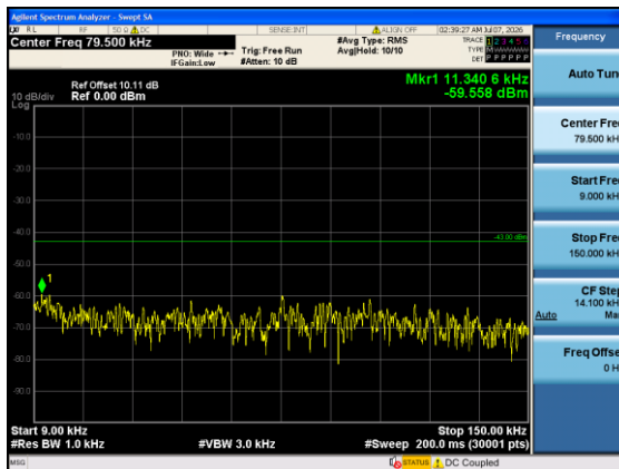
Band4-5MHz-16QAM-20375-1#5-0.009-0.15-PASS
