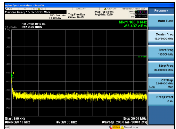
Band4-10MHz-QPSK-20175-1#0-0.15-30-PASS
