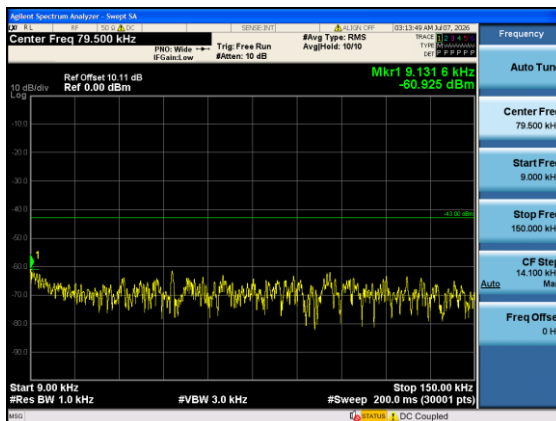
Band4-15MHz-QPSK-20325-1#5-0.009-0.15-PASS
