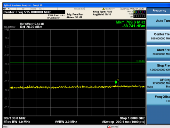
Band4-10MHz-QPSK-20000-1#0-30-1000-PASS
