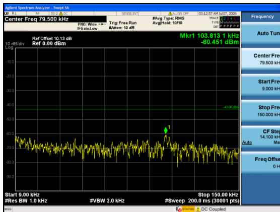
Band4-15MHz-QPSK-20175-1#0-0.009-0.15-PASS
