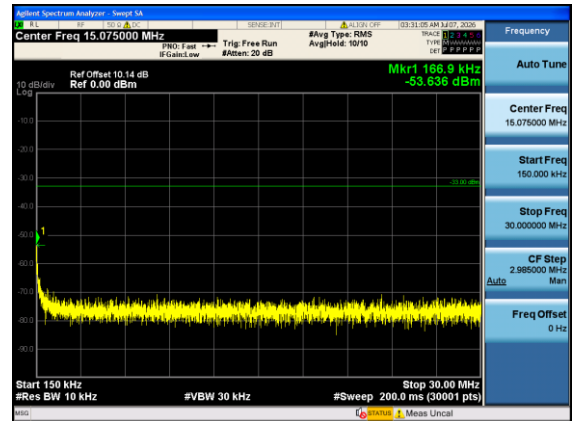
Band4-20MHz-QPSK-20050-1#0-0.15-30-PASS
