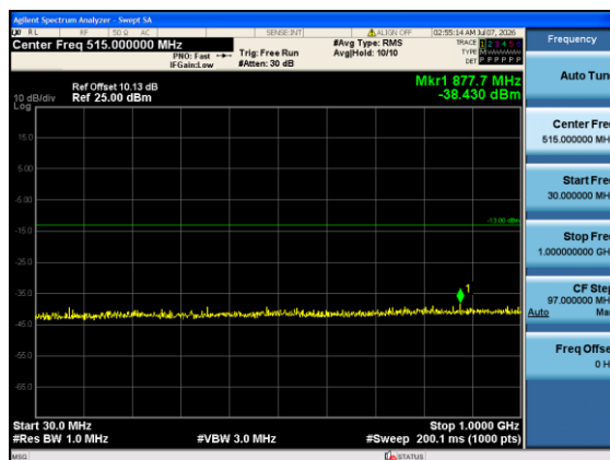
Band4-10MHz-QPSK-20175-1#0-30-1000-PASS
