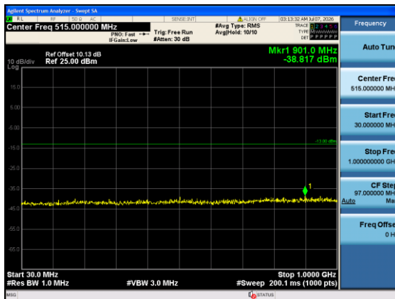
Band4-15MHz-16QAM-20175-1#0-30-1000-PASS
