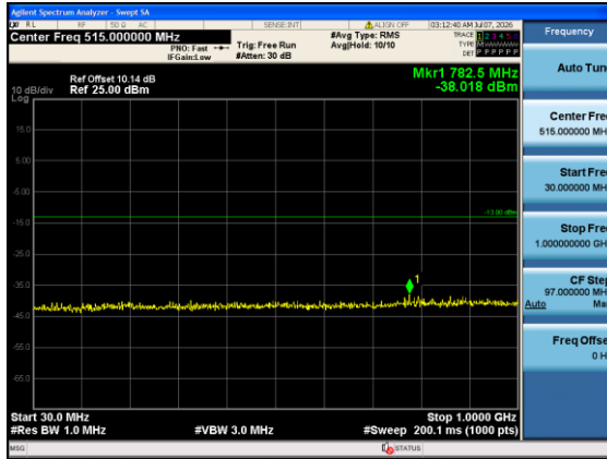
Band4-15MHz-16QAM-20025-1#0-30-1000-PASS
