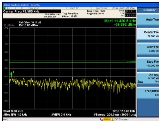
Band4-15MHz-16QAM-20325-1#5-0.009-0.15-PASS
