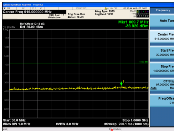
Band4-5MHz-16QAM-20175-1#0-30-1000-PASS
