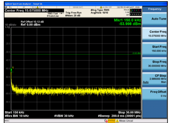
Band4-10MHz-16QAM-20175-1#0-0.15-30-PASS
