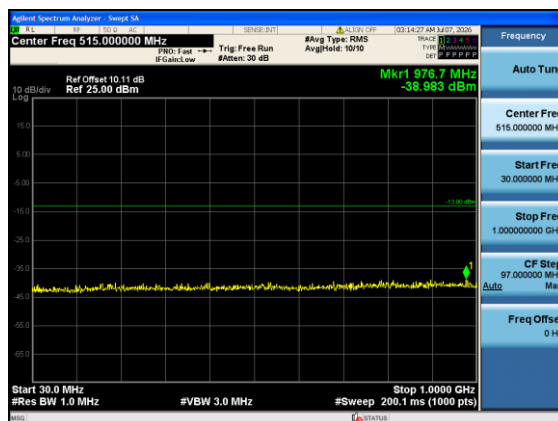
Band4-15MHz-16QAM-20325-1#5-30-1000-PASS
