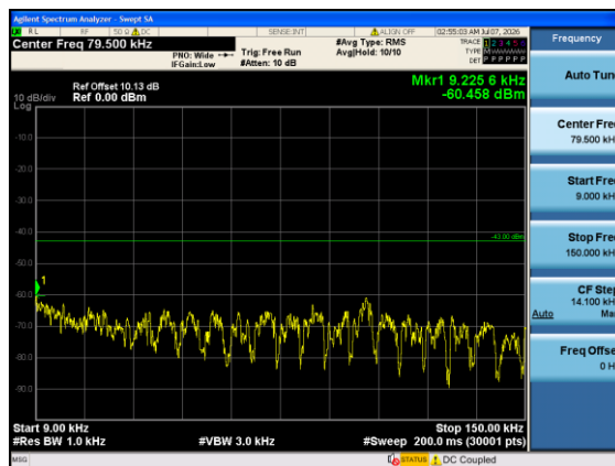
Band4-10MHz-QPSK-20175-1#0-0.009-0.15-PASS
