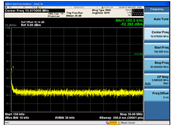
Band4-10MHz-QPSK-20000-1#0-0.15-30-PASS
