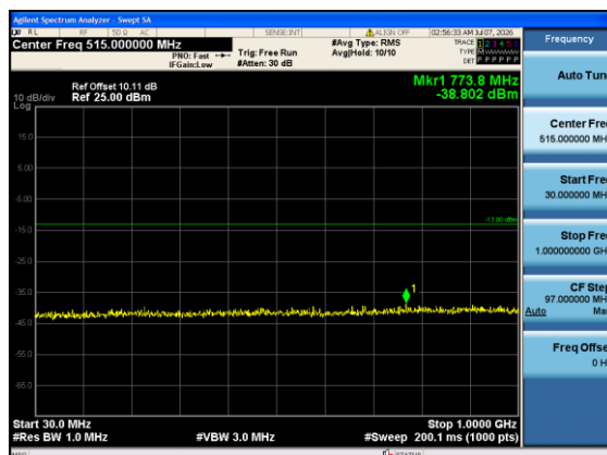
Band4-10MHz-16QAM-20350-1#5-30-1000-PASS
