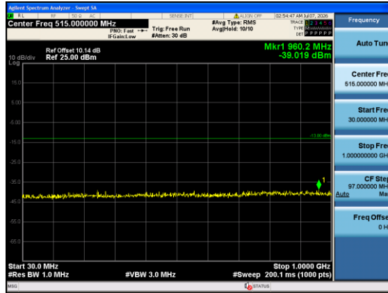
Band4-10MHz-16QAM-20000-1#0-30-1000-PASS
