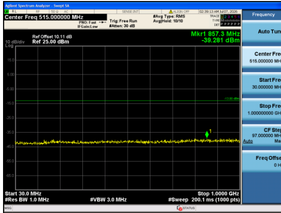
Band4-5MHz-QPSK-20375-1#5-30-1000-PASS
