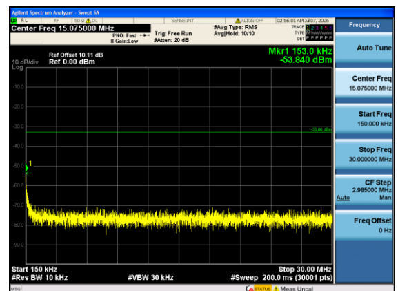
Band4-10MHz-QPSK-20350-1#5-0.15-30-PASS
