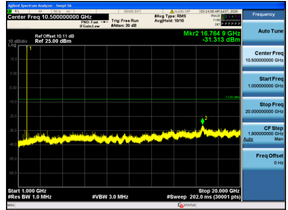
Band4-15MHz-QPSK-20325-1#5-1000-20000-PASS
