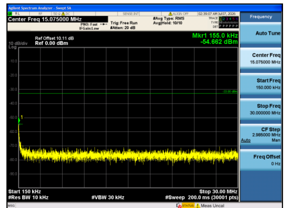
Band4-5MHz-QPSK-20375-1#5-0.15-30-PASS
