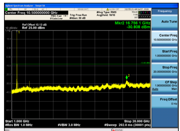
Band4-10MHz-QPSK-20175-1#0-1000-20000-PASS
