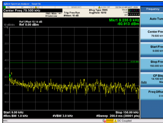
Band4-10MHz-QPSK-20000-1#0-0.009-0.15-PASS
