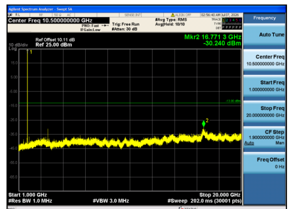
Band4-10MHz-16QAM-20350-1#5-1000-20000-PASS
