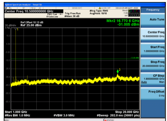
Band4-15MHz-QPSK-20175-1#0-1000-20000-PASS
