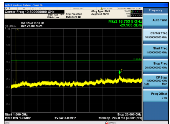
Band4-10MHz-16QAM-20175-1#0-1000-20000-PASS
