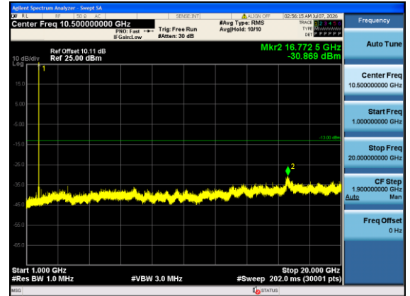
Band4-10MHz-QPSK-20350-1#5-1000-20000-PASS
