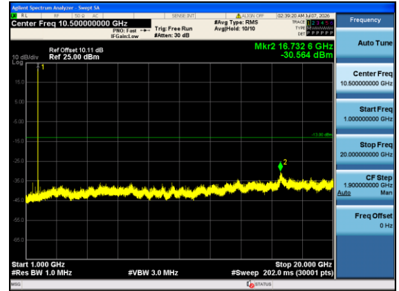
Band4-5MHz-QPSK-20375-1#5-1000-20000-PASS
