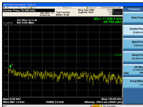
Band4-10MHz-16QAM-20000-1#0-0.009-0.15-PASS
