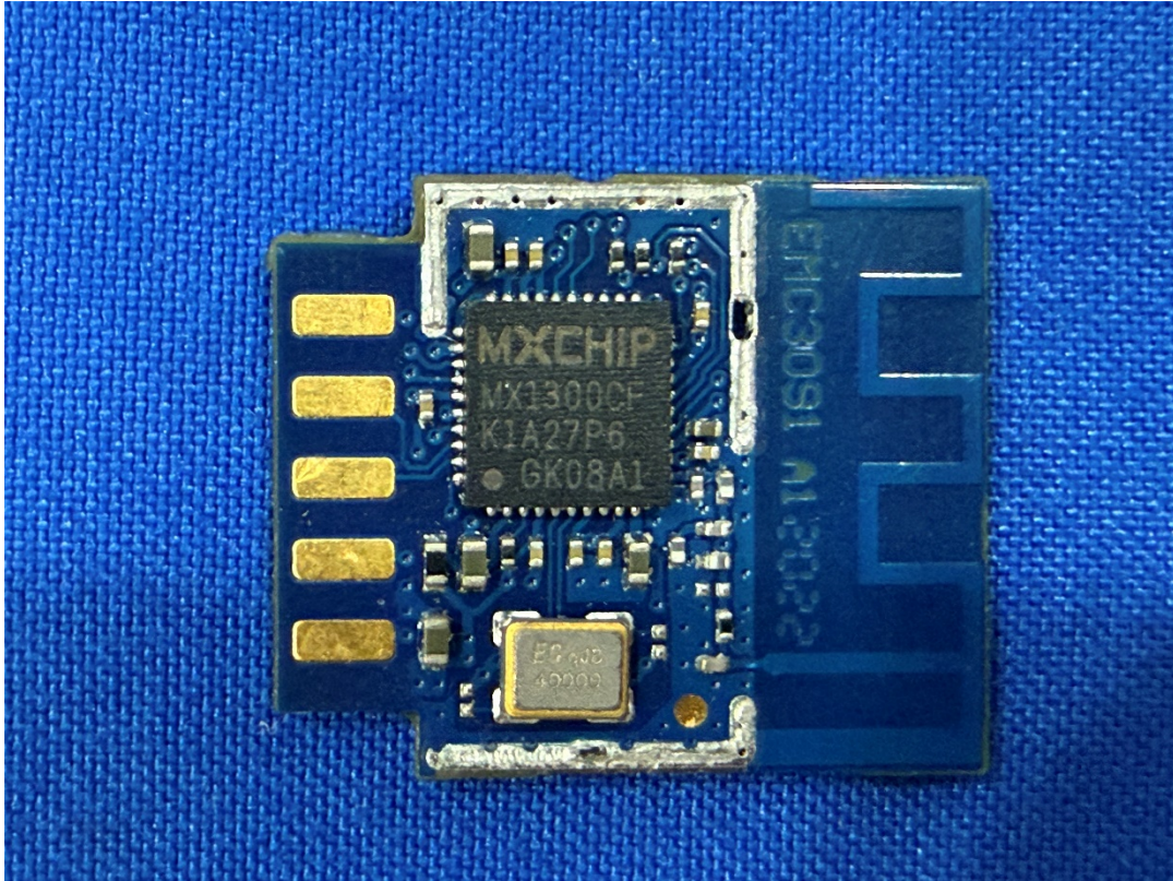
Photo 5: Internal View for BLE/WiFi Chip
