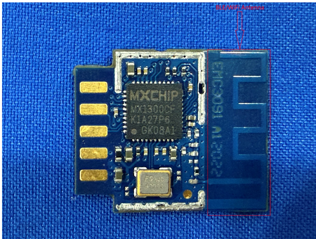
Photo 3: Internal View for BLE/WiFi Antenna
