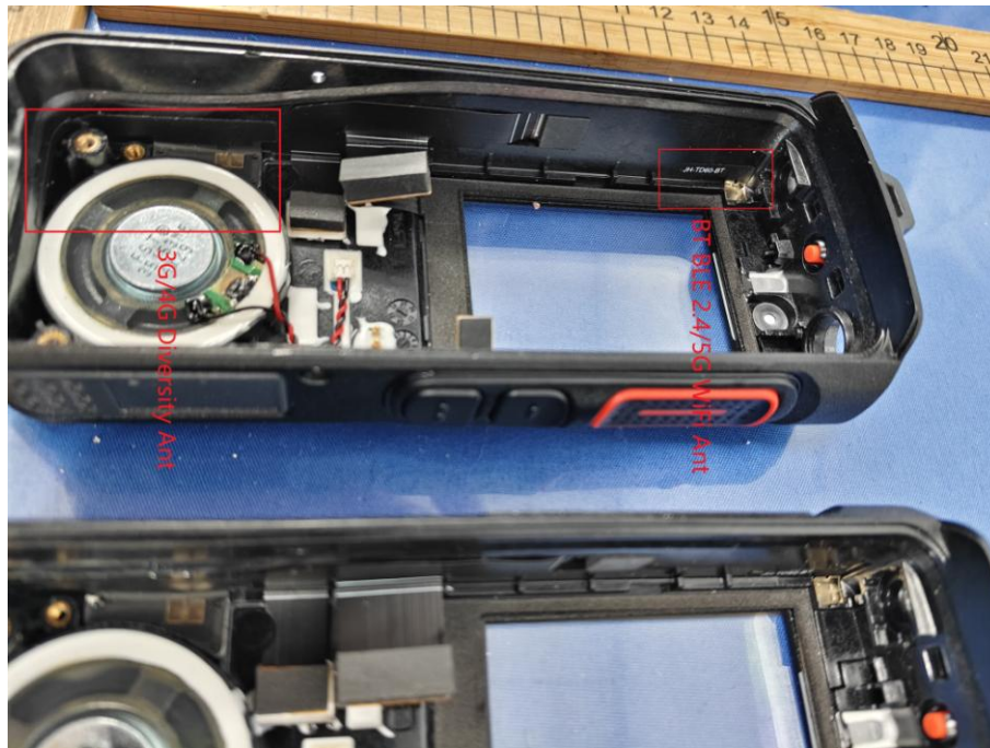
WWAN Diversity ANT
