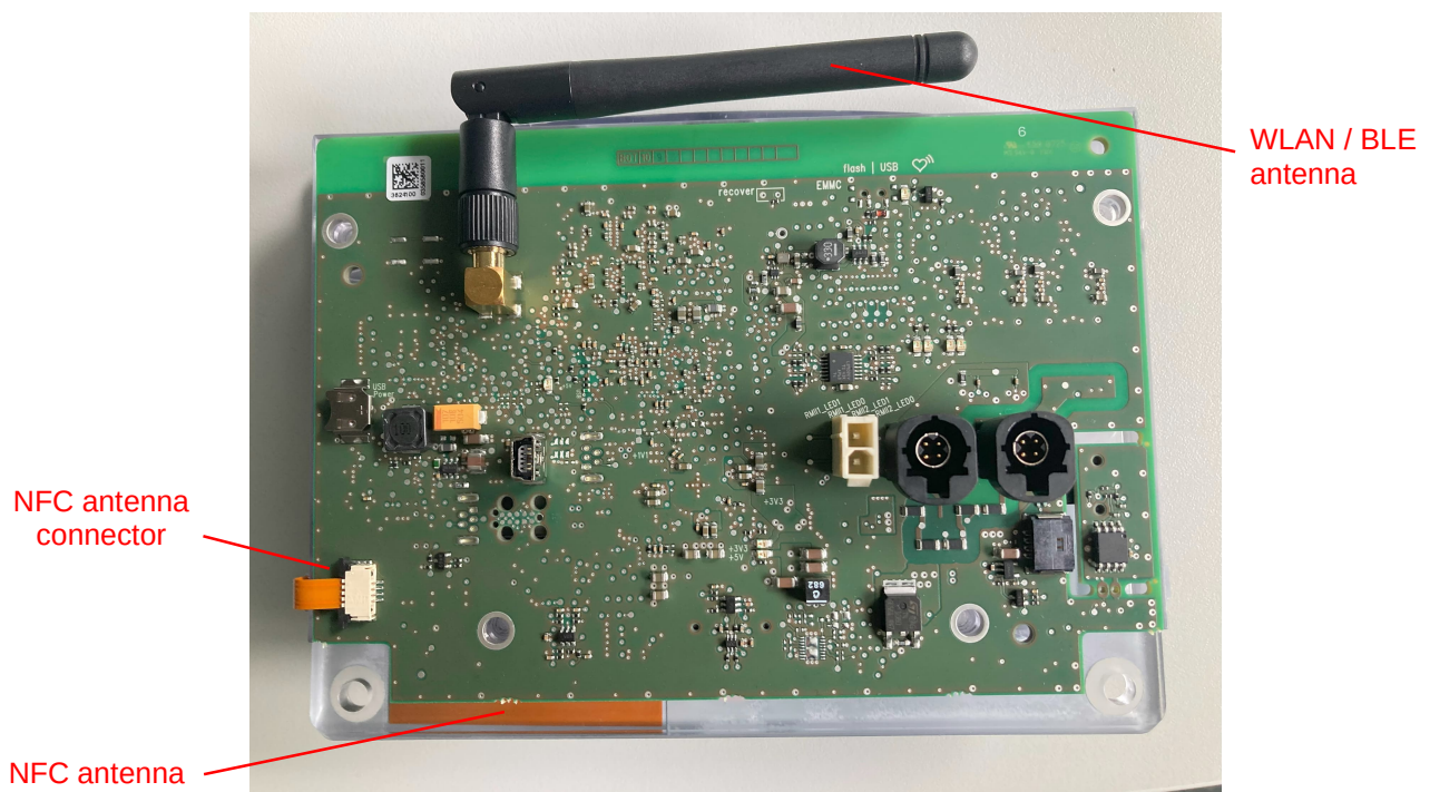
PCB – antennas connected *
