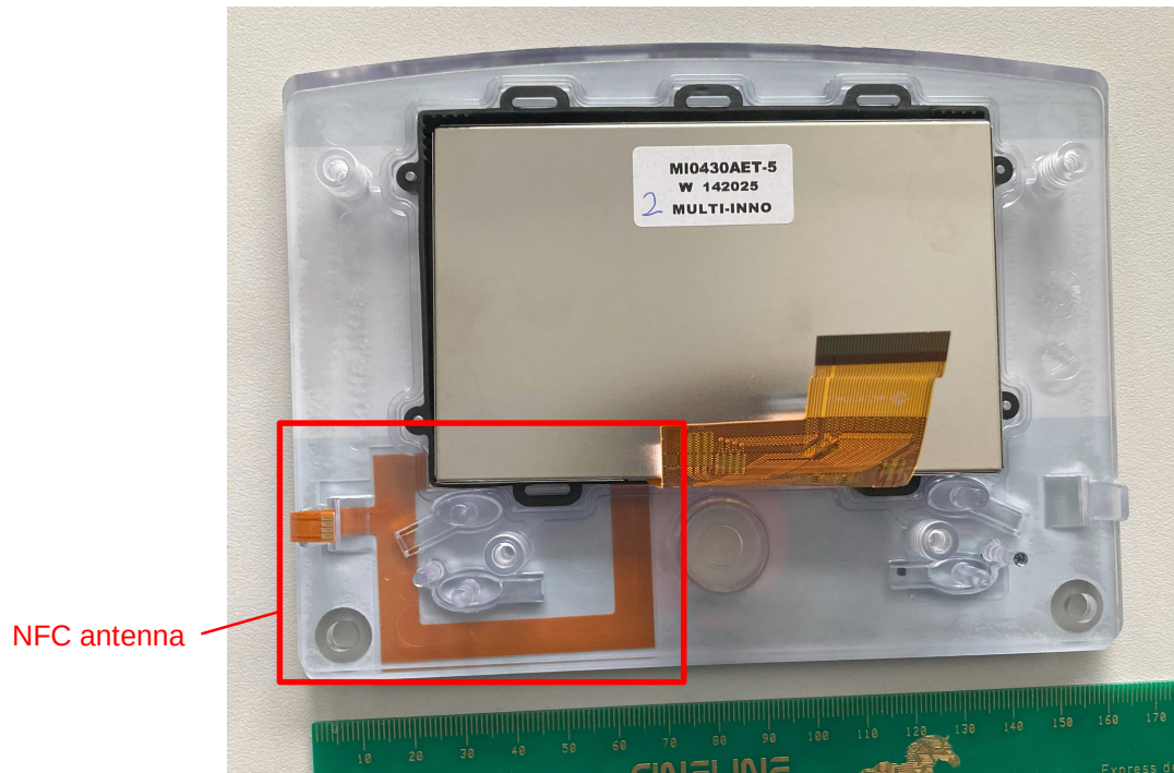
EUT – PCB and back cover removed *
