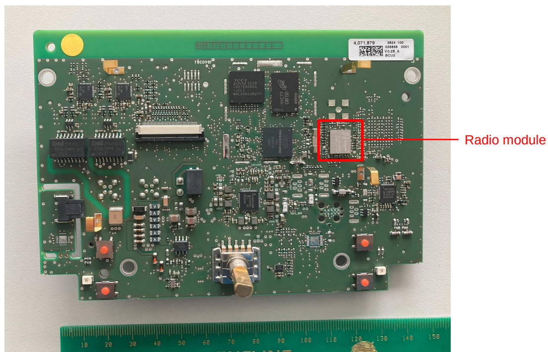
PCB – front view *
