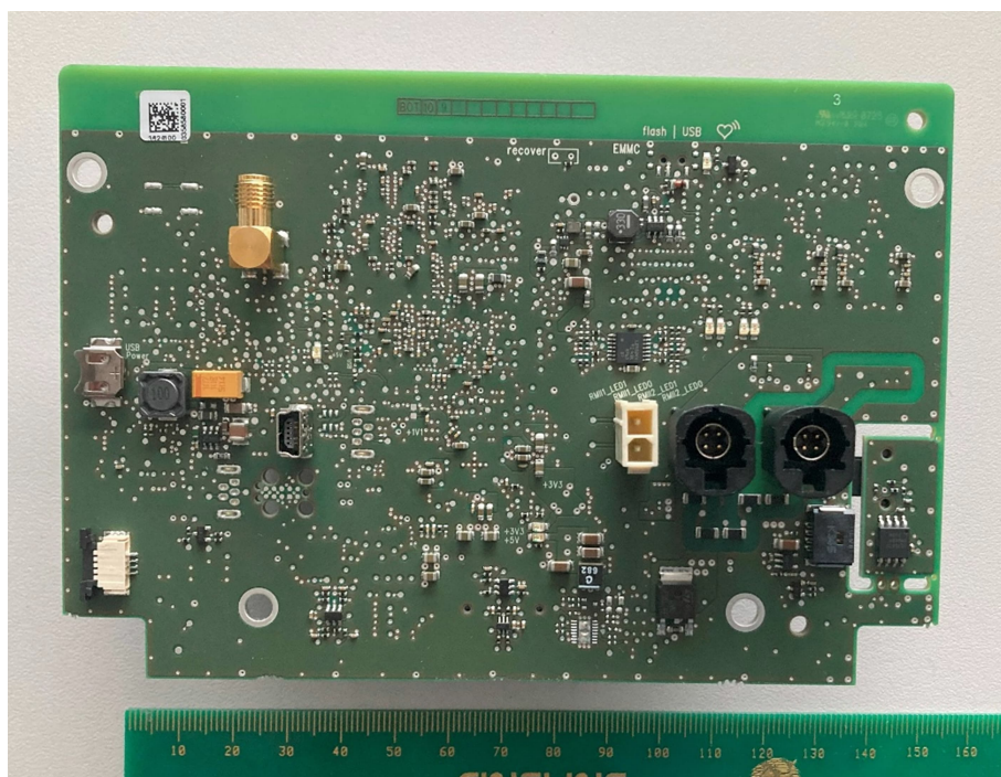
PCB – back view *
