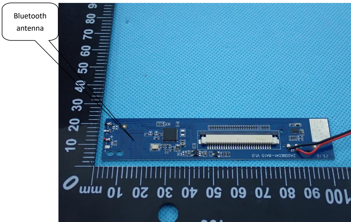
Internal Photo 4
