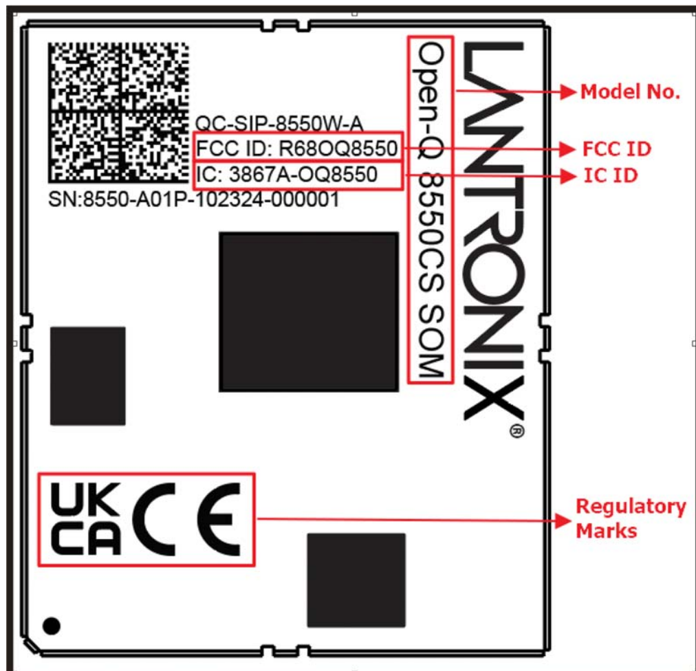
Top view of Module with Label etched unto metallic shield
