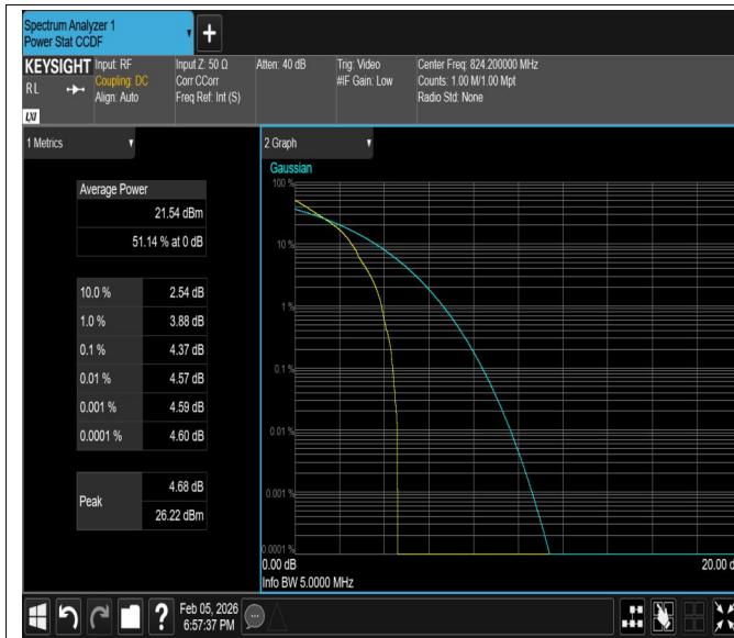
B26(824-849) -15KHz-QPSK-26915-12RB#0-PASS
