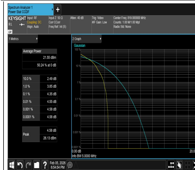
B26(814-824)-15KHz-QPSK-26740-12RB#0-PASS
