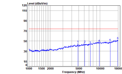
2.4G SRD_1M_TX_CH_19_Vertical-Peak
