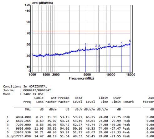
2.4G SRD_1M_TX_CH_00_Horizontal-Peak
