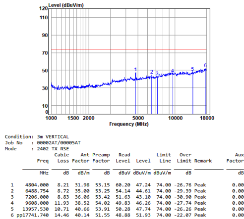
2.4G SRD_1M_TX_CH_00_Vertical-Peak
