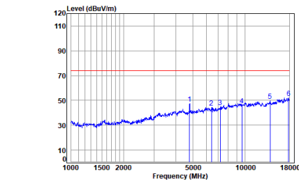
2.4G SRD_2M_TX_CH_00_Vertical-Peak
