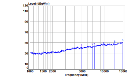
2.4G SRD_2M_TX_CH_39_Vertical-Peak
