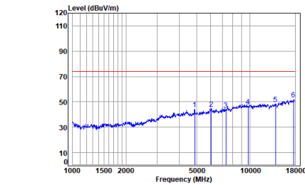
2.4G SRD_1M_TX_CH_19_Horizontal-Peak
