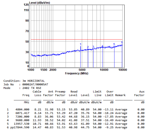
2.4G SRD_1M_TX_CH_00_Horizontal-Avg
