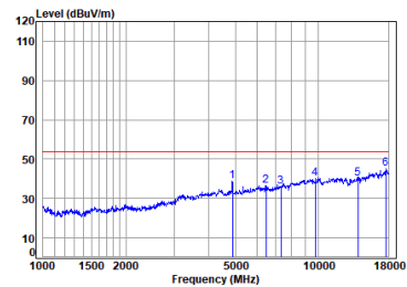
2.4G SRD_1M_TX_CH_19_Vertical-Avg
