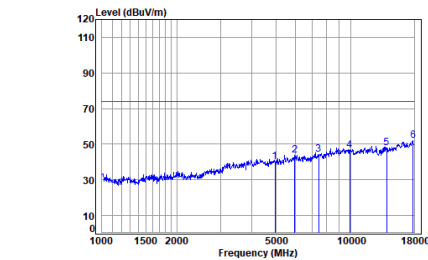
2.4G SRD_1M_TX_CH_39_Vertical-Peak
