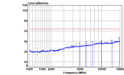
2.4G SRD_2M_TX_CH_39_Horizontal-Peak
