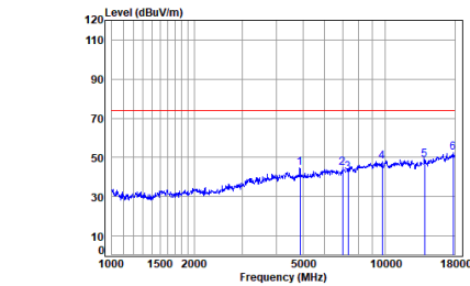
2.4G SRD_2M_TX_CH_19_Horizontal-Peak
