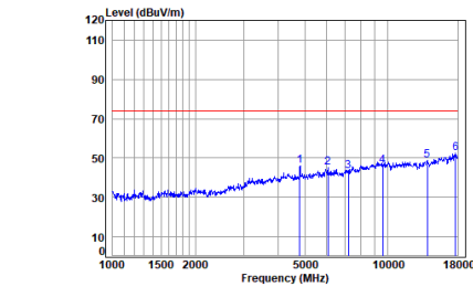
2.4G SRD_2M_TX_CH_00_Horizontal-Peak
