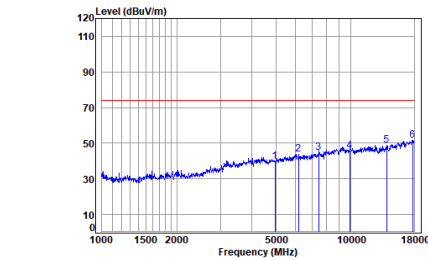
2.4G SRD_1M_TX_CH_39_Horizontal-Peak
