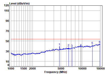
2.4G SRD_2M_TX_CH_00_Vertical-Avg
