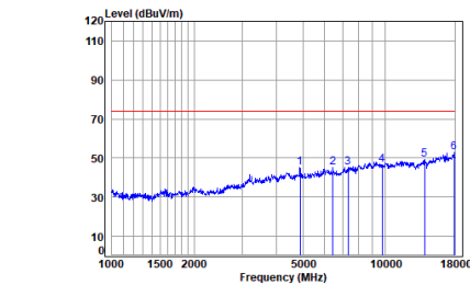
2.4G SRD_2M_TX_CH_19_Vertical-Peak
