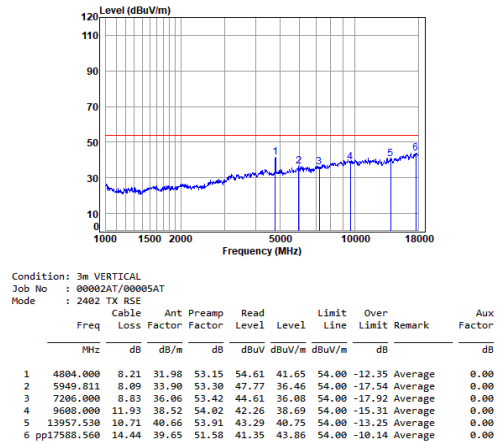
2.4G SRD_1M_TX_CH_00_Vertical-Avg
