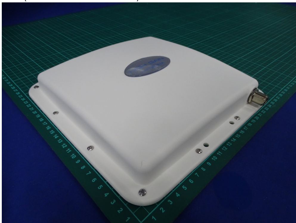
(10) EUT Photo (MOXA / ANT-WSB5-PNF-16)
