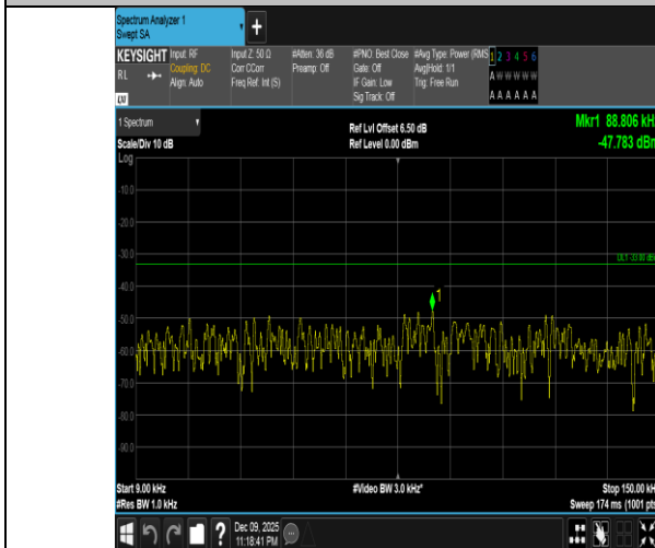
Band5-10MHz-QPSK-20525-1RB#0-0.009~0.15-PASS
