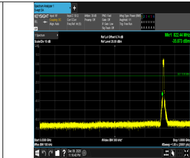
Band5-10MHz-16QAM-20450-50RB#0-30~1000-PASS
