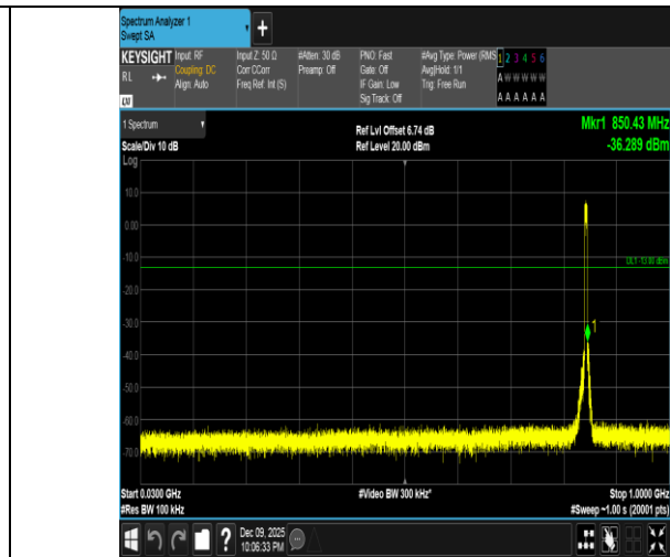
Band5-5MHz-16QAM-20625-25RB#0-30~1000-PASS
