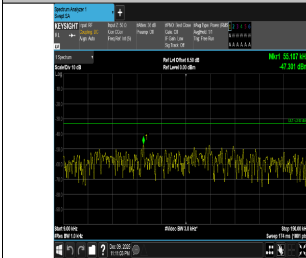
Band5-10MHz-QPSK-20450-50RB#0-0.009~0.15-PASS
