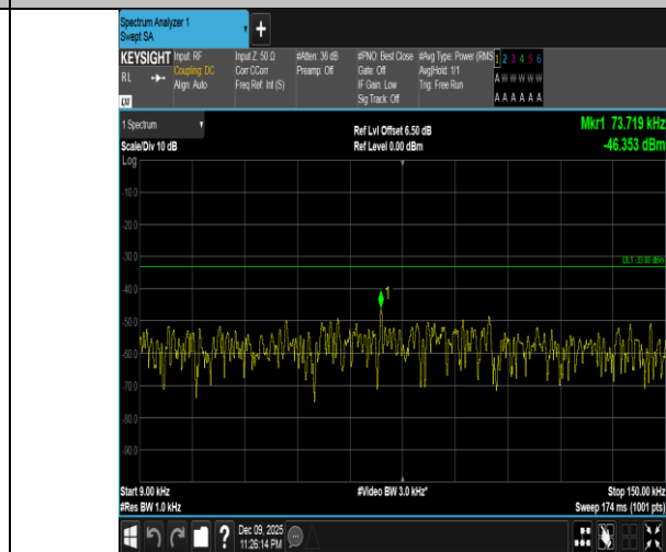
Band5-10MHz-QPSK-20525-1RB#49-0.009~0.15-PASS
