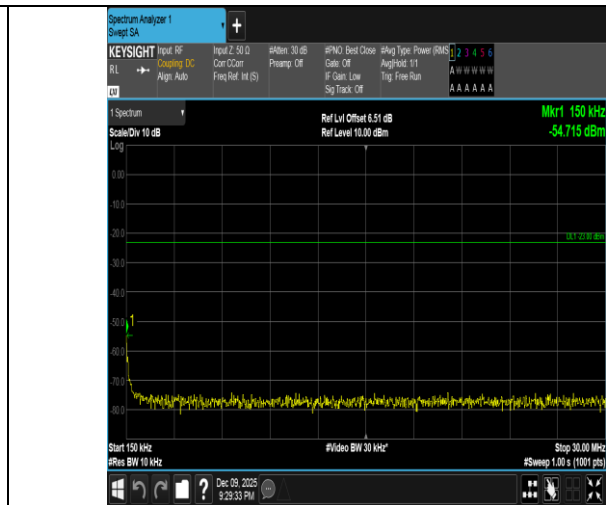
Band5-5MHz-16QAM-20525-1RB#24-0.15~30-PASS
