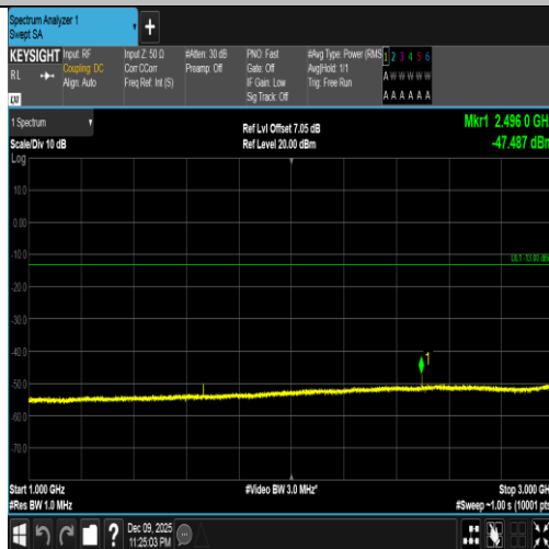
Band5-10MHz-16QAM-20525-1RB#0-1000~3000-PASS
