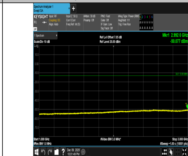
Band5-5MHz-QPSK-20625-25RB#0-1000~3000-PASS
