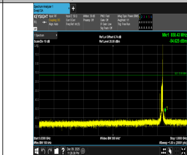
Band5-10MHz-QPSK-20525-1RB#49-30~1000-PASS
