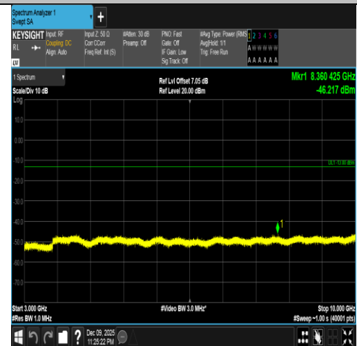
Band5-10MHz-16QAM-20525-1RB#0-3000~10000-PASS
