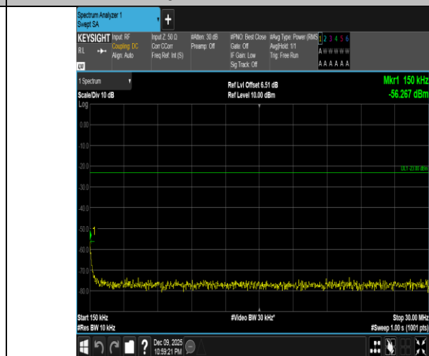
Band5-10MHz-QPSK-20450-1RB#0-0.15~30-PASS
