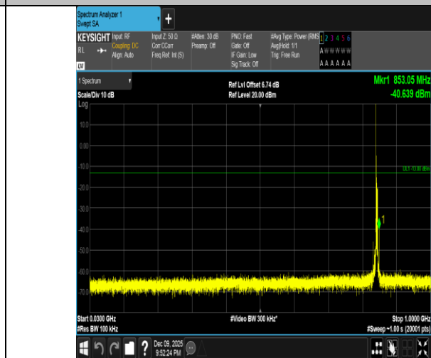
Band5-5MHz-16QAM-20625-1RB#0-30~1000-PASS
