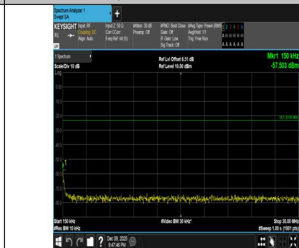
Band5-5MHz-QPSK-20625-1RB#0-0.15~30-PASS
