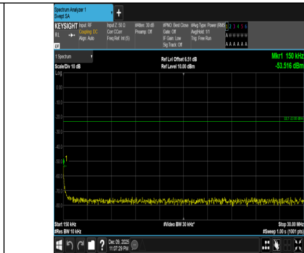
Band5-10MHz-16QAM-20450-1RB#49-0.15~30-PASS
