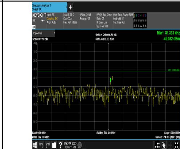
Band5-5MHz-16QAM-20625-25RB#0-0.009~0.15-PASS
