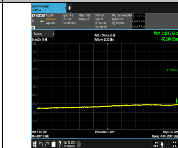
Band5-10MHz-QPSK-20525-50RB#0-1000~3000-PASS
