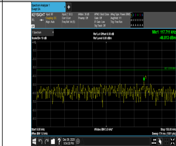
Band5-5MHz-QPSK-20625-1RB#24-0.009~0.15-PASS
