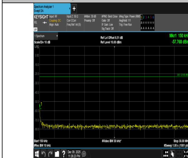
Band5-10MHz-QPSK-20525-1RB#49-0.15~30-PASS
