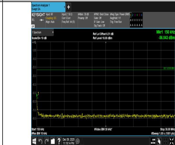
Band5-10MHz-QPSK-20525-1RB#0-0.15~30-PASS
