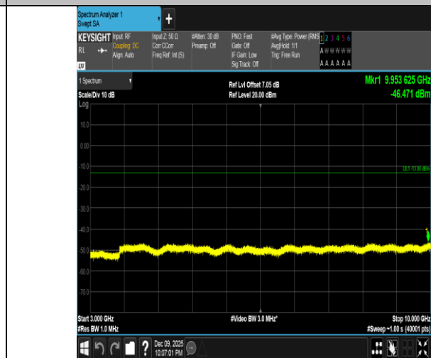
Band5-5MHz-16QAM-20625-25RB#0-3000~10000-PASS
