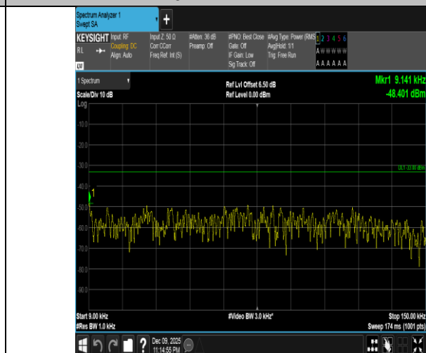
Band5-10MHz-16QAM-20450-50RB#0-0.009~0.15-PASS
