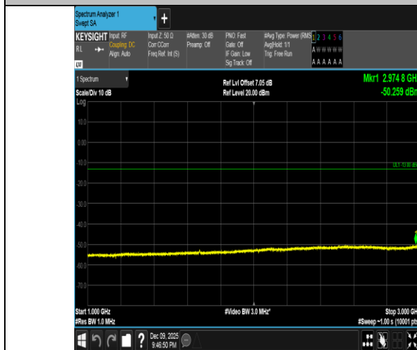
Band5-5MHz-16QAM-20525-25RB#0-1000~3000-PASS
