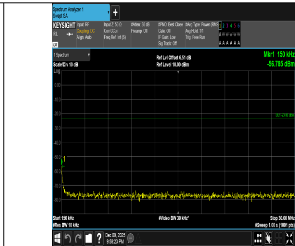
Band5-5MHz-16QAM-20625-1RB#24-0.15~30-PASS
