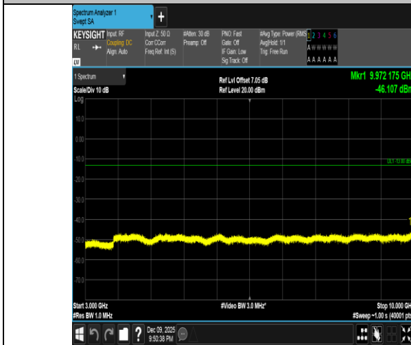
Band5-5MHz-QPSK-20625-1RB#0-3000~10000-PASS
