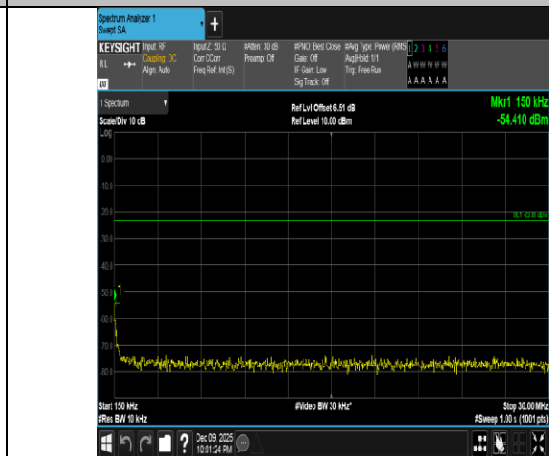
Band5-5MHz-QPSK-20625-25RB#0-0.15~30-PASS
