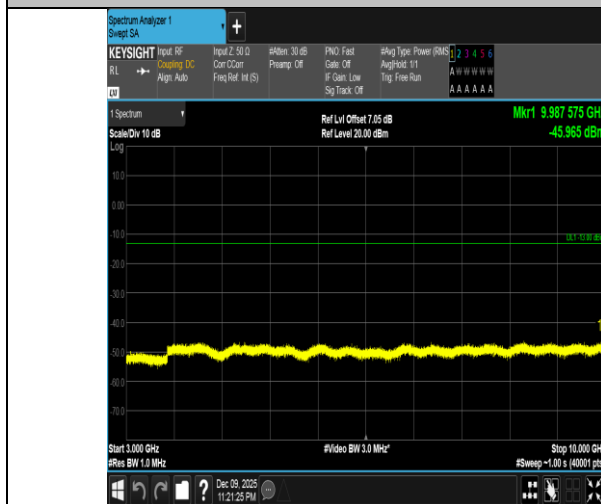
Band5-10MHz-QPSK-20525-1RB#0-3000~10000-PASS
