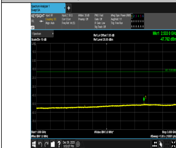
Band5-5MHz-16QAM-20625-1RB#0-1000~3000-PASS
