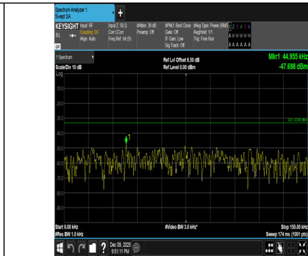
Band5-5MHz-16QAM-20625-1RB#0-0.009~0.15-PASS
