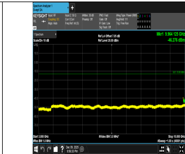
Band5-5MHz-QPSK-20625-1RB#24-3000~10000-PASS
