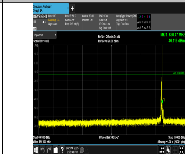
Band5-5MHz-QPSK-20625-1RB#24-30~1000-PASS
