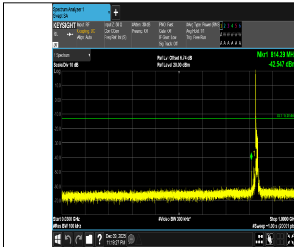
Band5-10MHz-QPSK-20525-1RB#0-30~1000-PASS
