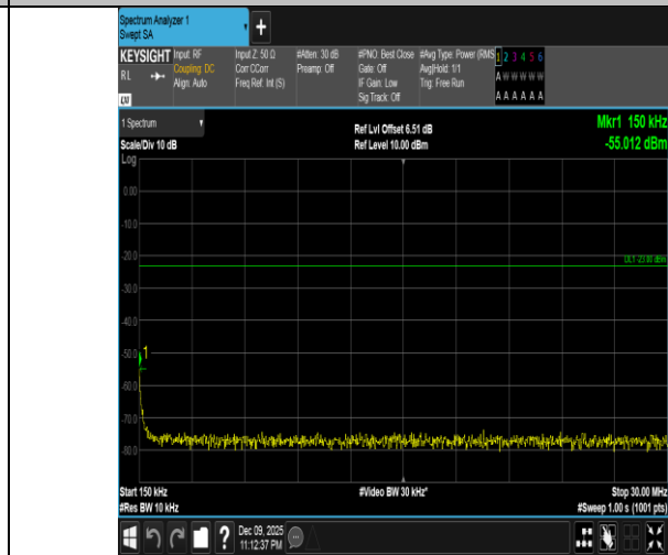
Band5-10MHz-QPSK-20450-50RB#0-0.15~30-PASS
