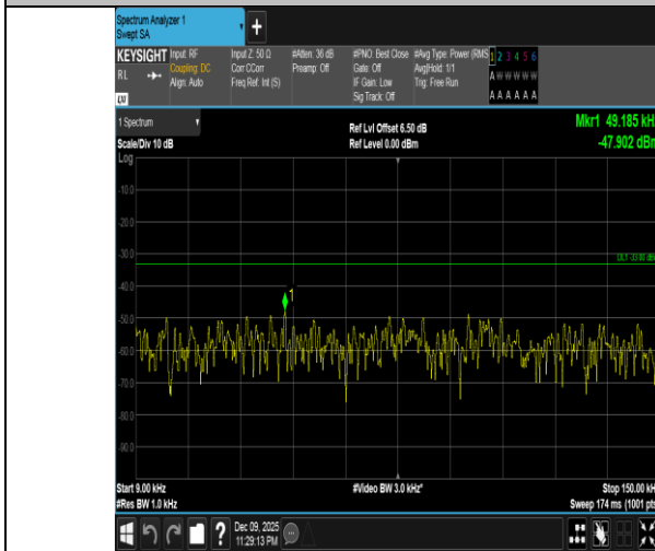
Band5-10MHz-QPSK-20525-50RB#0-0.009~0.15-PASS
