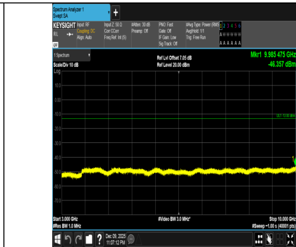
Band5-10MHz-QPSK-20450-1RB#49-3000~10000-PASS
