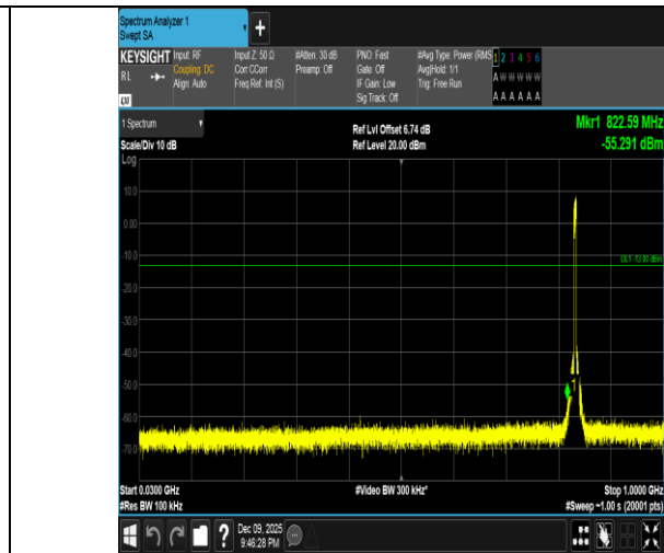
Band5-5MHz-16QAM-20525-25RB#0-30~1000-PASS
