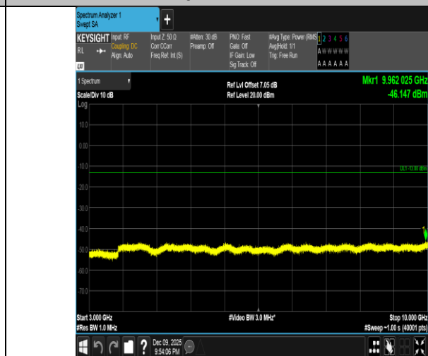
Band5-5MHz-16QAM-20625-1RB#0-3000~10000-PASS
