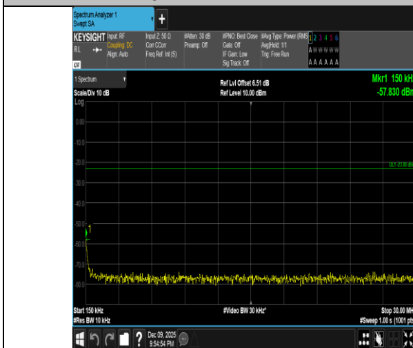
Band5-5MHz-QPSK-20625-1RB#24-0.15~30-PASS
