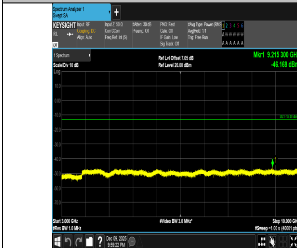
Band5-5MHz-16QAM-20625-1RB#24-3000~10000-PASS
