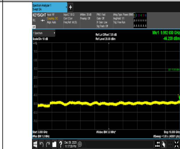
Band5-10MHz-16QAM-20450-50RB#0-3000~10000-PASS
