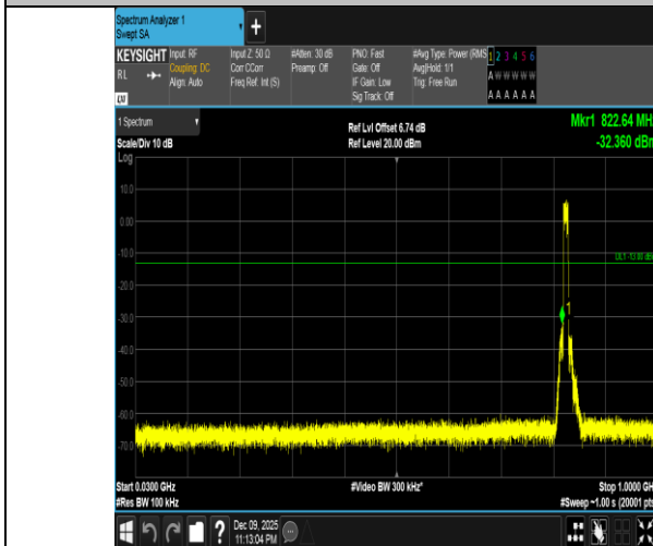
Band5-10MHz-QPSK-20450-50RB#0-30~1000-PASS
