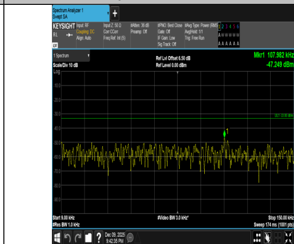
Band5-5MHz-16QAM-20525-25RB#0-0.009~0.15-PASS
