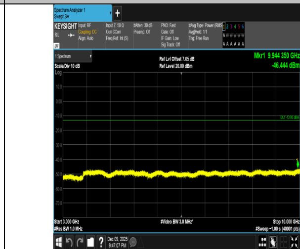
Band5-5MHz-16QAM-20525-25RB#0-3000~10000-PASS
