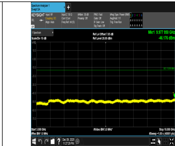
Band5-10MHz-QPSK-20525-1RB#49-3000~10000-PASS
