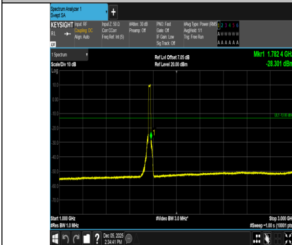
Band66-20MHz-16QAM-132572-100RB#0-1000~3000-PASS
