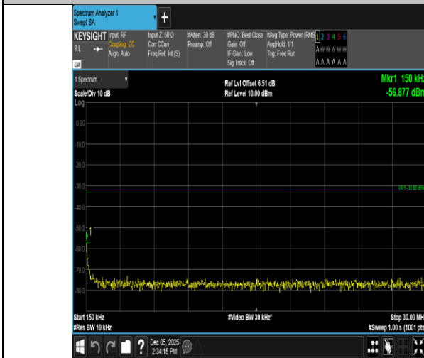
Band66-20MHz-16QAM-132572-100RB#0-0.15~30-PASS
