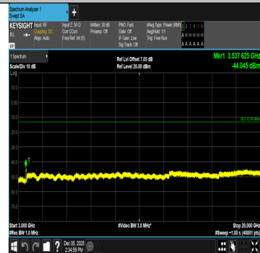
Band66-20MHz-16QAM-132572-100RB#0-3000~20000-PASS
