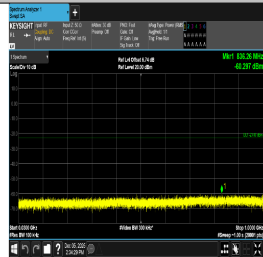
Band66-20MHz-16QAM-132572-100RB#0-30~1000-PASS
