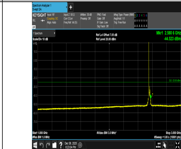
Band7-20MHz-16QAM-21350-1RB#0-1000~3000-PASS
