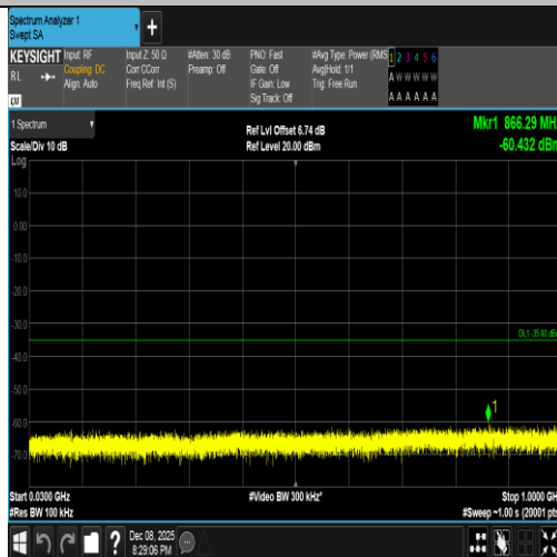
Band7-20MHz-16QAM-21350-100RB#0-30~1000-PASS
