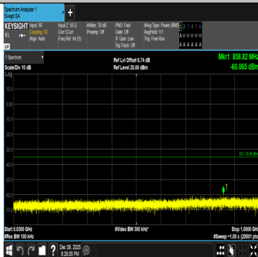
Band7-20MHz-16QAM-21350-1RB#99-30~1000-PASS
