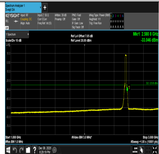
Band7-20MHz-16QAM-21350-100RB#0-1000~3000-PASS
