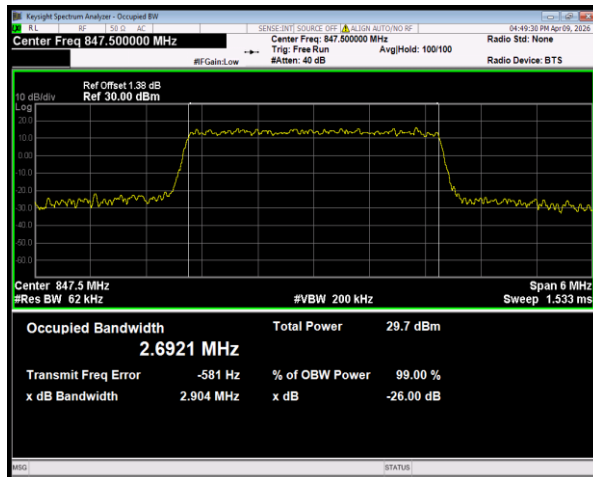
Band26(824-849) QPSK BW=3MHz Channel=27025 RB Size=15 Position=#0
