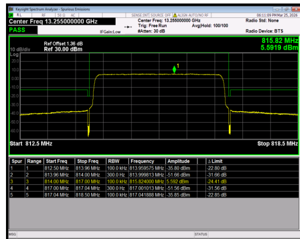
Band26(814-824) 16QAM BW=3MHz LowChannel=26705 RB Size=15 Position=#0
