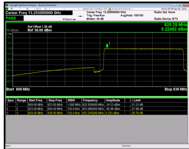
Band26(824-849) 16QAM BW=15MHz LowChannel=26865 RB Size=75 Position=#0
