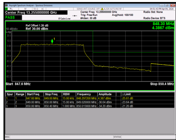
Band26(824-849) 16QAM BW=1.4MHz HighChannel=27033 RB Size=6 Position=#0
