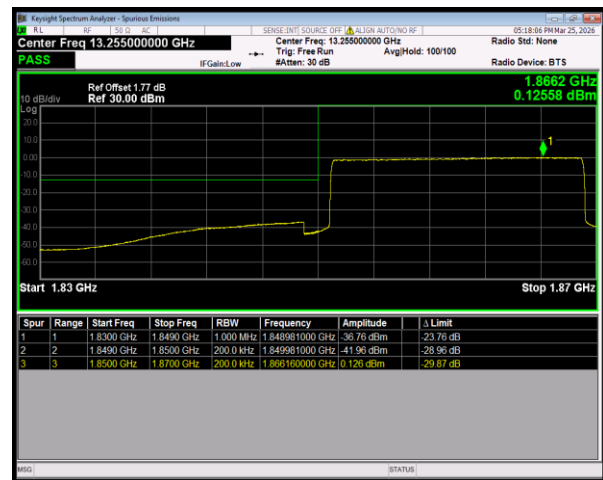
Band25 16QAM BW=20MHz LowChannel=26140 RB Size=100 Position=#0
