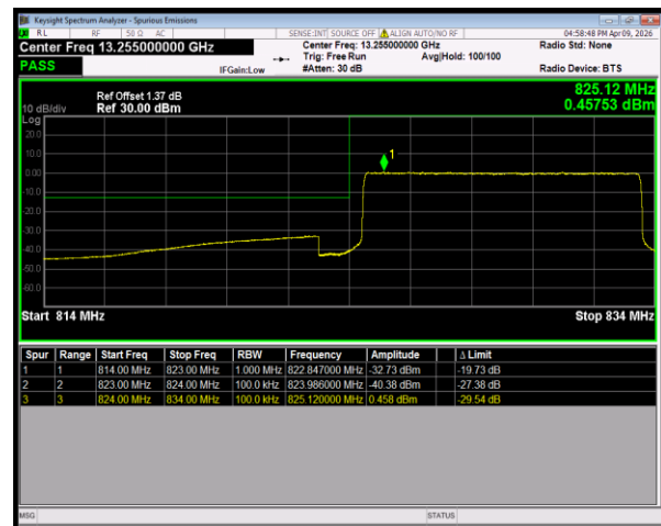
Band26(824-849) 16QAM BW=10MHz LowChannel=26840 RB Size=50 Position=#0
