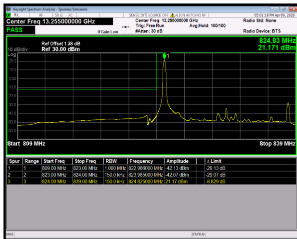
Band26(824-849) QPSK BW=15MHz LowChannel=26865 RB Size=1 Position=#0
