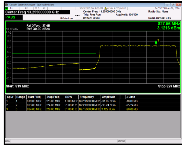
Band26(824-849) 16QAM BW=5MHz LowChannel=26815 RB Size=25 Position=#0
