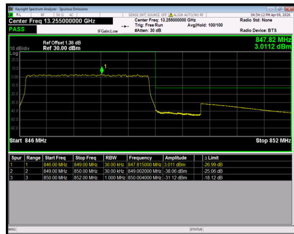
Band26(824-849) 16QAM BW=3MHz HighChannel=27025 RB Size=15 Position=#0
