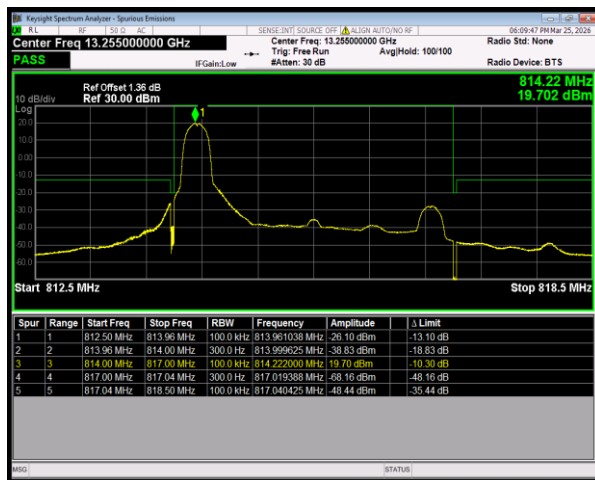
Band26(814-824) QPSK BW=3MHz LowChannel=26705 RB Size=1 Position=#0
