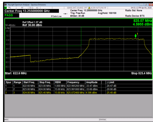
Band26(824-849) 16QAM BW=1.4MHz LowChannel=26797 RB Size=6 Position=#0
