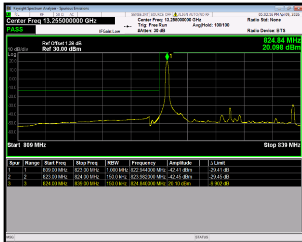
Band26(824-849) 16QAM BW=15MHz LowChannel=26865 RB Size=1 Position=#0
