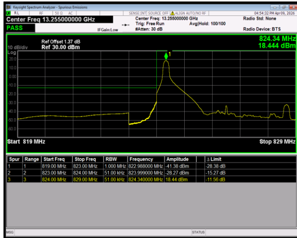
Band26(824-849) QPSK BW=5MHz LowChannel=26815 RB Size=1 Position=#0
