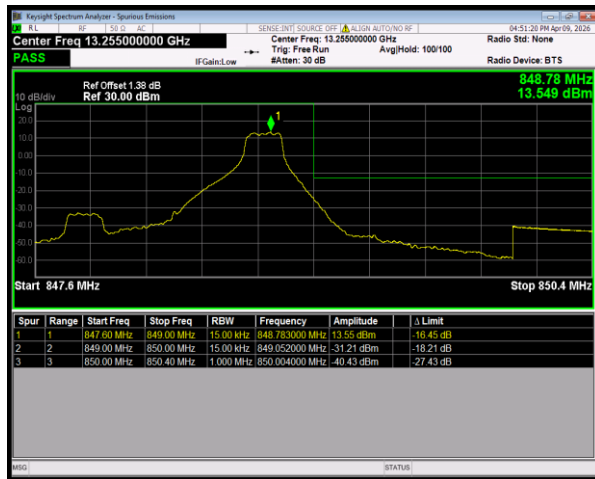
Band26(824-849) QPSK BW=1.4MHz HighChannel=27033 RB Size=1 Position=#Max
