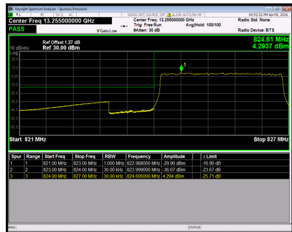
Band26(824-849) QPSK BW=3MHz LowChannel=26805 RB Size=15 Position=#0
