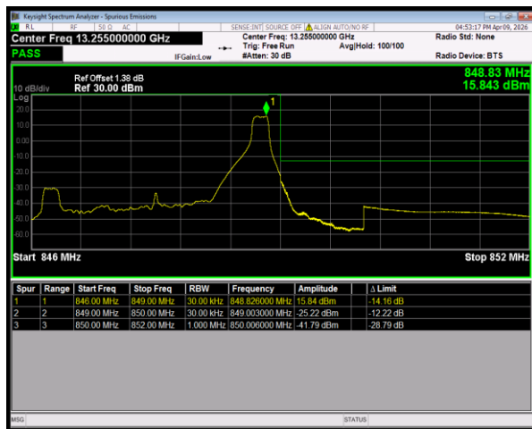
Band26(824-849) QPSK BW=3MHz HighChannel=27025 RB Size=1 Position=#Max
