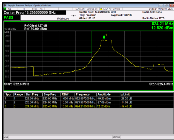
Band26(824-849) 16QAM BW=1.4MHz LowChannel=26797 RB Size=1 Position=#0
