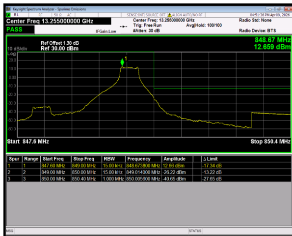
Band26(824-849) 16QAM BW=1.4MHz HighChannel=27033 RB Size=1 Position=#Max
