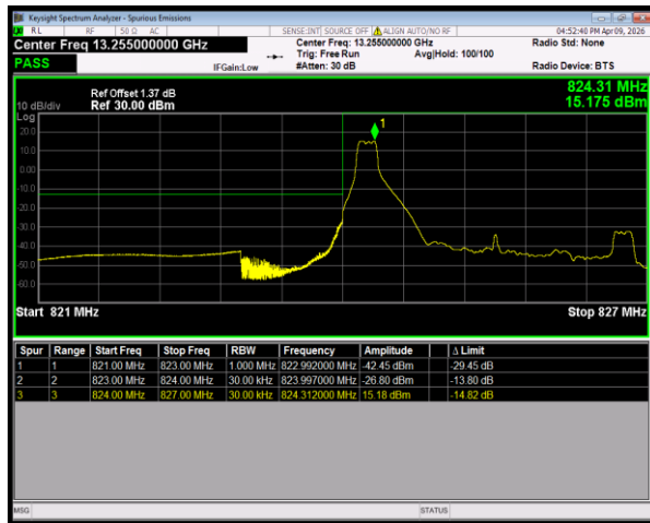
Band26(824-849) 16QAM BW=3MHz LowChannel=26805 RB Size=1 Position=#0
