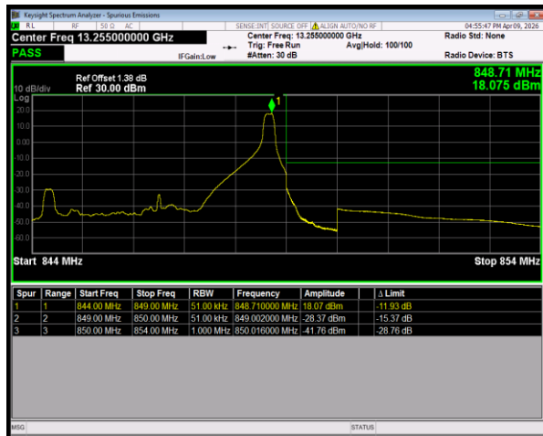
Band26(824-849) QPSK BW=5MHz HighChannel=27015 RB Size=1 Position=#Max
