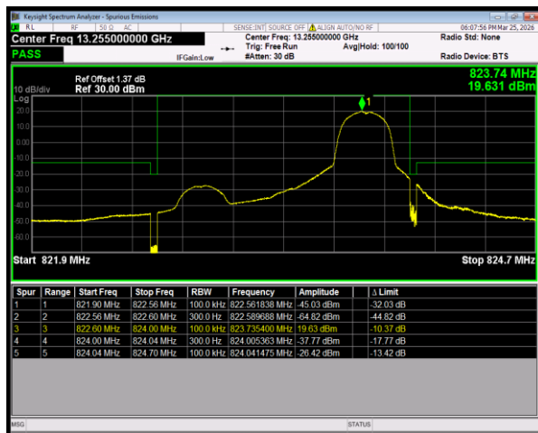
Band26(814-824) QPSK BW=1.4MHz HighChannel=26783 RB Size=1 Position=#Max
