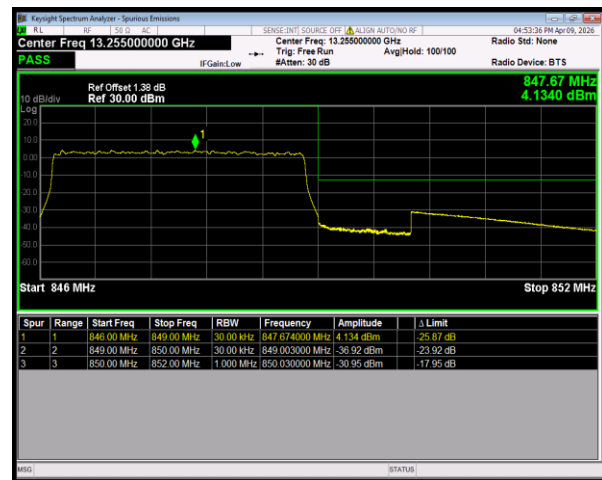
Band26(824-849) QPSK BW=3MHz HighChannel=27025 RB Size=15 Position=#0
