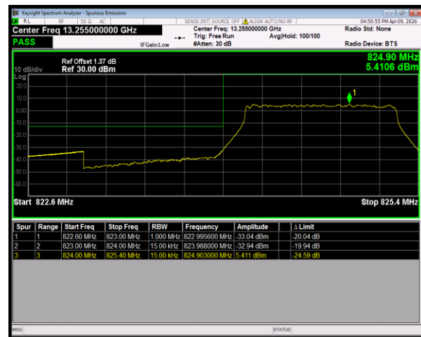
Band26(824-849) QPSK BW=1.4MHz LowChannel=26797 RB Size=6 Position=#0
