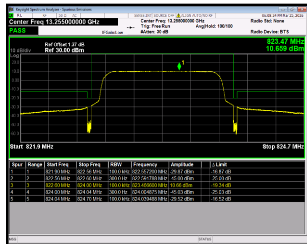
Band26(814-824) QPSK BW=1.4MHz HighChannel=26783 RB Size=6 Position=#0
