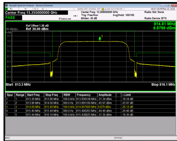
Band26(814-824) 16QAM BW=1.4MHz LowChannel=26697 RB Size=6 Position=#0
