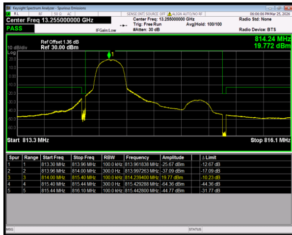
Band26(814-824) QPSK BW=1.4MHz LowChannel=26697 RB Size=1 Position=#0
