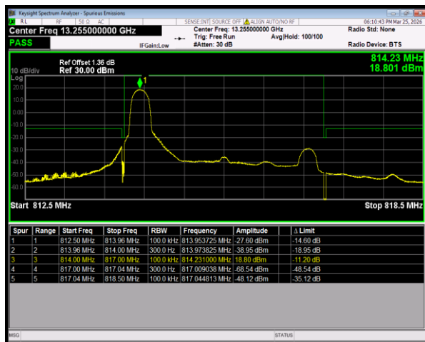
Band26(814-824) 16QAM BW=3MHz LowChannel=26705 RB Size=1 Position=#0
