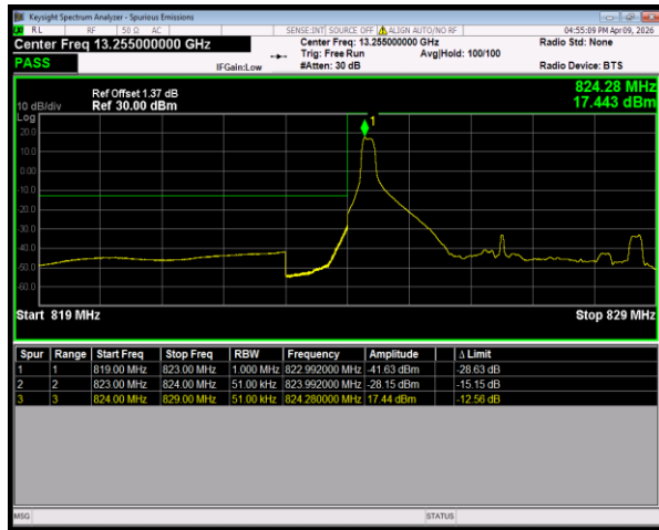
Band26(824-849) 16QAM BW=5MHz LowChannel=26815 RB Size=1 Position=#0
