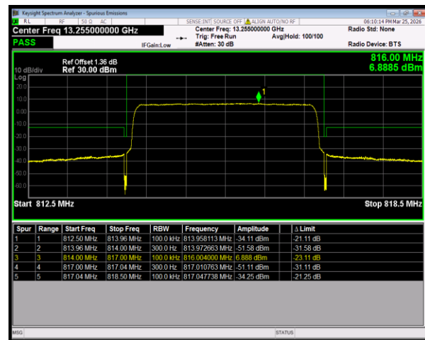
Band26(814-824) QPSK BW=3MHz LowChannel=26705 RB Size=15 Position=#0
