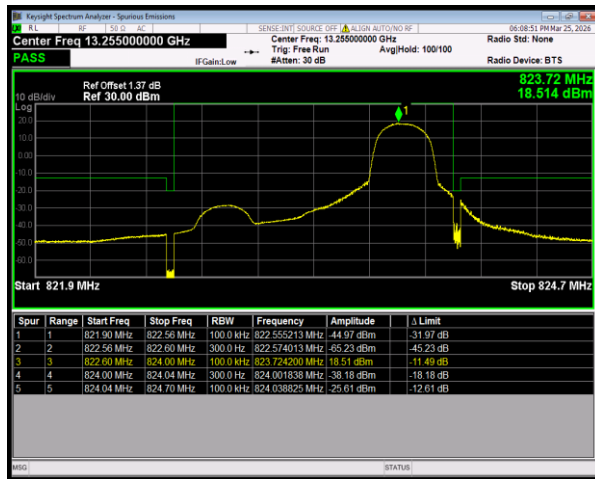
Band26(814-824) 16QAM BW=1.4MHz HighChannel=26783 RB Size=1 Position=#Max
