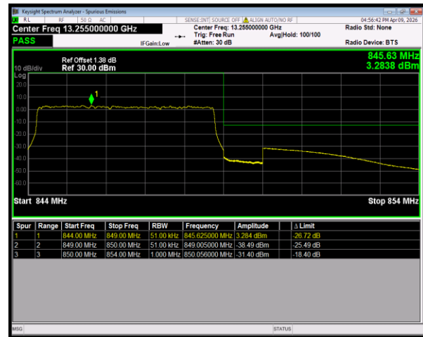
Band26(824-849) 16QAM BW=5MHz HighChannel=27015 RB Size=25 Position=#0
