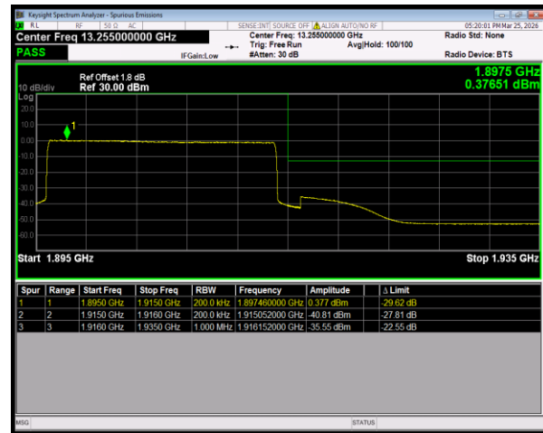
Band25 16QAM BW=20MHz HighChannel=26590 RB Size=100 Position=#0
