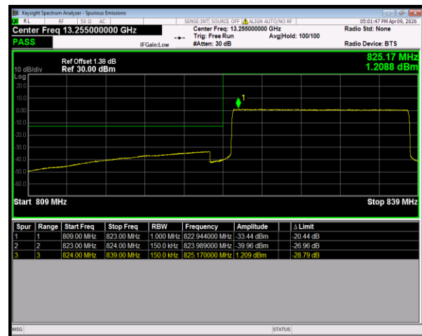
Band26(824-849) QPSK BW=15MHz LowChannel=26865 RB Size=75 Position=#0
