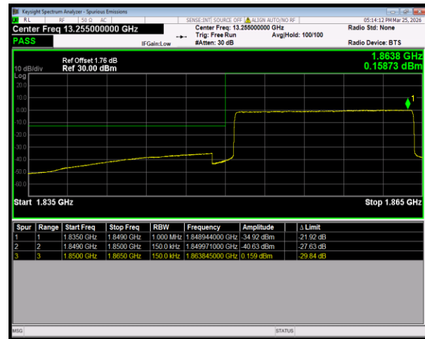
Band25 16QAM BW=15MHz LowChannel=26115 RB Size=75 Position=#0
