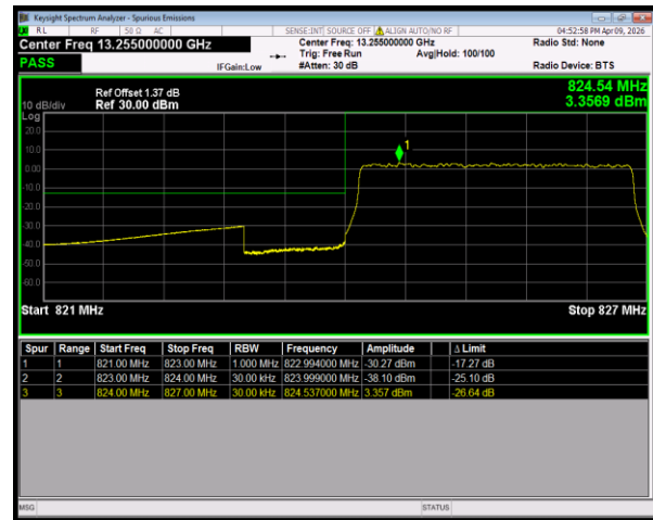
Band26(824-849) 16QAM BW=3MHz LowChannel=26805 RB Size=15 Position=#0
