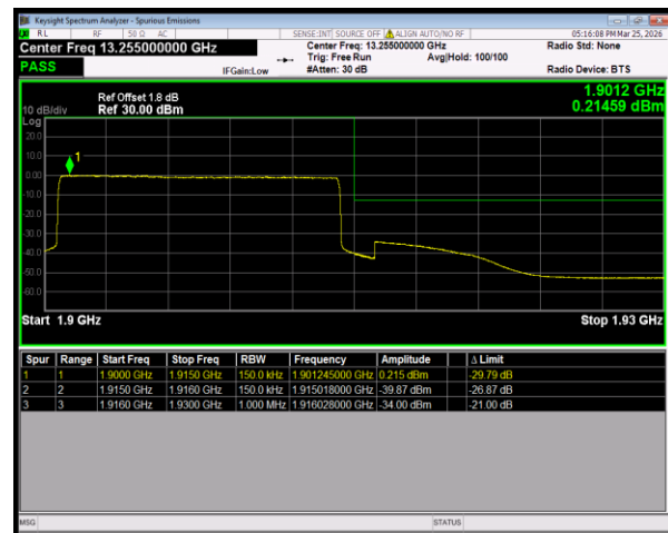
Band25 16QAM BW=15MHz HighChannel=26615 RB Size=75 Position=#0
