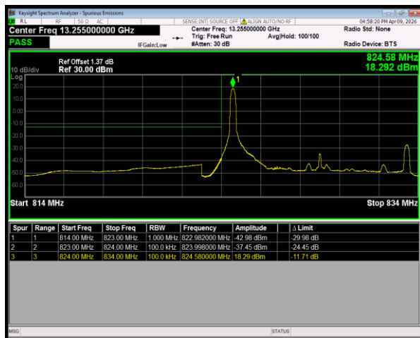
Band26(824-849) 16QAM BW=10MHz LowChannel=26840 RB Size=1 Position=#0
