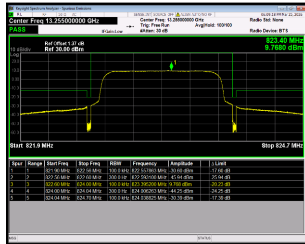
Band26(814-824) 16QAM BW=1.4MHz HighChannel=26783 RB Size=6 Position=#0
