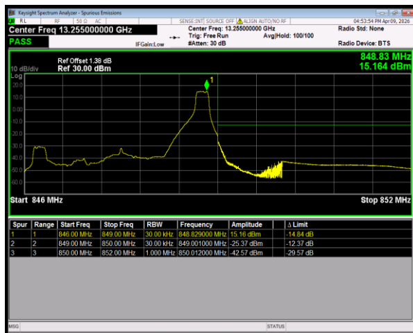
Band26(824-849) 16QAM BW=3MHz HighChannel=27025 RB Size=1 Position=#Max
