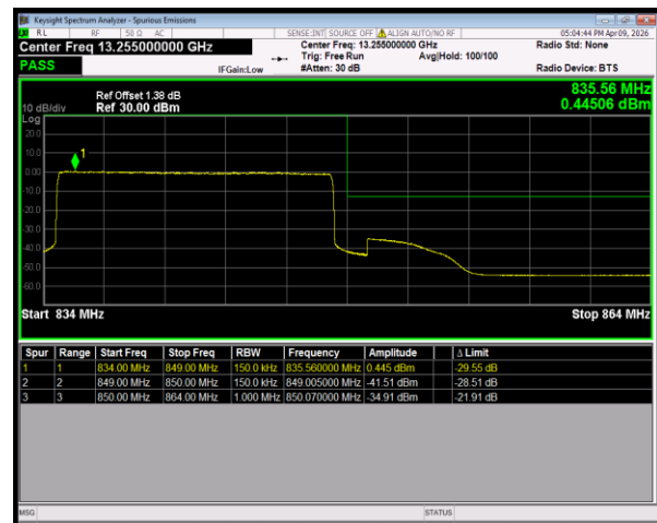
Band26(824-849) 16QAM BW=15MHz HighChannel=26965 RB Size=75 Position=#0
