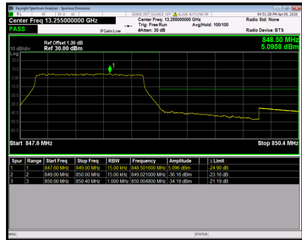
Band26(824-849) QPSK BW=1.4MHz HighChannel=27033 RB Size=6 Position=#0
