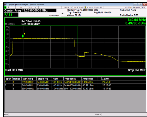
Band26(824-849) 16QAM BW=10MHz HighChannel=26990 RB Size=50 Position=#0
