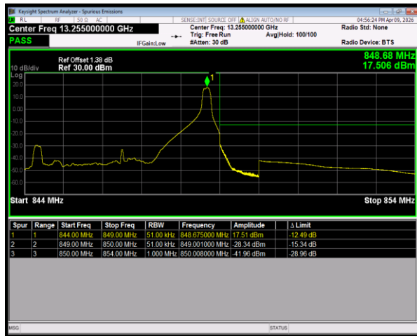
Band26(824-849) 16QAM BW=5MHz HighChannel=27015 RB Size=1 Position=#Max
