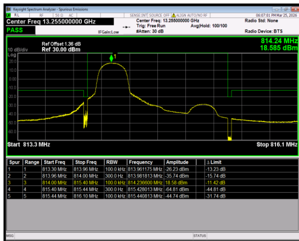
Band26(814-824) 16QAM BW=1.4MHz LowChannel=26697 RB Size=1 Position=#0
