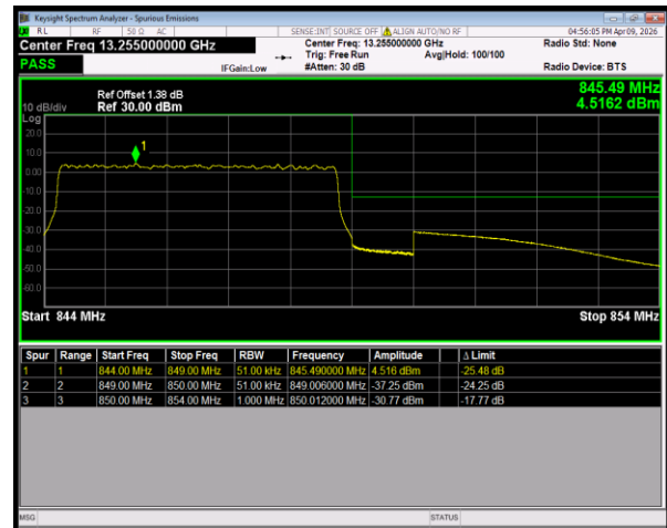
Band26(824-849) QPSK BW=5MHz HighChannel=27015 RB Size=25 Position=#0
