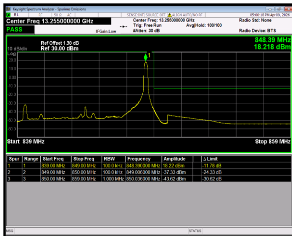
Band26(824-849) 16QAM BW=10MHz HighChannel=26990 RB Size=1 Position=#Max
