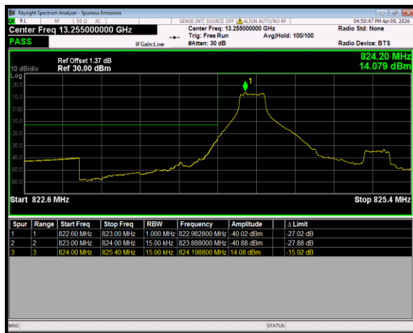
Band26(824-849) QPSK BW=1.4MHz LowChannel=26797 RB Size=1 Position=#0
