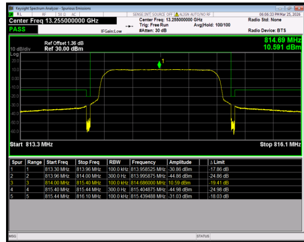
Band26(814-824) QPSK BW=1.4MHz LowChannel=26697 RB Size=6 Position=#0
