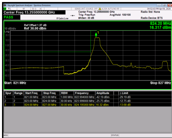
Band26(824-849) QPSK BW=3MHz LowChannel=26805 RB Size=1 Position=#0
