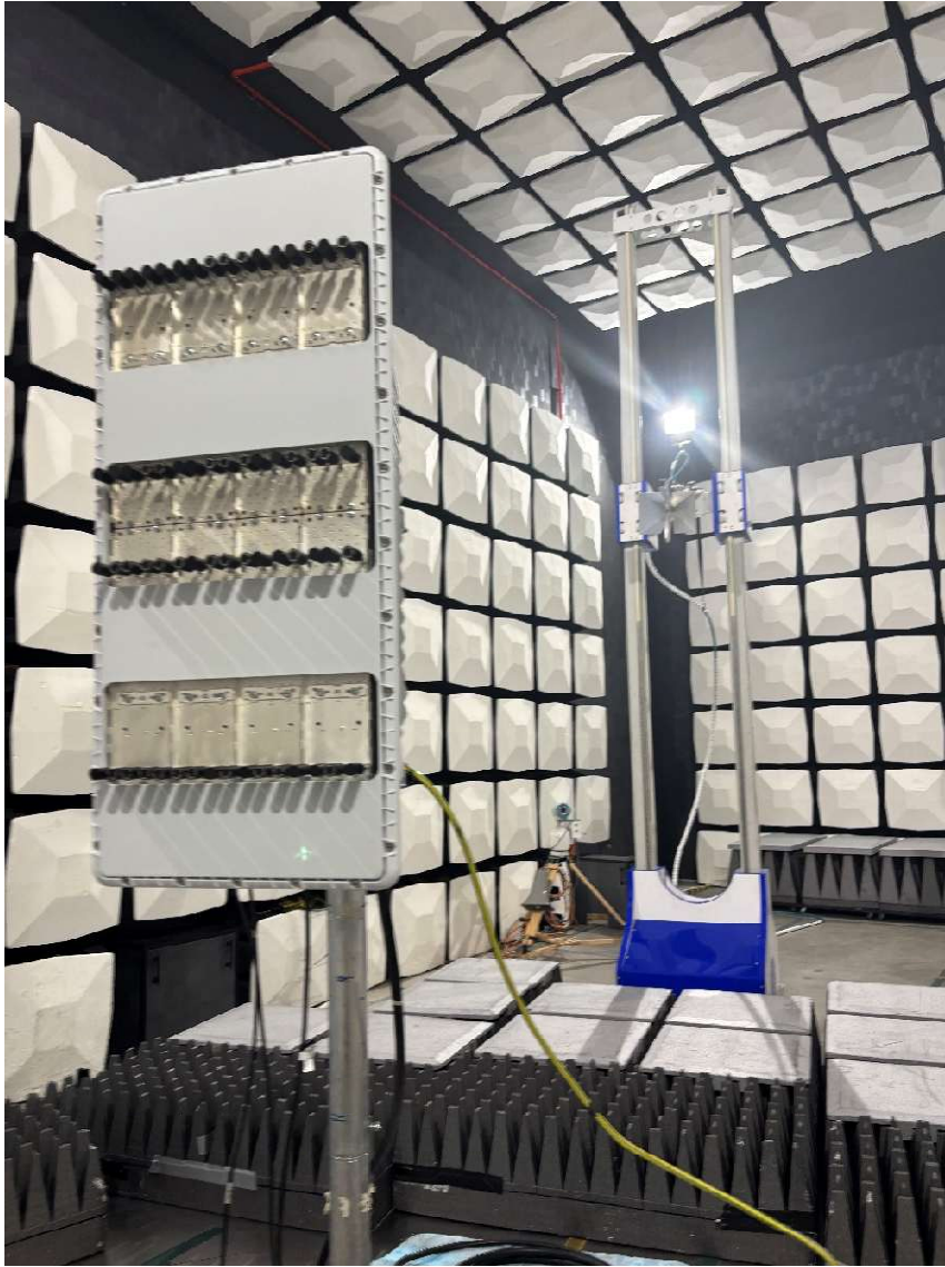
Photo of the test set-up for radiated emission 1 – 18 GHz
