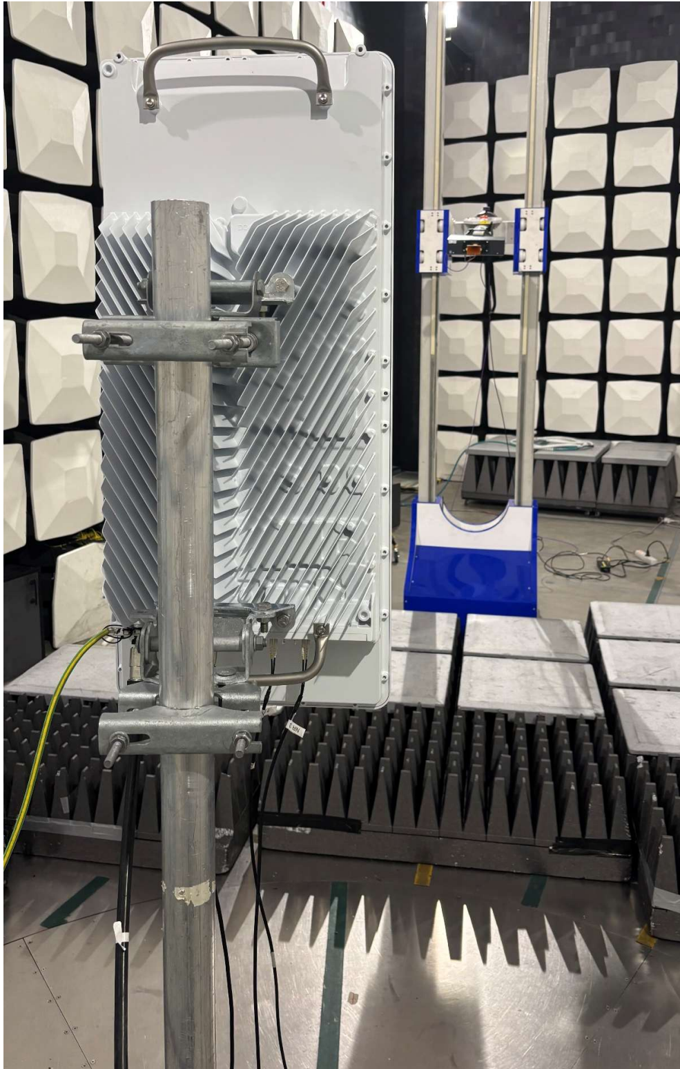
Photo of the test set-up for radiated emission 18 – 40 GHz
