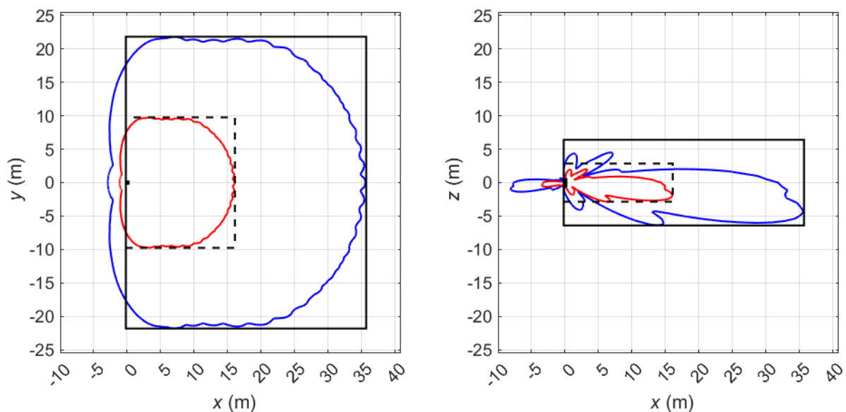
Figure 2 Compliance boundaries for general public exposure (black solid line) and occupational exposure (black dashed line) for the markets where the FCC limits apply. The blue solid lines correspond to compliance distance results for general public exposure obtained using the spherical models. The red solid lines indicate the corresponding compliance distance results for occupational exposure. The EUT is shown from above (left) and from the side (right) with its backplane located at x = 0 m. Mode: B25 (NR) + B66 (NR). Total time-averaged power delivered to the antenna: 59.1 dBm / 805.7 W. Electrical tilt: 7 degrees- Sector shape: Macro.
