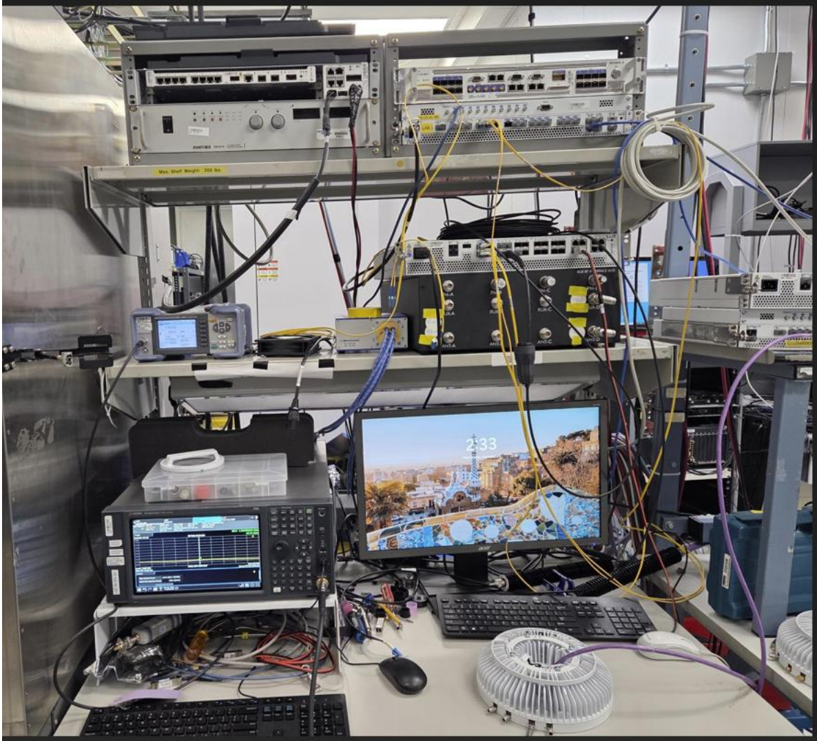
Figure 3.4-1: Set up photo for Conducted Radio Compliance Testing
