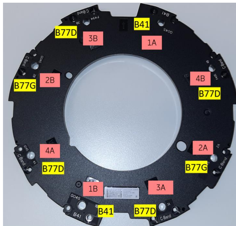
Figure C.2 Top view of the EUT without the radome with the active antenna elements labeled.
