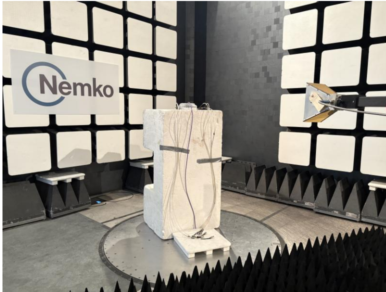
Figure 3.5-5: EUT Set-up photo for Radiated Emissions [1-6 GHz]
