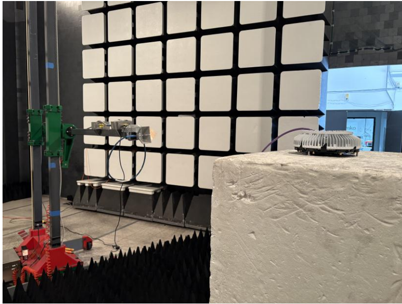
Figure 3.5-7: EUT Set-up photo for Radiated Emissions [18-40 GHz]
