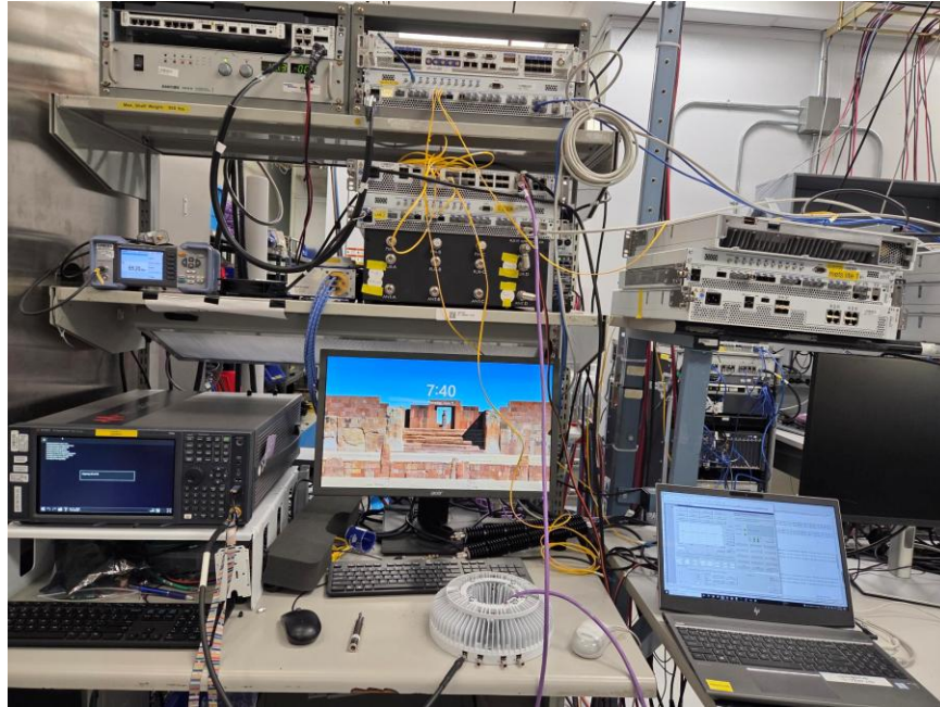
Figure 3.5-1: Set up photo for Conducted Radio Compliance Testing
