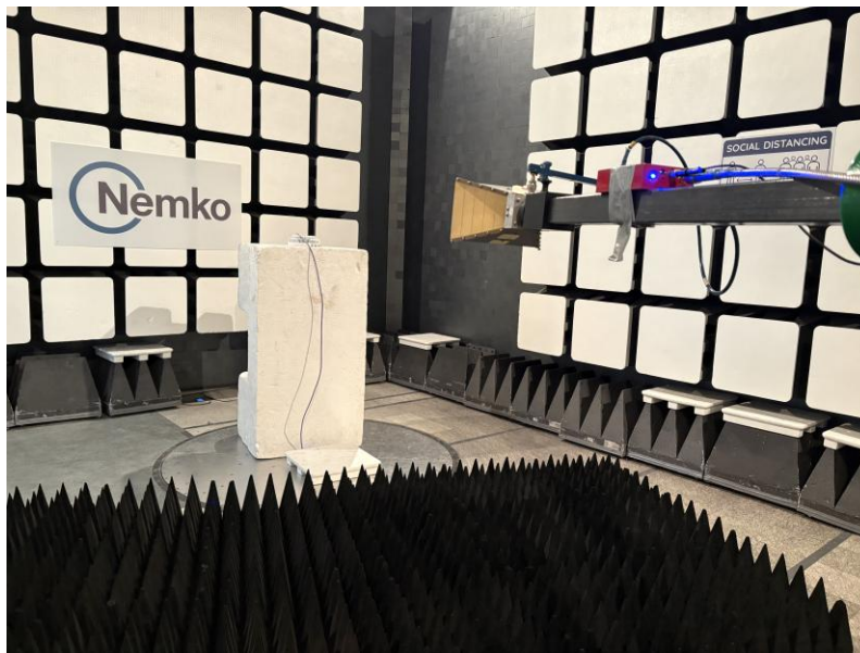
Figure 3.5-6: EUT Set-up photo for Radiated Emissions [6-18 GHz]
