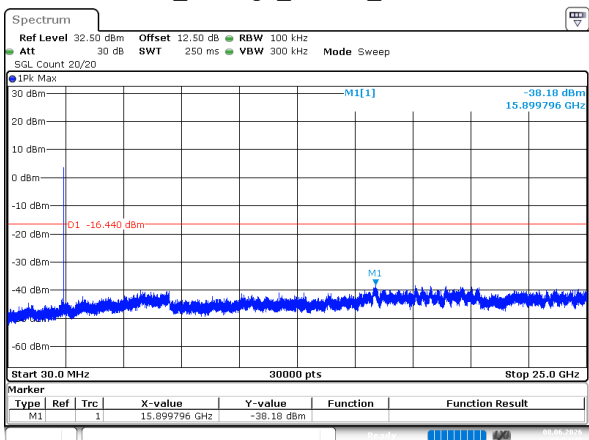
BLE_125kbps_Middle_Channel
