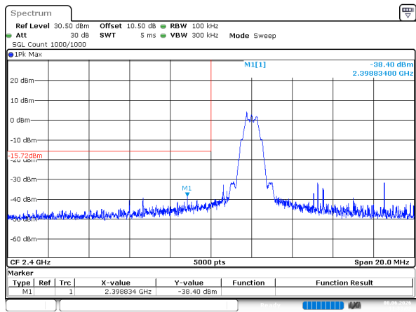
BLE_125kbps_Low_Channel
