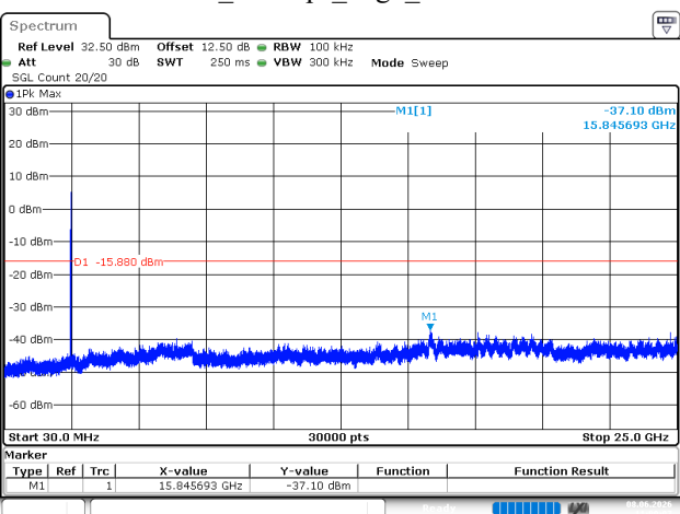
BLE_500kbps_High_Channel
