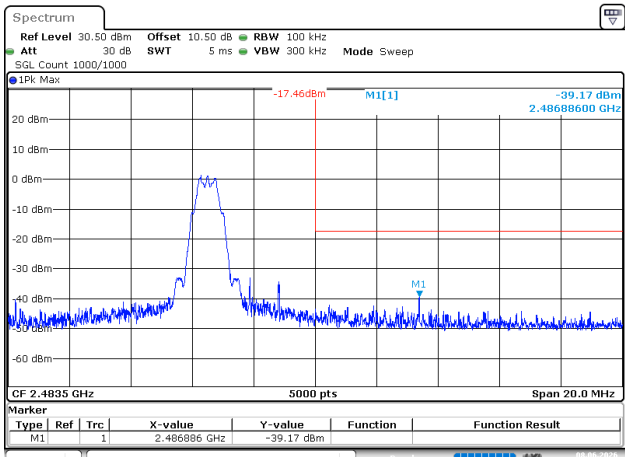
BLE_125kbps_High_Channel
