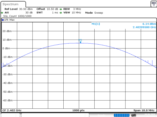
BLE_125kbps_Low_Channel
