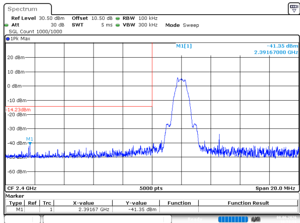
BLE_500kbps_Low_Channel
