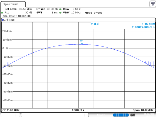
BLE_125kbps_High_Channel
