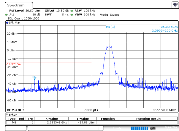
BLE_1M_Low_Channel
