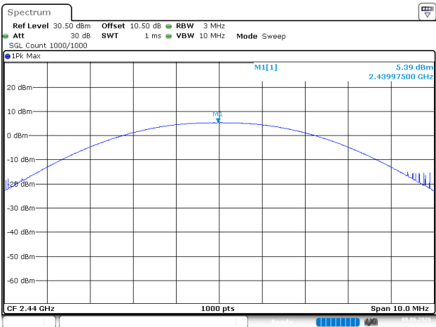
BLE_500kbps_Middle_Channel
