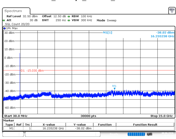
BLE_500kbps_Middle_Channel
