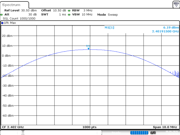
BLE_500kbps_Low_Channel
