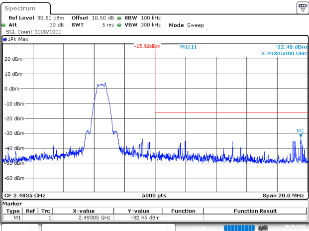
BLE_1M_High_Channel
