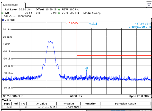
BLE_500kbps_High_Channel
