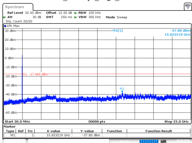
BLE_125kbps_High_Channel
