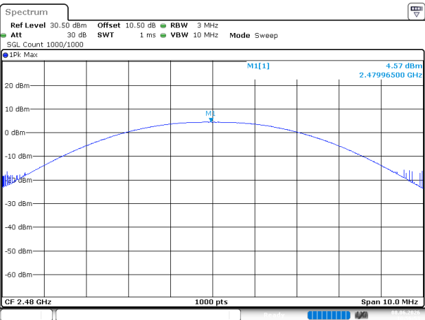
BLE_500kbps_High_Channel
