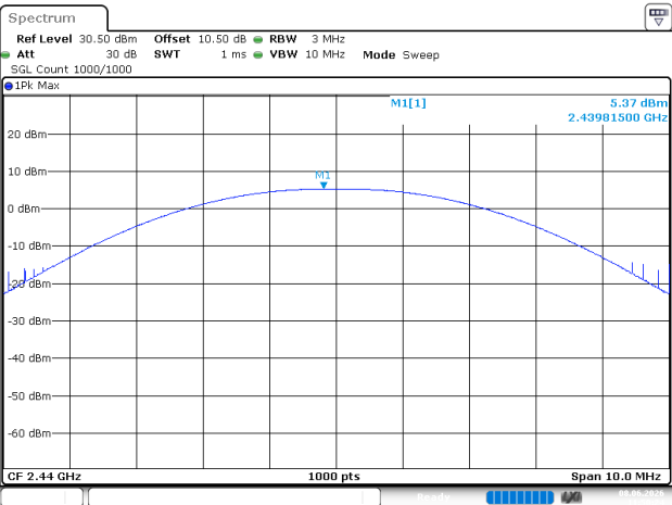
BLE_125kbps_Middle_Channel
