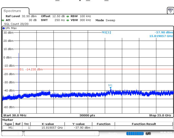
BLE_500kbps_Low_Channel
