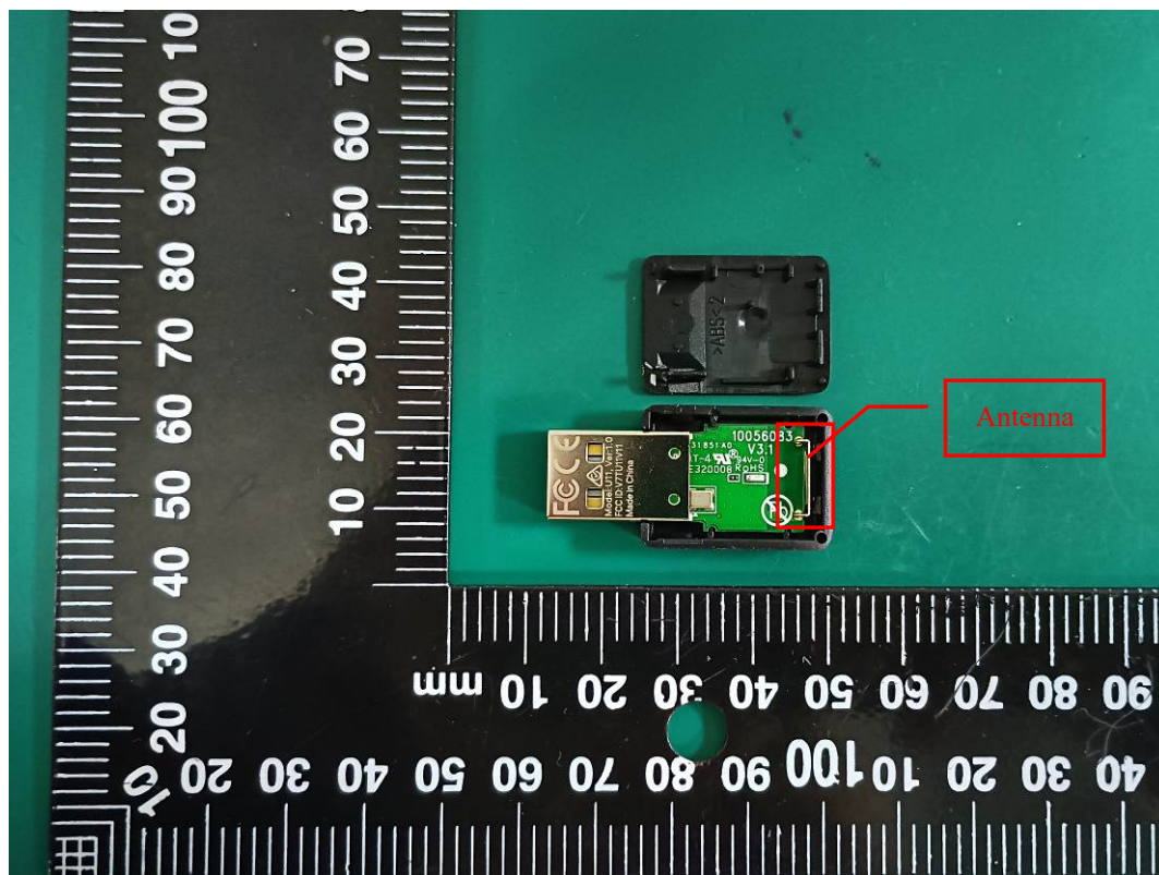
EUT Horizontal-UP View
