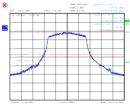
802.11ax20_5240MHz_RU_Full_Chain 0
