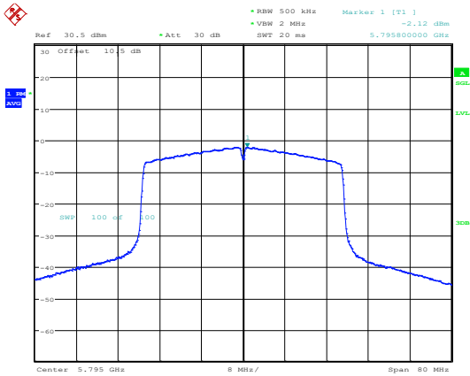
802.11ax40_5795MHz_RU_Full_Chain 0
