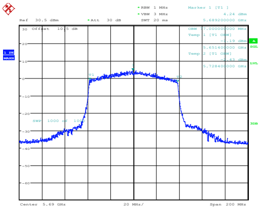
802.11ax80_5690MHz_RU_Full_Chain 0
