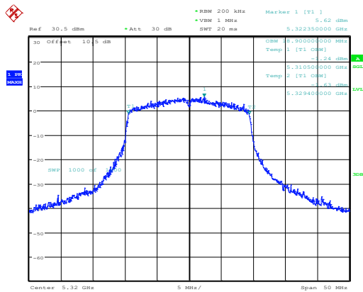
802.11ax20_5320MHz_RU_Full_Chain 0
