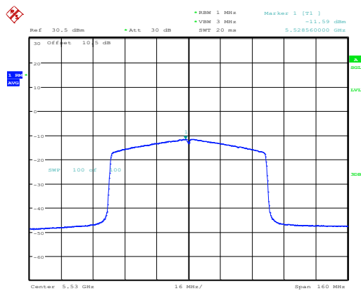
802.11ax80_5530MHz_RU_Full_Chain 1
