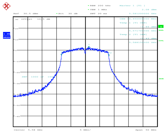
802.11a_5580MHz_Chain 0
