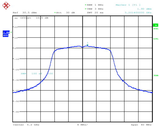
802.11a_5200MHz_Chain 1
