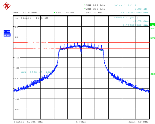
802.11a_5785MHz_Chain 0
