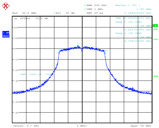
802.11a_5700MHz_Chain 0
