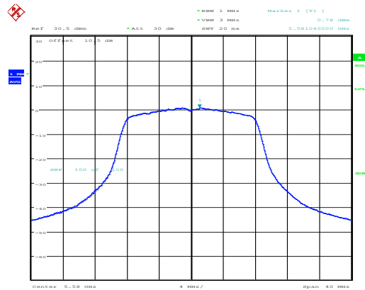
802.11a_5580MHz_Chain 0
