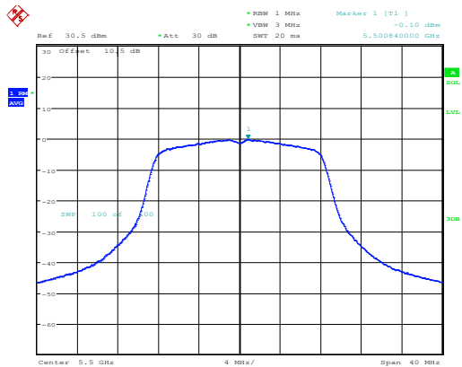
802.11a_5500MHz_Chain 0
