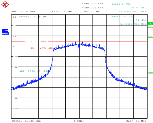
802.11ax20_5745MHz_RU_Full_Chain 0
