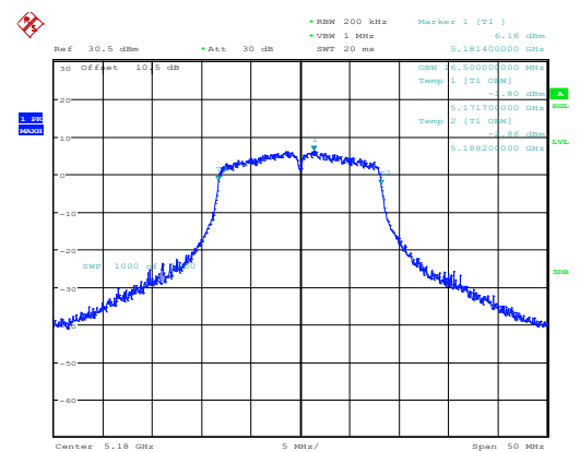
802.11a_5180MHz_Chain 0
