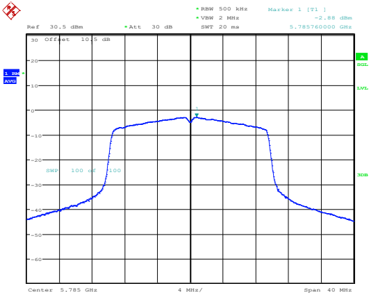
802.11ax20_5785MHz_RU_Full_Chain 1
