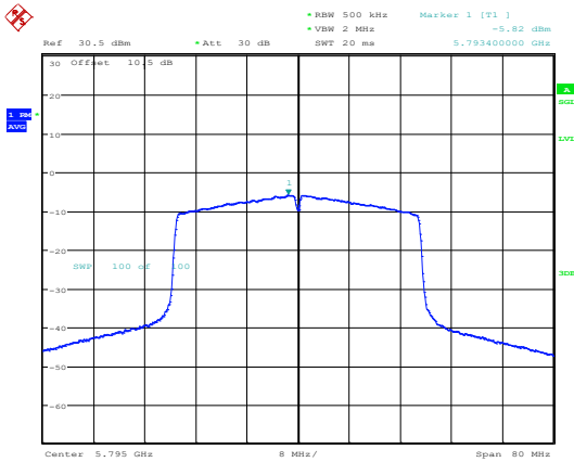
802.11ax40_5795MHz_RU_Full_Chain 1
