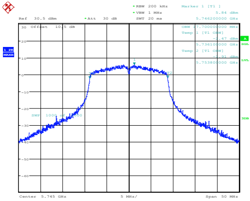
802.11ac20_5745MHz_Chain 0
