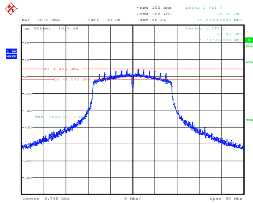
802.11ac20_5745MHz_Chain 0
