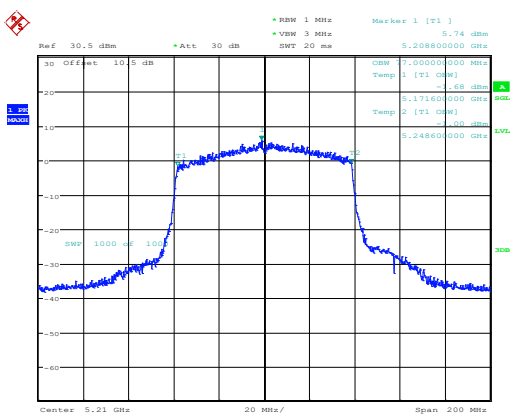
802.11ax80_5210MHz_RU_Full_Chain 0
