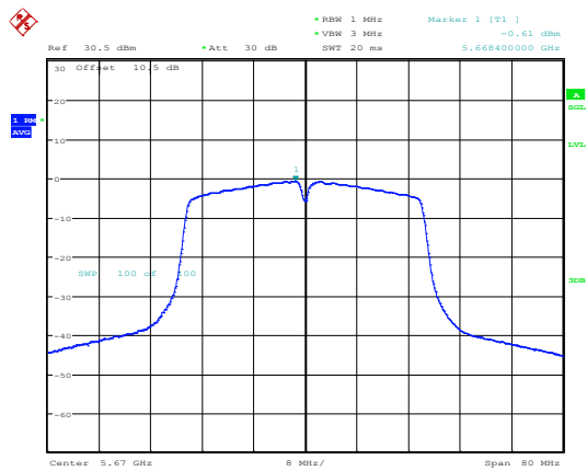
802.11ac40_5670MHz_Chain 0
