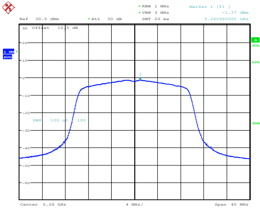
802.11ax20_5260MHz_RU_Full_Chain 1
