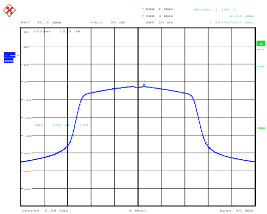
802.11ax20_5580MHz_RU_Full_Chain 1
