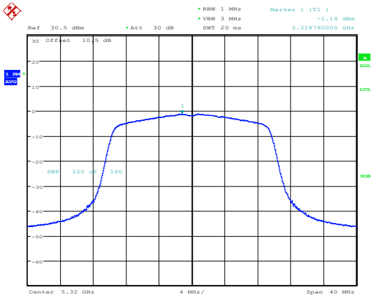
802.11ax20_5320MHz_RU_Full_Chain 1
