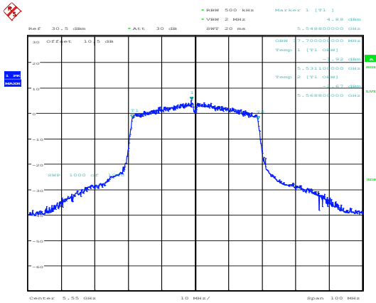
802.11ax40_5550MHz_RU_Full_Chain 0
