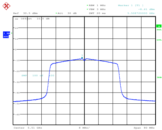
802.11ax40_5510MHz_RU_Full_Chain 1
