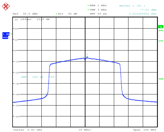
802.11ax80_5610MHz_RU_Full_Chain 0
