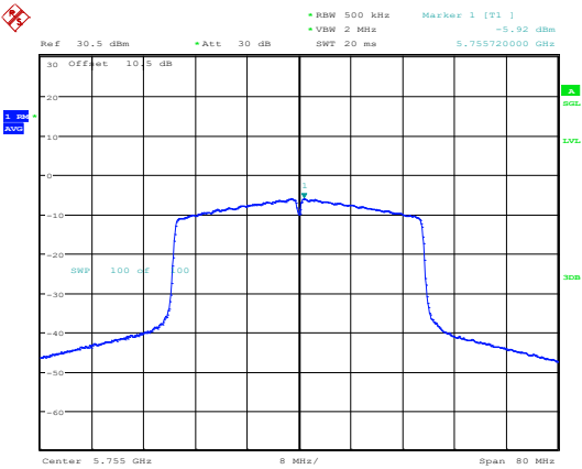
802.11ax40_5755MHz_RU_Full_Chain 1
