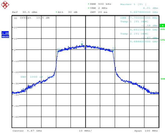
802.11ax40_5670MHz_RU_Full_Chain 0
