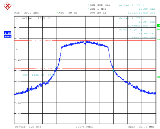
802.11ax20_5500MHz_RU_Full_Chain 0
