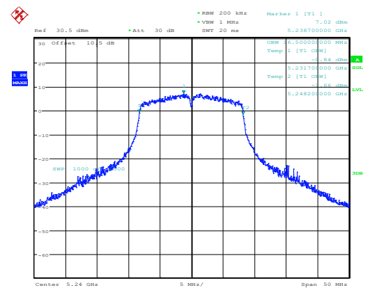
802.11a_5240MHz_Chain 0
