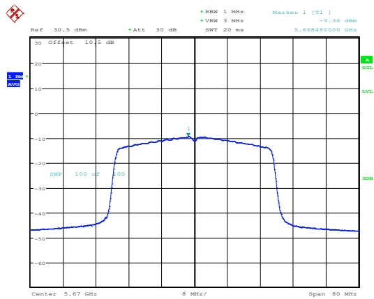
802.11ax40_5670MHz_RU_Full_Chain 1
