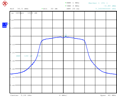
802.11a_5260MHz_Chain 1
