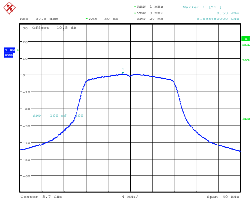
802.11a_5700MHz_Chain 0
