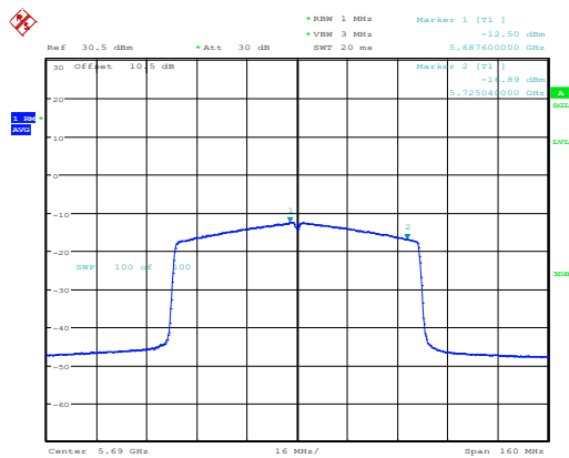
802.11ax80_5690MHz_RU_Full_Chain 1
