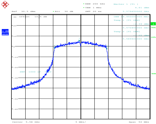
802.11ax20_5580MHz_RU_Full_Chain 0
