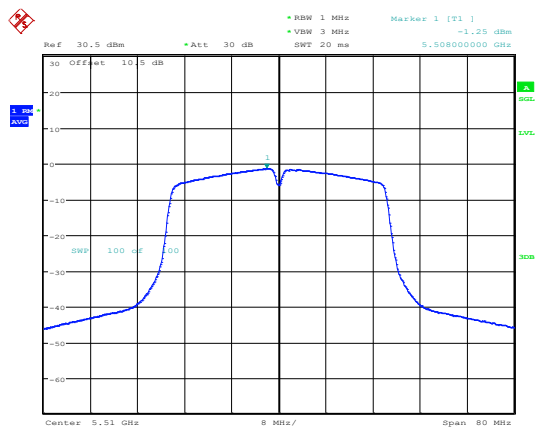
802.11ac40_5510MHz_Chain 0
