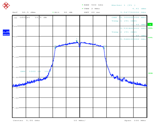
802.11ac40_5550MHz_Chain 0
