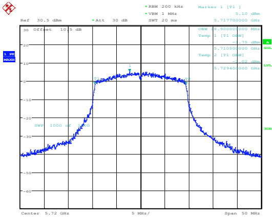
802.11ax20_5720MHz_RU_Full_Chain 0
