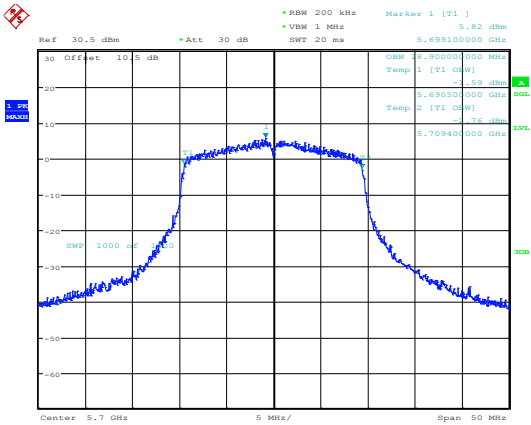
802.11ax20_5700MHz_RU_Full_Chain 0
