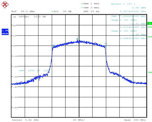
802.11ax80_5610MHz_RU_Full_Chain 0
