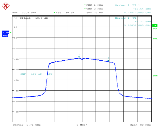
802.11ax40_5710MHz_RU_Full_Chain 1
