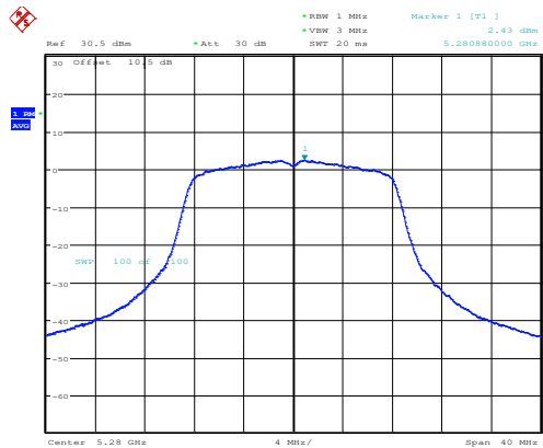
802.11a_5280MHz_Chain 0
