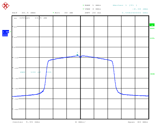
802.11ax40_5550MHz_RU_Full_Chain 1
