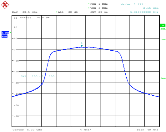
802.11ax20_5320MHz_RU_Full_Chain 0
