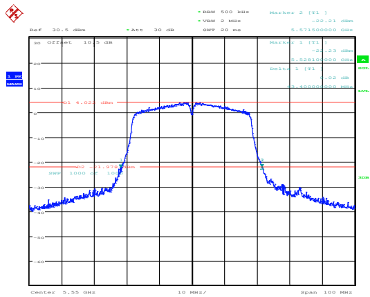
802.11ac40_5550MHz_Chain 0
