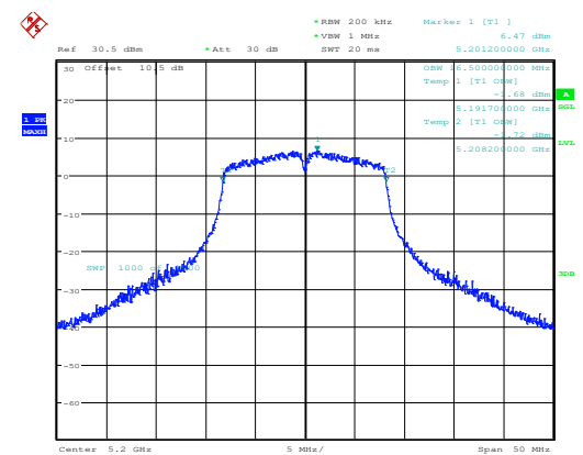
802.11a_5200MHz_Chain 0
