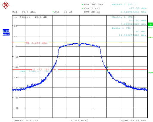
802.11a_5500MHz_Chain 0
