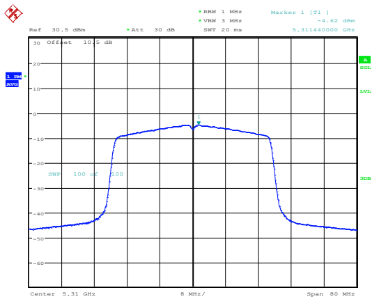
802.11ax40_5310MHz_RU_Full_Chain 1
