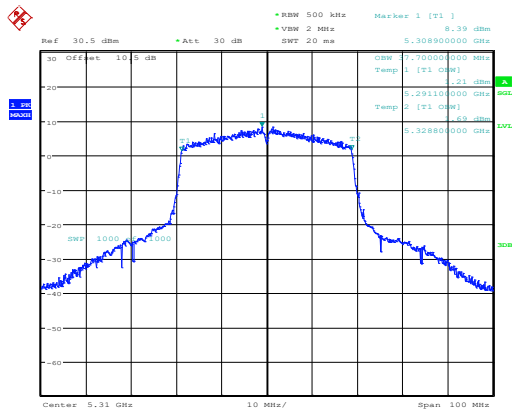
802.11ax40_5310MHz_RU_Full_Chain 0
