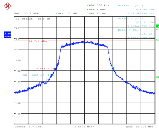
802.11ax20_5700MHz_RU_Full_Chain 0
