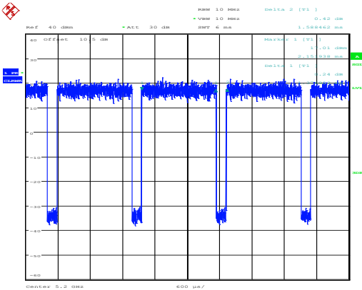
802.11a_5200MHz_Chain 0
