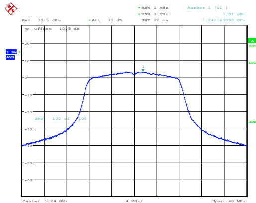
802.11a_5240MHz_Chain 1
