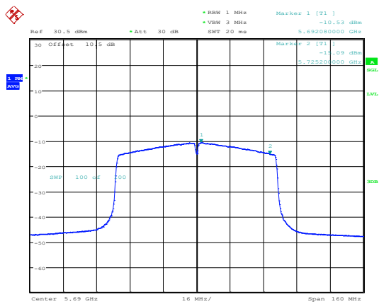
802.11ac80_5690MHz_Chain 1
