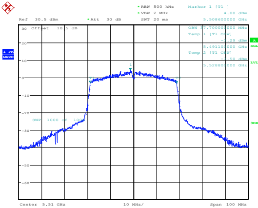
802.11ax40_5510MHz_RU_Full_Chain 0
