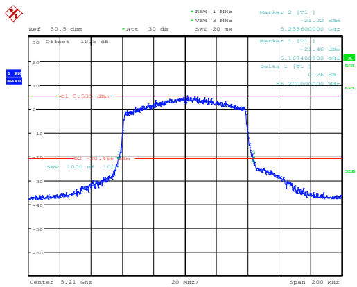
802.11ax80_5210MHz_RU_Full_Chain 0
