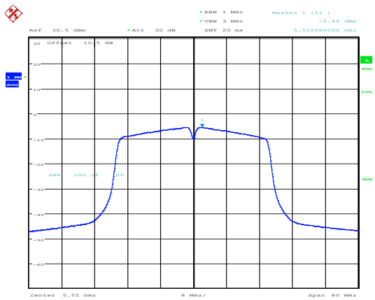
802.11ac40_5550MHz_Chain 1
