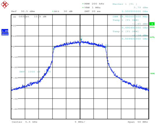
802.11ax20_5500MHz_RU_Full_Chain 0
