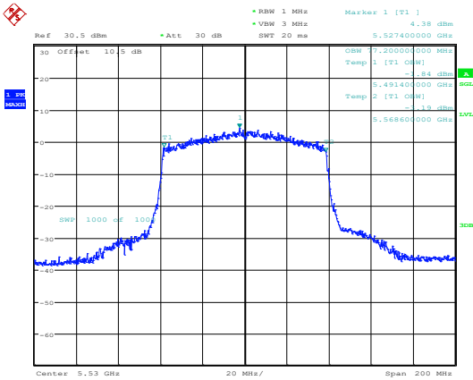
802.11ax80_5530MHz_RU_Full_Chain 0
