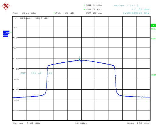
802.11ax80_5610MHz_RU_Full_Chain 1
