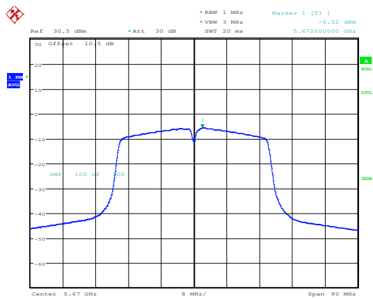
802.11ac40_5670MHz_Chain 1
