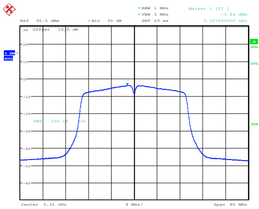
802.11ac40_5310MHz_Chain 1
