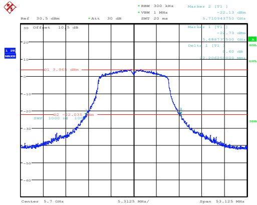
802.11a_5700MHz_Chain 0
