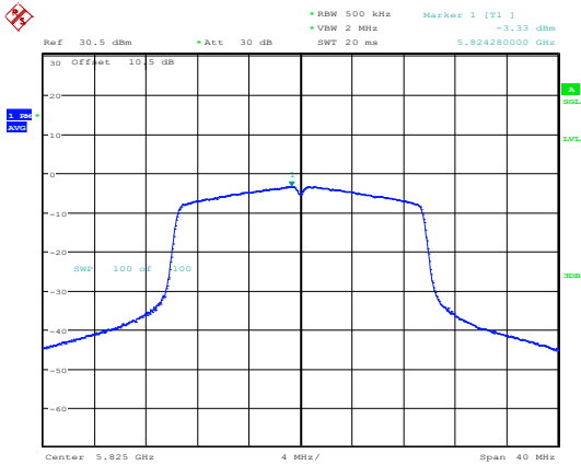
802.11ax20_5825MHz_RU_Full_Chain 1
