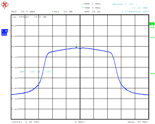
802.11ax20_5280MHz_RU_Full_Chain 1
