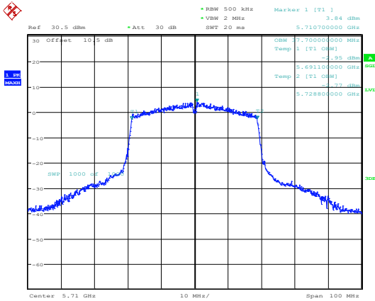
802.11ax40_5710MHz_RU_Full_Chain 0
