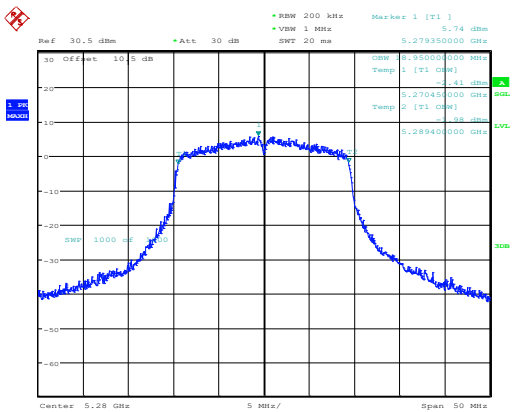
802.11ax20_5280MHz_RU_Full_Chain 0
