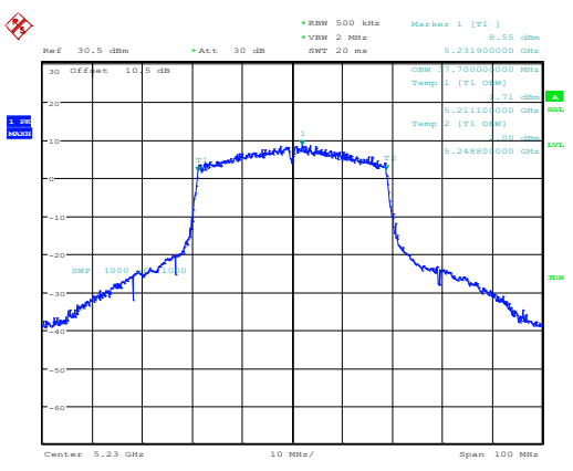
802.11ax40_5230MHz_RU_Full_Chain 0
