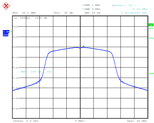
802.11ax20_5500MHz_RU_Full_Chain 1
