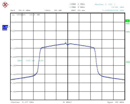
802.11ax40_5270MHz_RU_Full_Chain 1
