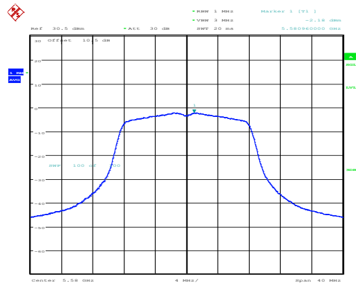
802.11a_5580MHz_Chain 1
