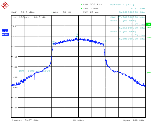
802.11ax40_5270MHz_RU_Full_Chain 0
