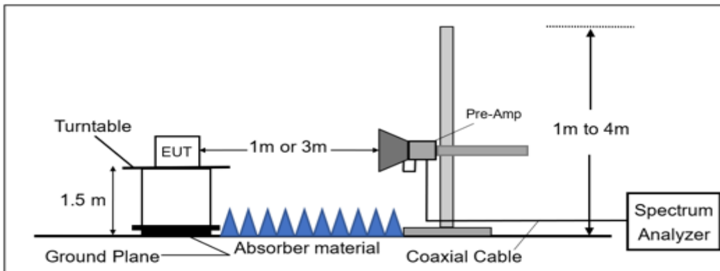
Radiated Emission Test Set-Up, Frequency Above 1GHz.
