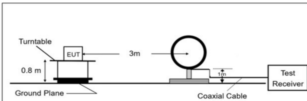
Radiated Emission Test Set-Up, Frequency Below 30MHz.
