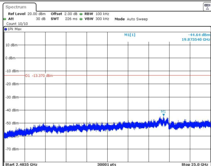
BLE_1M_Ant1_2402_2483.5~25000
