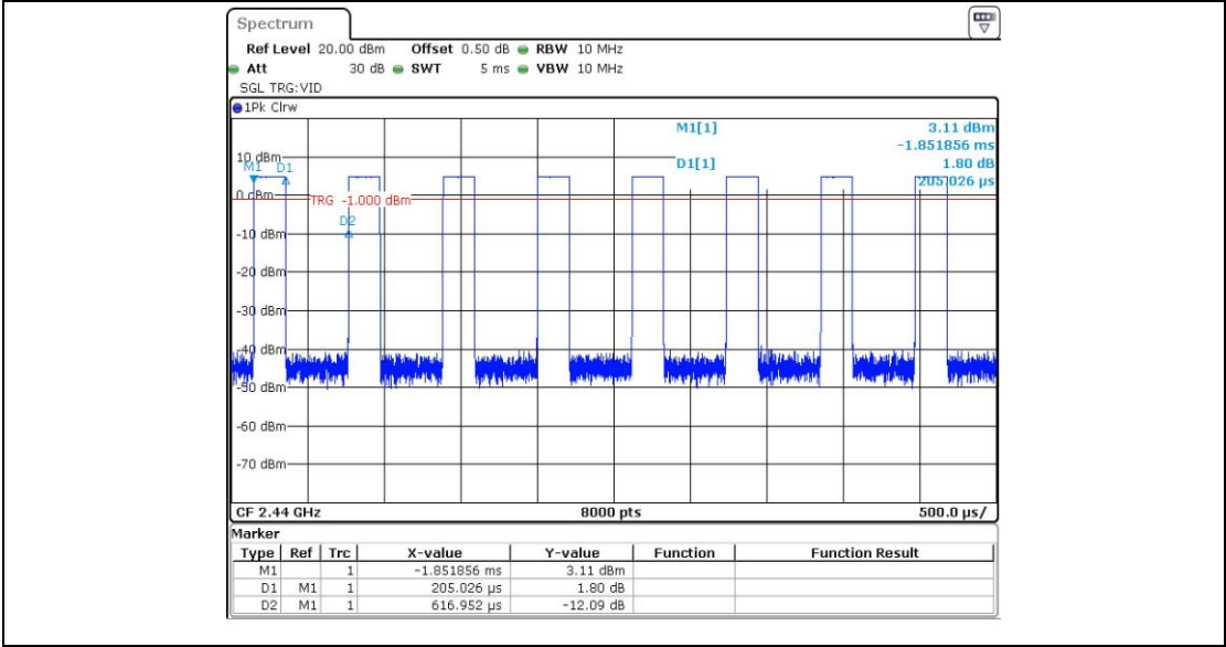
BLE_1M_Ant1_2440
