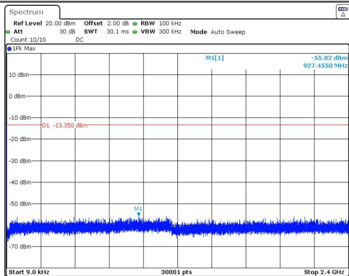
BLE_1M_Ant1_2440_0~Reference
