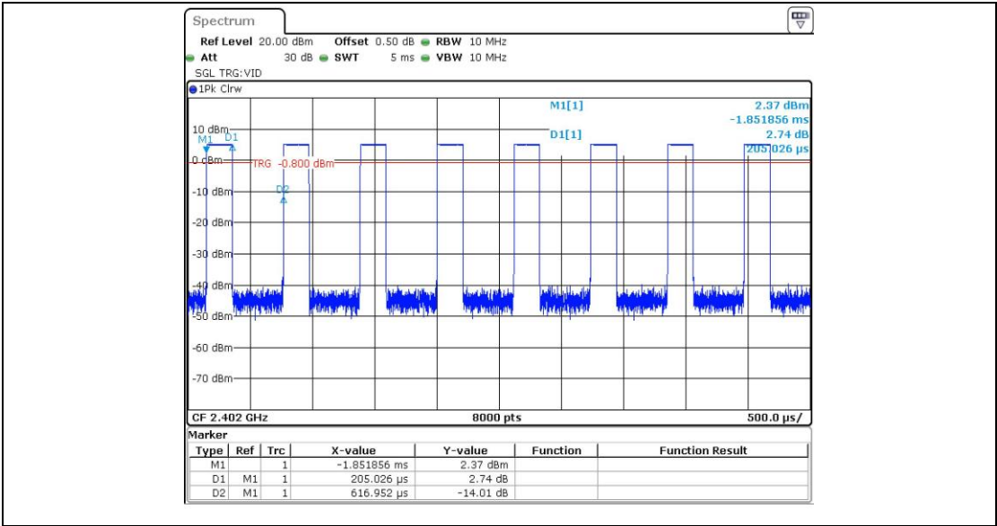
BLE_1M_Ant1_2402
