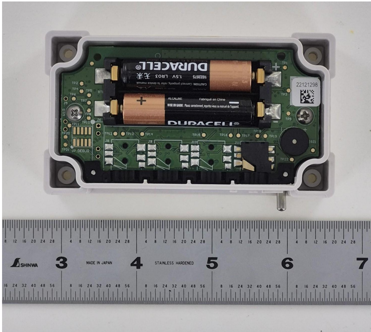
MX1104 PCB Back In Housing
