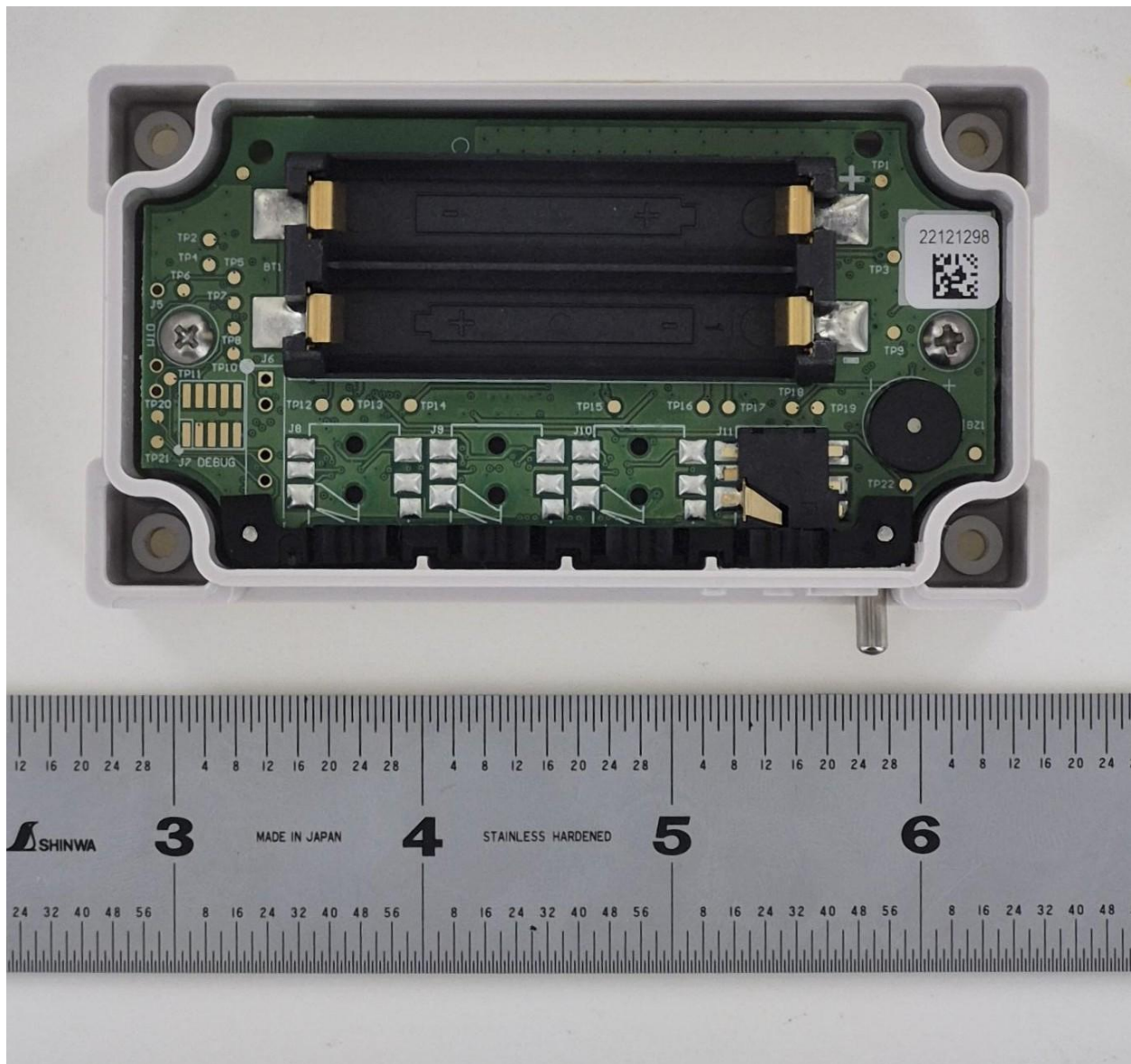
MX1104 PCB Back In Housing No Batteries
