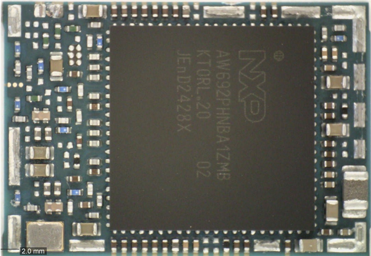
JODY-W662-01A_internal photo.jpg
