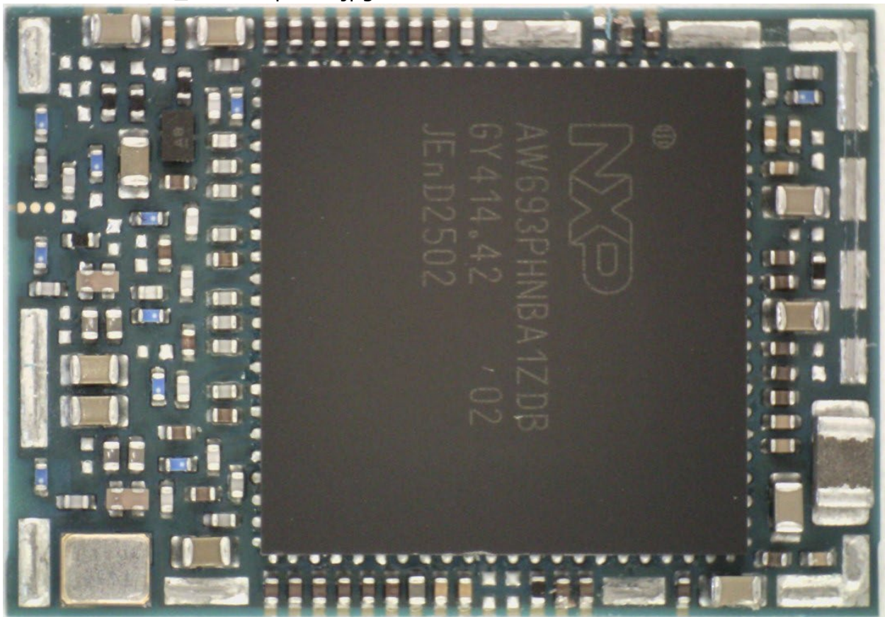
JODY-W683-21A_internal photo.jpg
