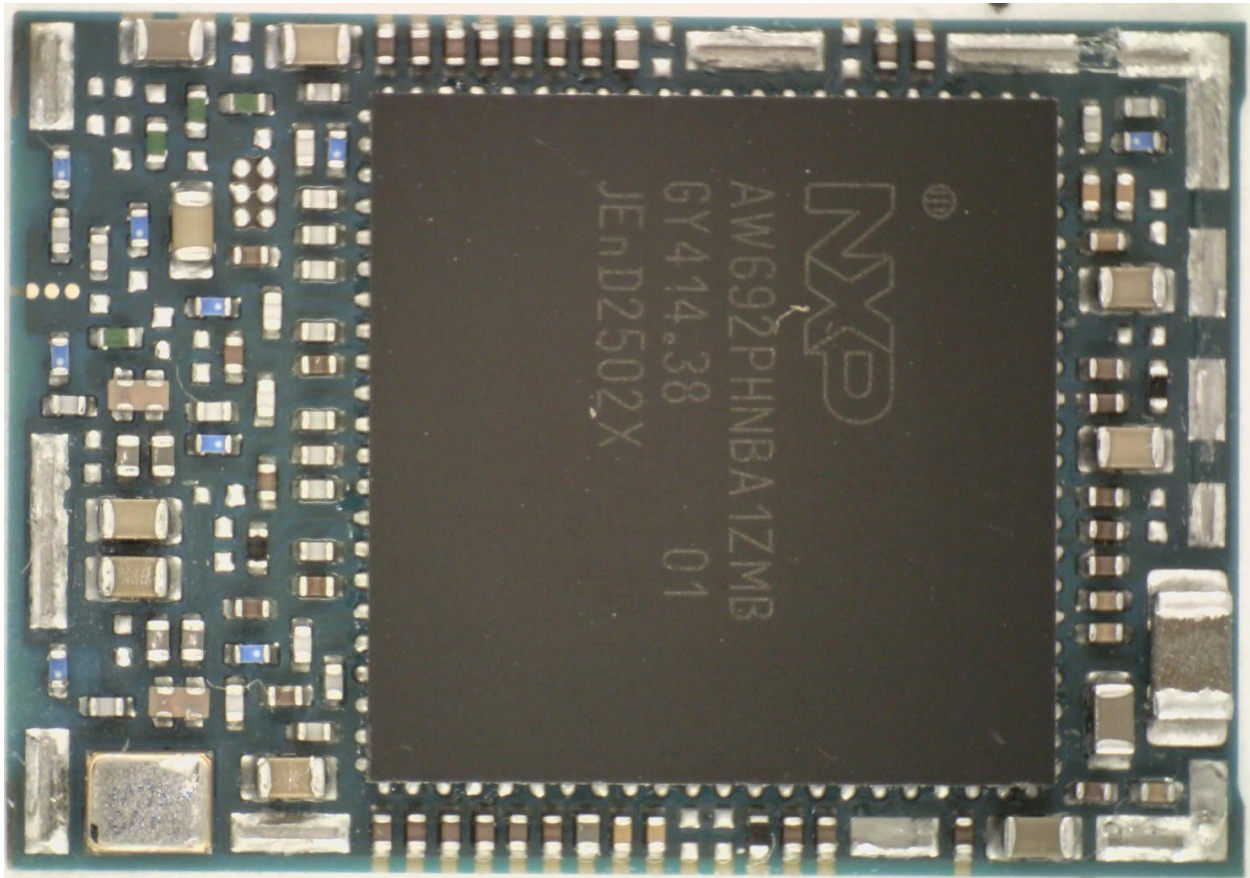
JODY-W663-01A_internal photo.jpg
