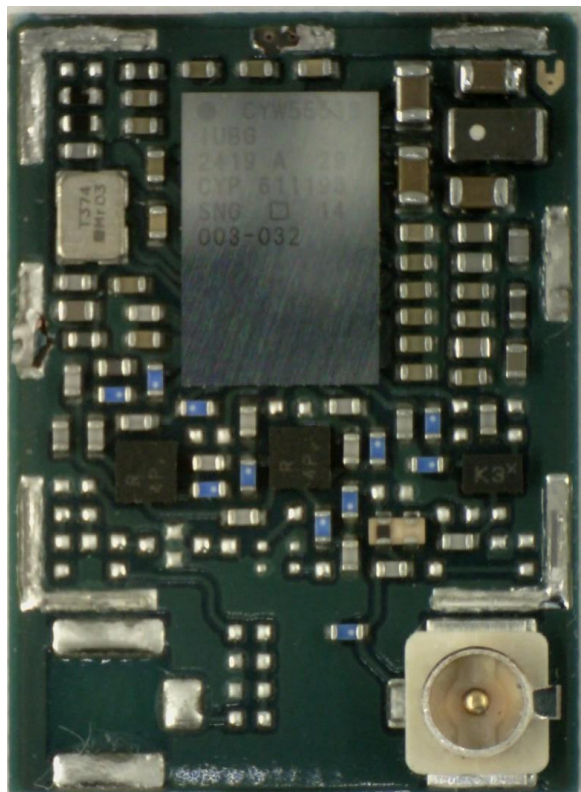
Figure 1: MAYA-W382-00B internal photo
