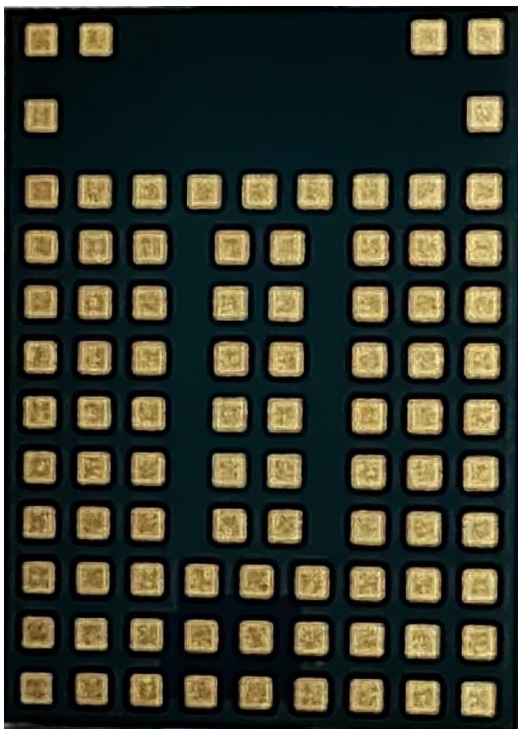
Figure 2: Bottom view of MAYA-W332-00B
