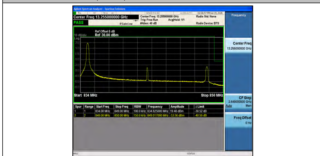
26(824-849)-15MHz-16QAM-26965-1RB#0-PASS
