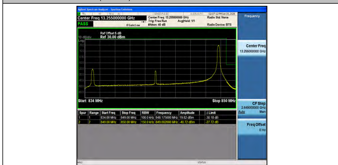
26(824-849)-15MHz-QPSK-26965-1RB#74-PASS
