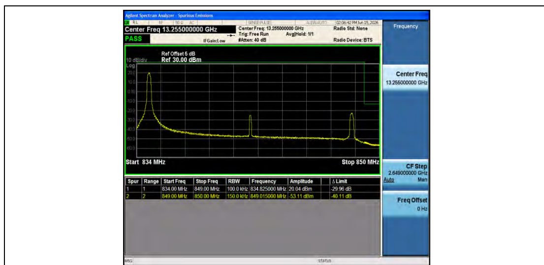
26(824-849)-15MHz-QPSK-26965-1RB#0-PASS
