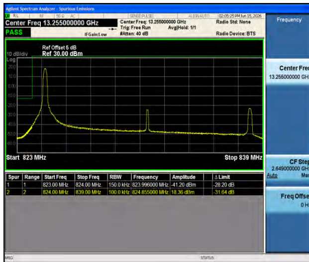
26(824-849)-15MHz-16QAM-26865-1RB#0-PASS
