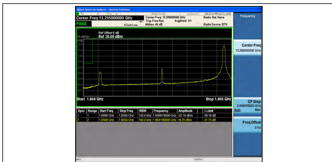
Band2-15MHz-16QAM-18675-1RB#74-PASS
