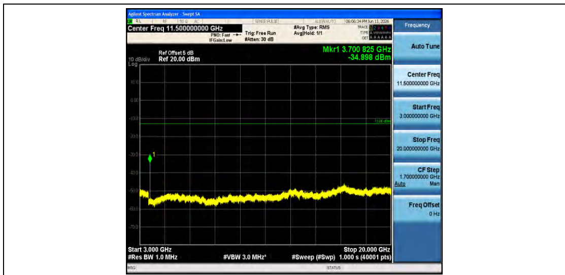
Band2-1.4MHz-16QAM-18607-1RB#0-3000~20000-PASS
