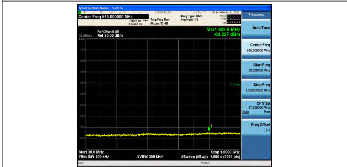
Band2-5MHz-QPSK-18625-1RB#0-30~1000-PASS
