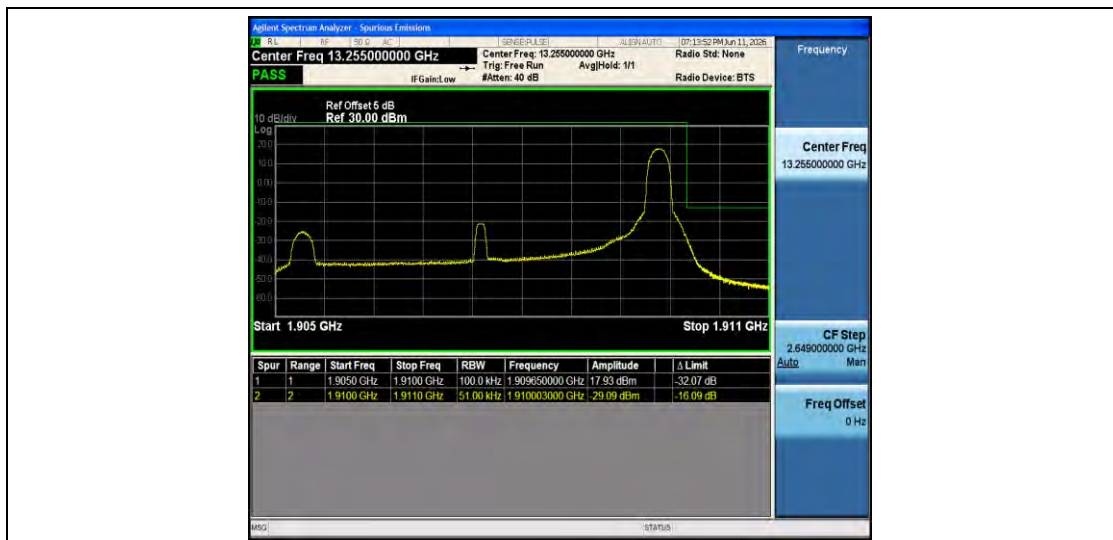
Band2-5MHz-16QAM-19175-1RB#24-PASS
