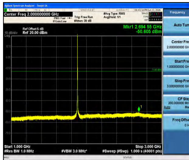
Band2-3MHz-16QAM-18900-1RB#0-1000~3000-PASS
