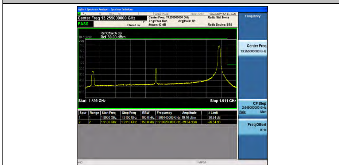
Band2-15MHz-QPSK-19125-1RB#74-PASS
