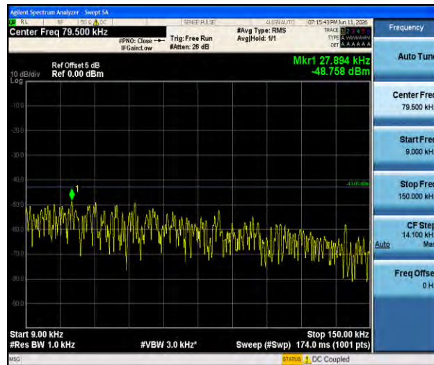
Band2-5MHz-16QAM-18625-1RB#0-0.009~0.15-PASS
