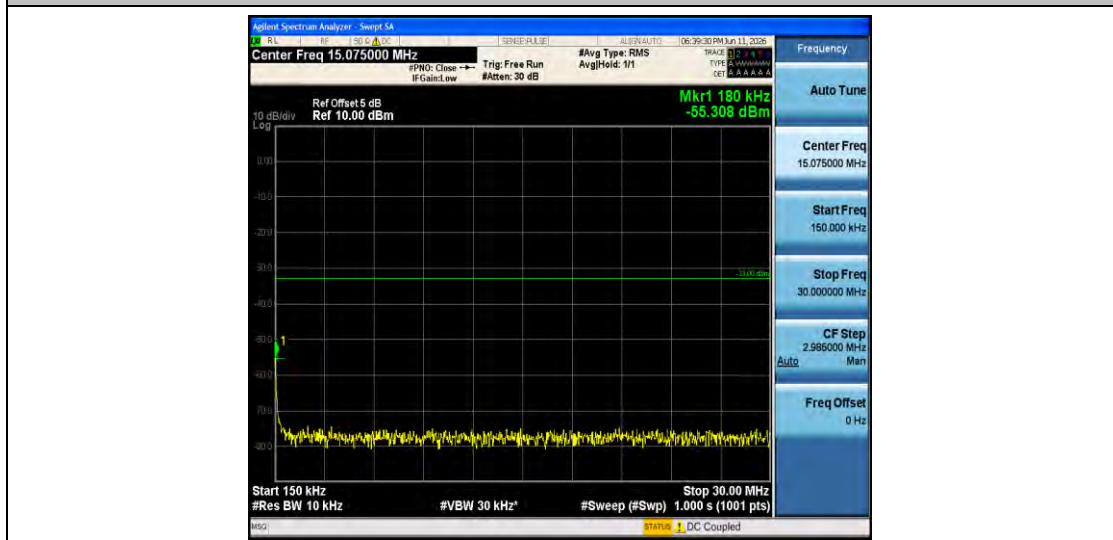
Band2-3MHz-QPSK-18615-1RB#0-0.15~30-PASS
