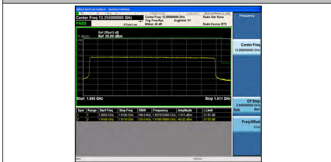
Band2-15MHz-16QAM-19125-75RB#0-PASS
