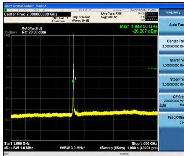
Band2-5MHz-16QAM-18625-1RB#0-1000~3000-PASS
