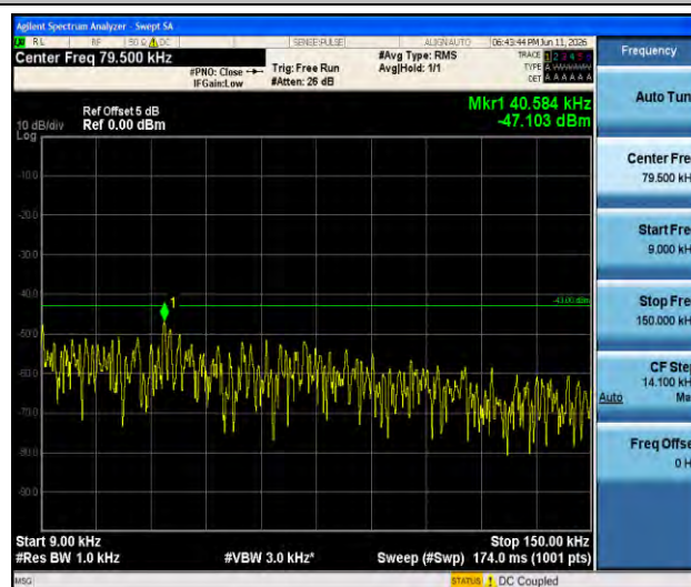
Band2-3MHz-QPSK-19185-1RB#0-0.009~0.15-PASS
