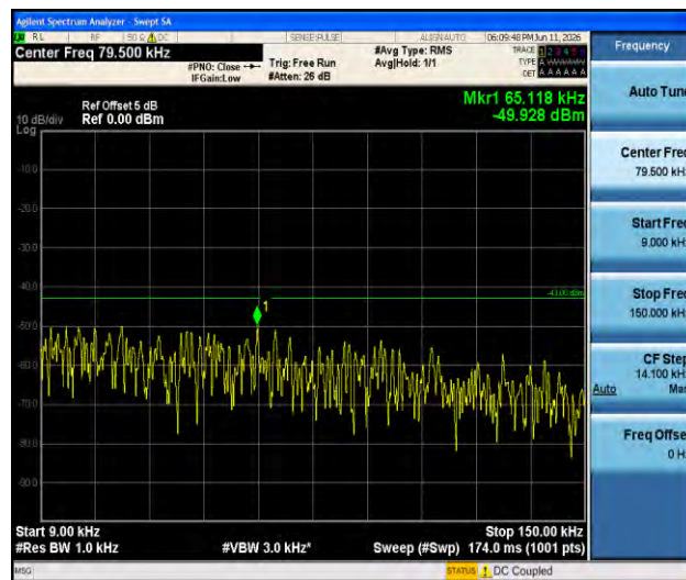
Band2-1.4MHz-16QAM-19193-1RB#0-0.009~0.15-PASS
