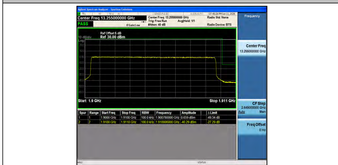
Band2-10MHz-QPSK-19150-50RB#0-PASS
