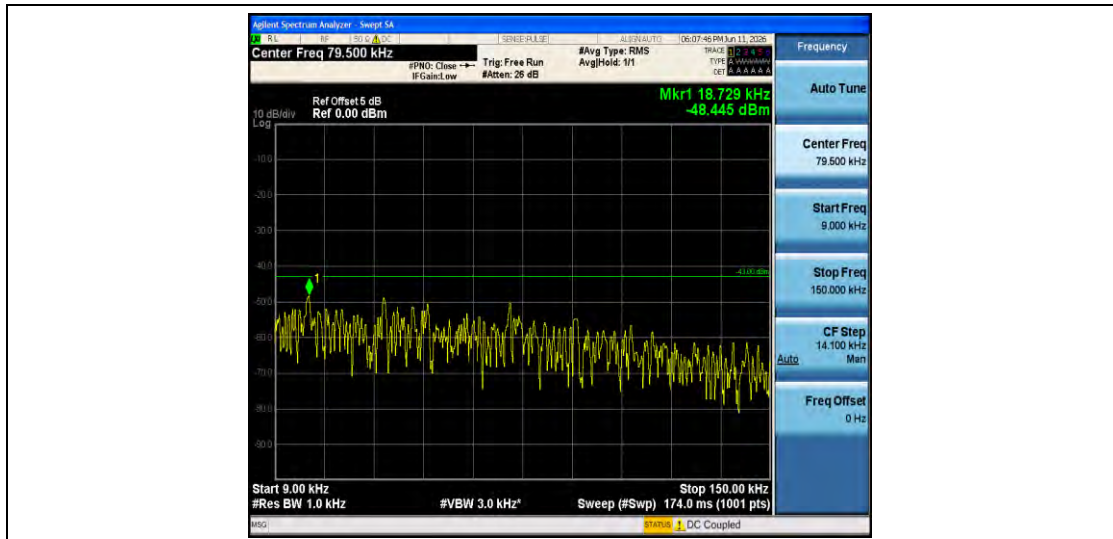
Band2-1.4MHz-16QAM-18900-1RB#0-0.009~0.15-PASS
