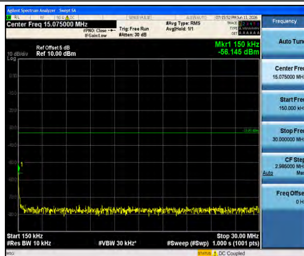
Band2-5MHz-16QAM-18625-1RB#0-0.15~30-PASS
