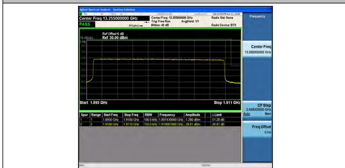
Band2-15MHz-QPSK-19125-75RB#0-PASS
