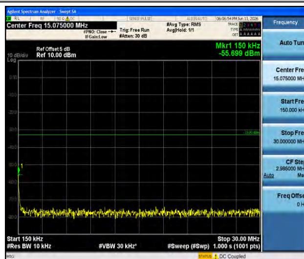
Band2-1.4MHz-QPSK-18900-1RB#0-0.15~30-PASS
