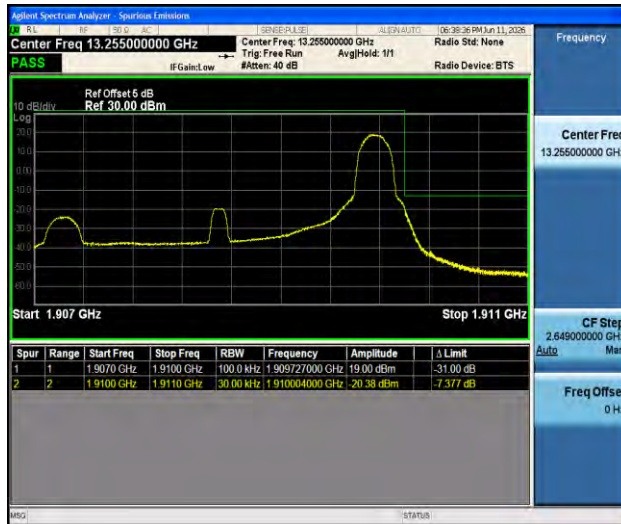
Band2-3MHz-16QAM-19185-1RB#14-PASS
