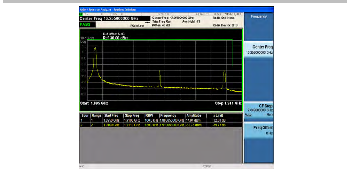
Band2-15MHz-16QAM-19125-1RB#0-PASS
