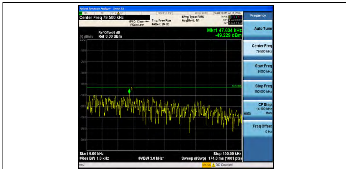
Band2-1.4MHz-QPSK-18607-1RB#0-0.009~0.15-PASS
