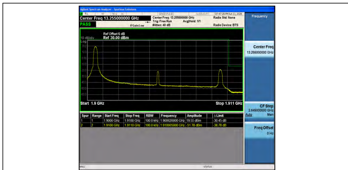
Band2-10MHz-QPSK-19150-1RB#0-PASS
