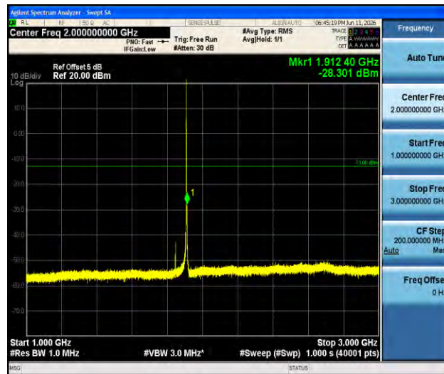
Band2-3MHz-16QAM-19185-1RB#0-1000~3000-PASS
