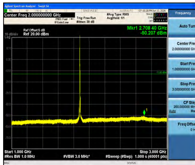
Band2-5MHz-16QAM-18900-1RB#0-1000~3000-PASS
