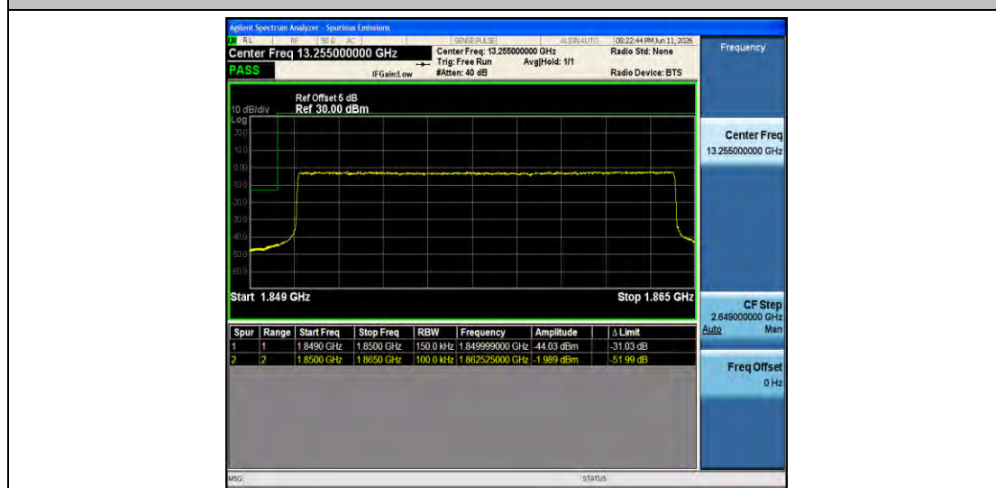
Band2-15MHz-16QAM-18675-75RB#0-PASS
