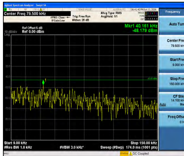
Band2-3MHz-QPSK-18900-1RB#0-0.009~0.15-PASS
