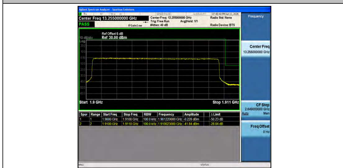
Band2-10MHz-16QAM-19150-50RB#0-PASS
