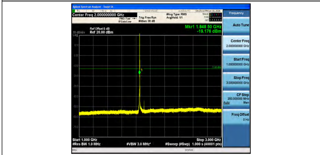
Band2-3MHz-16QAM-18615-1RB#0-1000~3000-PASS
