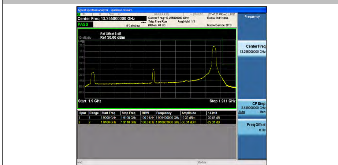
Band2-10MHz-QPSK-19150-1RB#49-PASS
