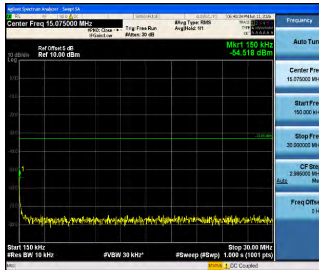
Band2-3MHz-16QAM-18615-1RB#0-0.15~30-PASS
