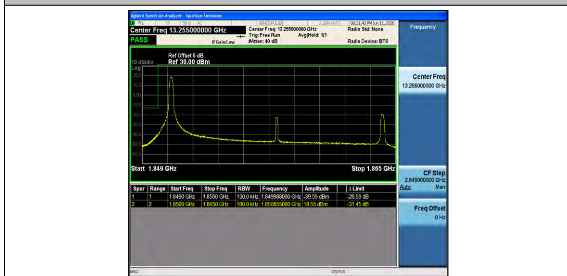
Band2-15MHz-16QAM-18675-1RB#0-PASS
