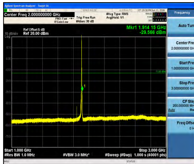
Band2-5MHz-QPSK-19175-1RB#0-1000~3000-PASS
