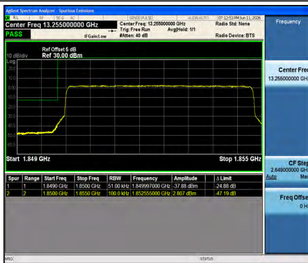
Band2-5MHz-16QAM-18625-25RB#0-PASS
