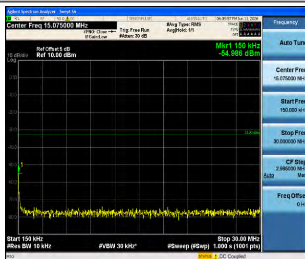
Band2-1.4MHz-16QAM-19193-1RB#0-0.15~30-PASS
