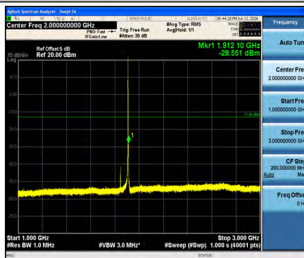
Band2-3MHz-QPSK-19185-1RB#0-1000~3000-PASS
