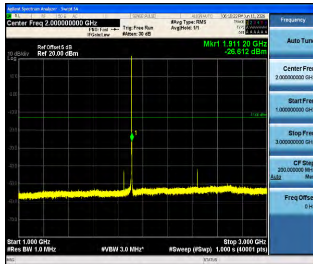
Band2-1.4MHz-16QAM-19193-1RB#0-1000~3000-PASS
