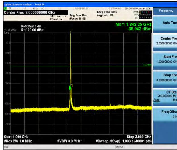
Band2-10MHz-16QAM-18650-1RB#0-1000~3000-PASS
