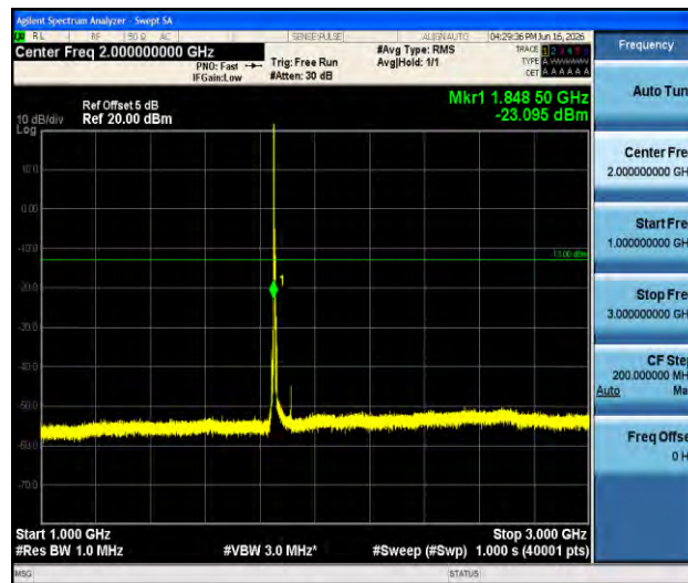
Band2-5MHz-QPSK-18625-1RB#0-1000~3000-PASS
