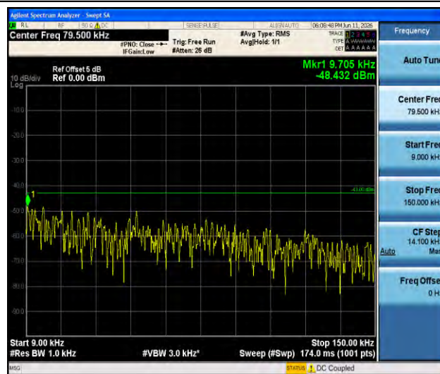
Band2-1.4MHz-QPSK-19193-1RB#0-0.009~0.15-PASS
