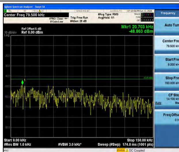
Band2-5MHz-16QAM-19175-1RB#0-0.009~0.15-PASS
