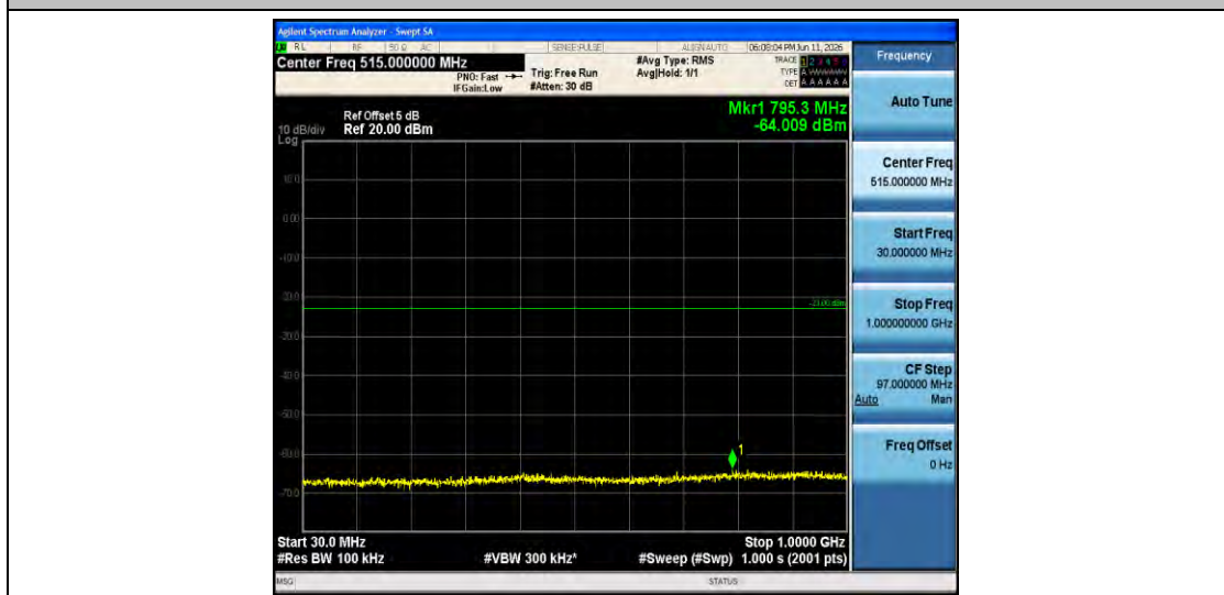
Band2-1.4MHz-16QAM-18900-1RB#0-30~1000-PASS
