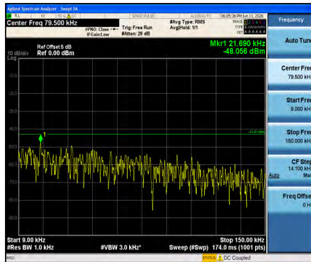
Band2-1.4MHz-16QAM-18607-1RB#0-0.009~0.15-PASS
