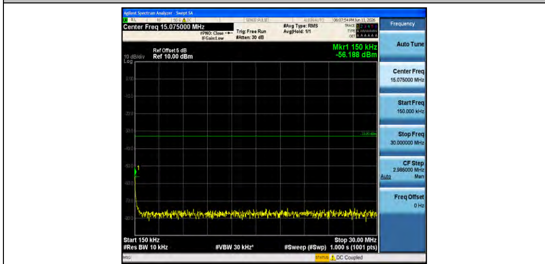
Band2-1.4MHz-16QAM-18900-1RB#0-0.15~30-PASS
