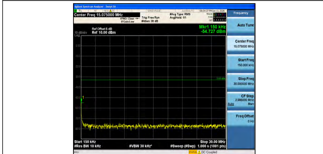
Band2-1.4MHz-QPSK-18607-1RB#0-0.15~30-PASS
