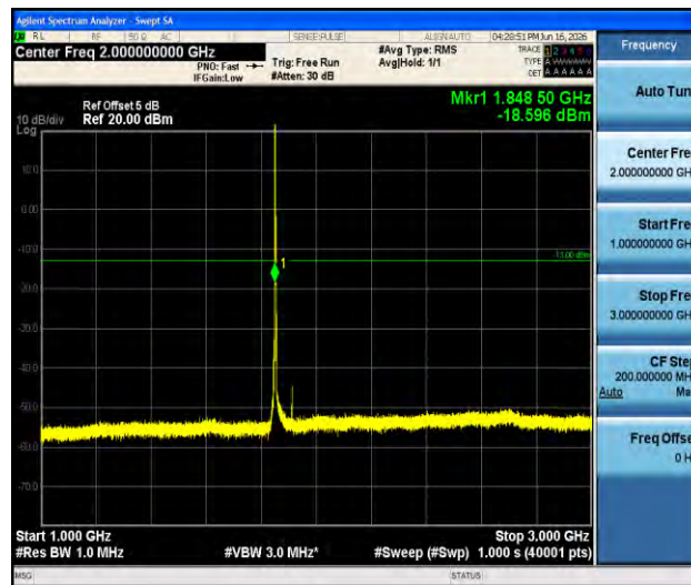
Band2-3MHz-QPSK-18615-1RB#0-1000~3000-PASS
