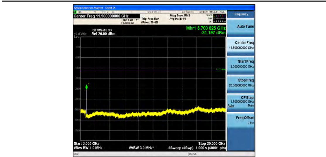
Band2-5MHz-16QAM-18625-1RB#0-3000~20000-PASS
