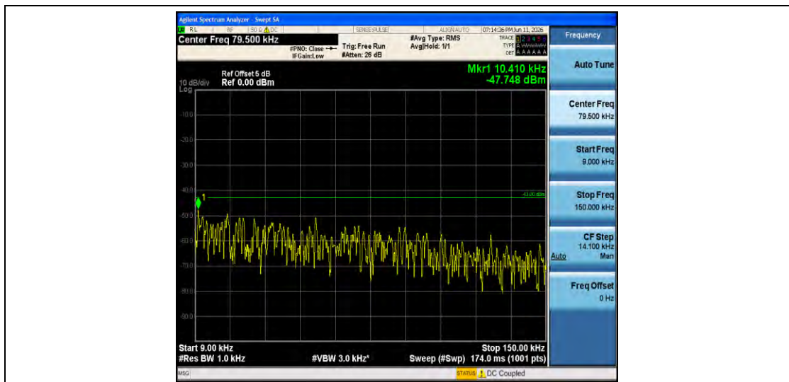
Band2-5MHz-QPSK-18625-1RB#0-0.009~0.15-PASS
