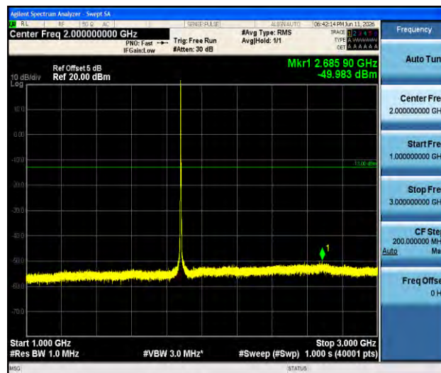
Band2-3MHz-QPSK-18900-1RB#0-1000~3000-PASS
