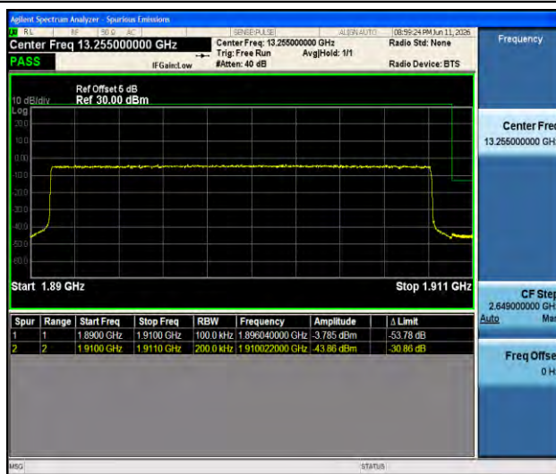
Band2-20MHz-16QAM-19100-100RB#0-PASS
