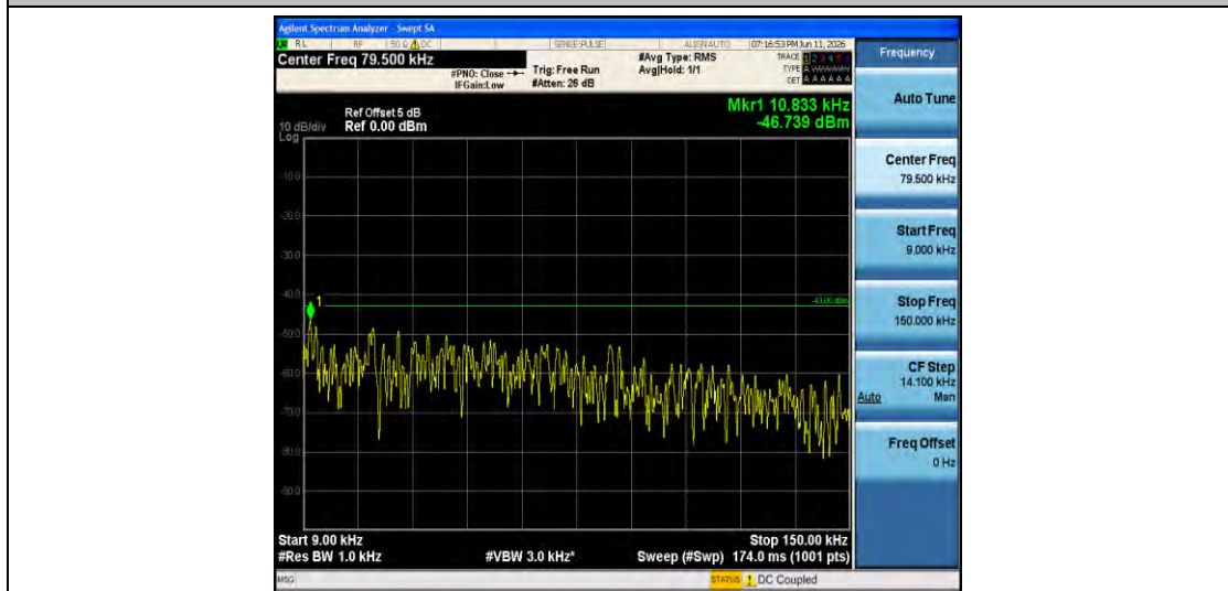
Band2-5MHz-QPSK-18900-1RB#0-0.009~0.15-PASS
