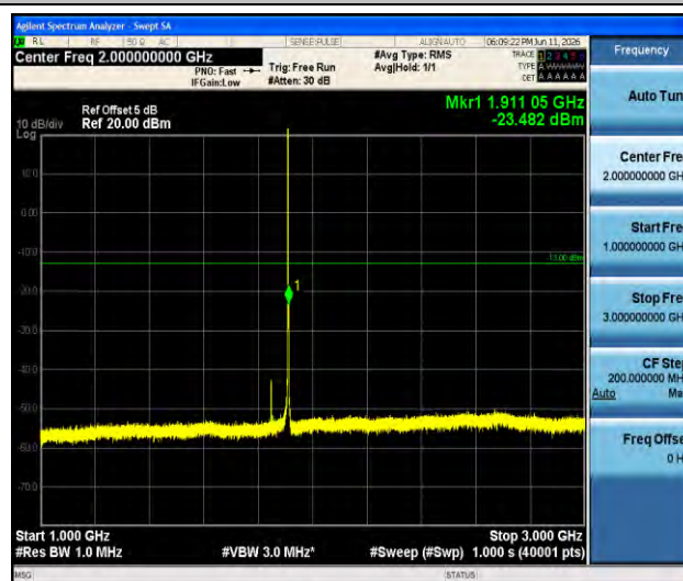
Band2-1.4MHz-QPSK-19193-1RB#0-1000~3000-PASS
