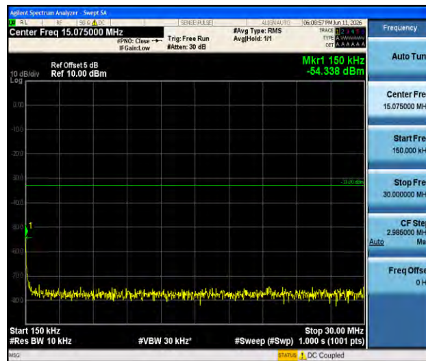
Band2-1.4MHz-QPSK-19193-1RB#0-0.15~30-PASS
