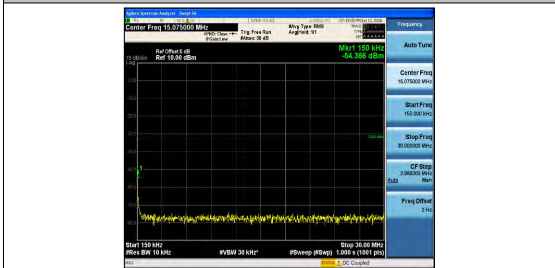
Band2-5MHz-QPSK-19175-1RB#0-0.15~30-PASS
