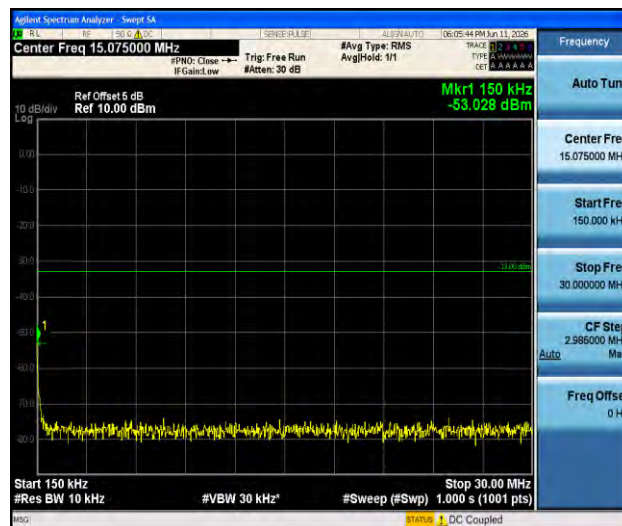
Band2-1.4MHz-16QAM-18607-1RB#0-0.15~30-PASS
