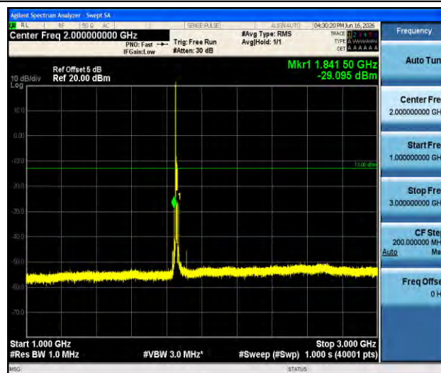
Band2-10MHz-QPSK-18650-1RB#0-1000~3000-PASS
