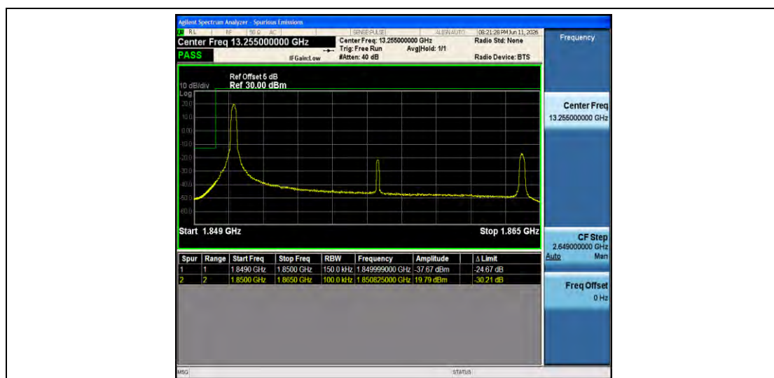
Band2-15MHz-QPSK-18675-1RB#0-PASS
