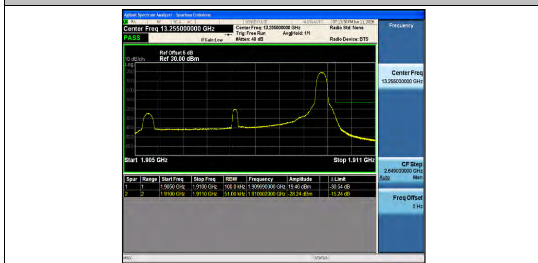
Band2-5MHz-QPSK-19175-1RB#24-PASS
