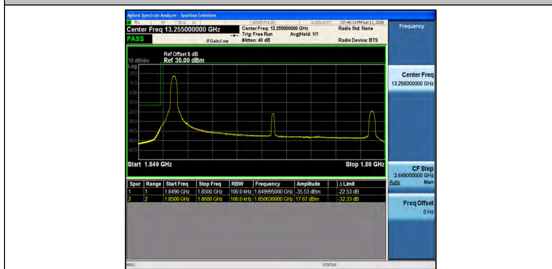
Band2-10MHz-16QAM-18650-1RB#0-PASS
