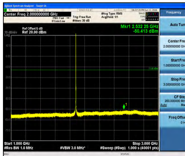
Band2-1.4MHz-QPSK-18900-1RB#0-1000~3000-PASS
