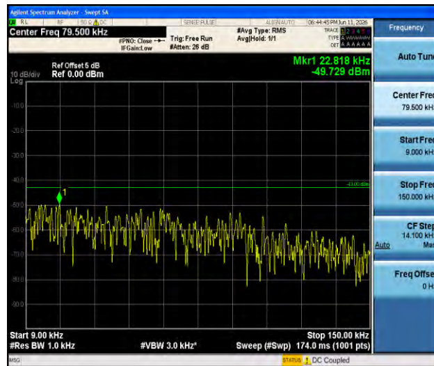
Band2-3MHz-16QAM-19185-1RB#0-0.009~0.15-PASS
