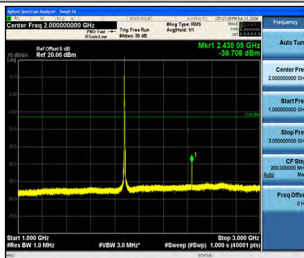
Band2-5MHz-QPSK-18900-1RB#0-1000~3000-PASS
