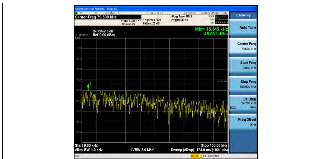
Band2-3MHz-16QAM-18900-1RB#0-0.009~0.15-PASS
