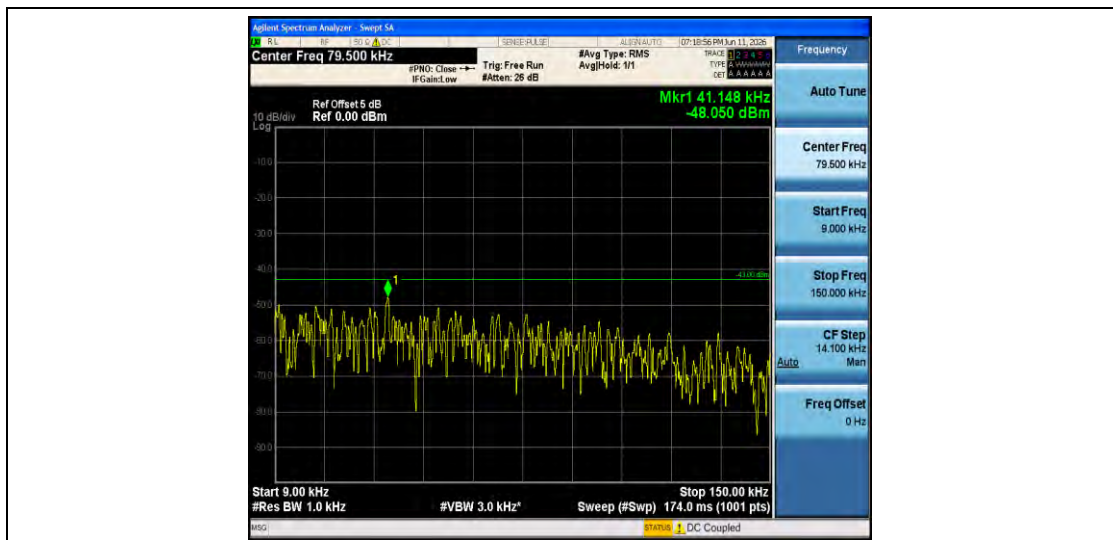
Band2-5MHz-QPSK-19175-1RB#0-0.009~0.15-PASS
