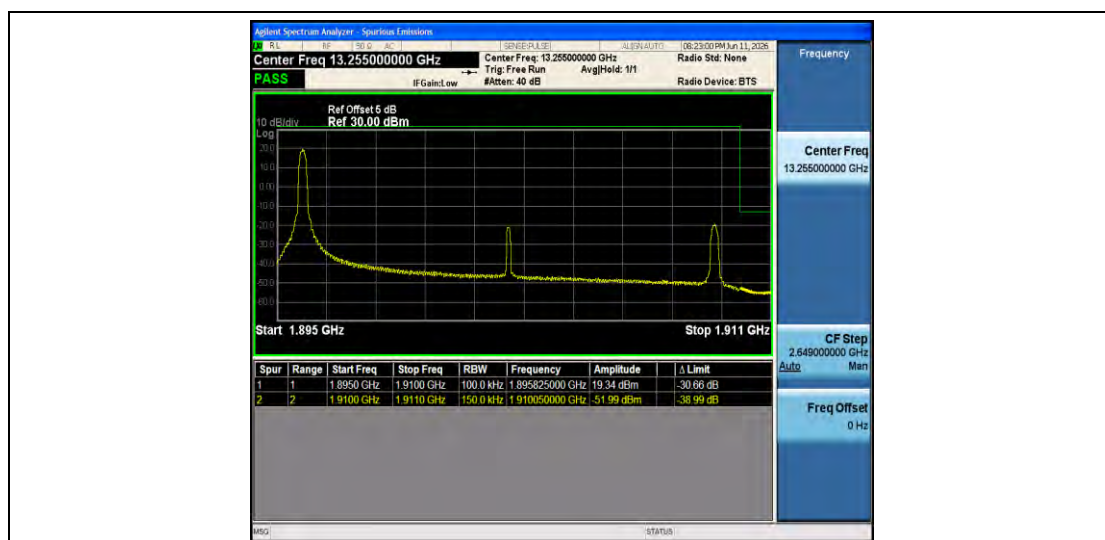
Band2-15MHz-QPSK-19125-1RB#0-PASS
