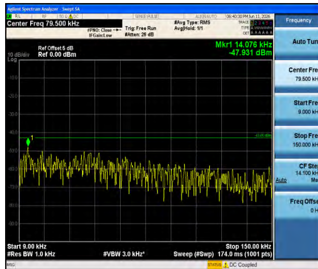
Band2-3MHz-16QAM-18615-1RB#0-0.009~0.15-PASS
