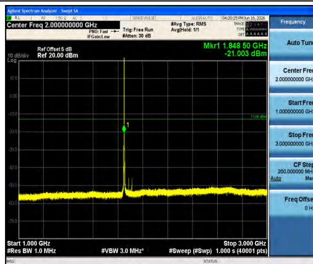
Band2-1.4MHz-16QAM-18607-1RB#0-1000~3000-PASS
