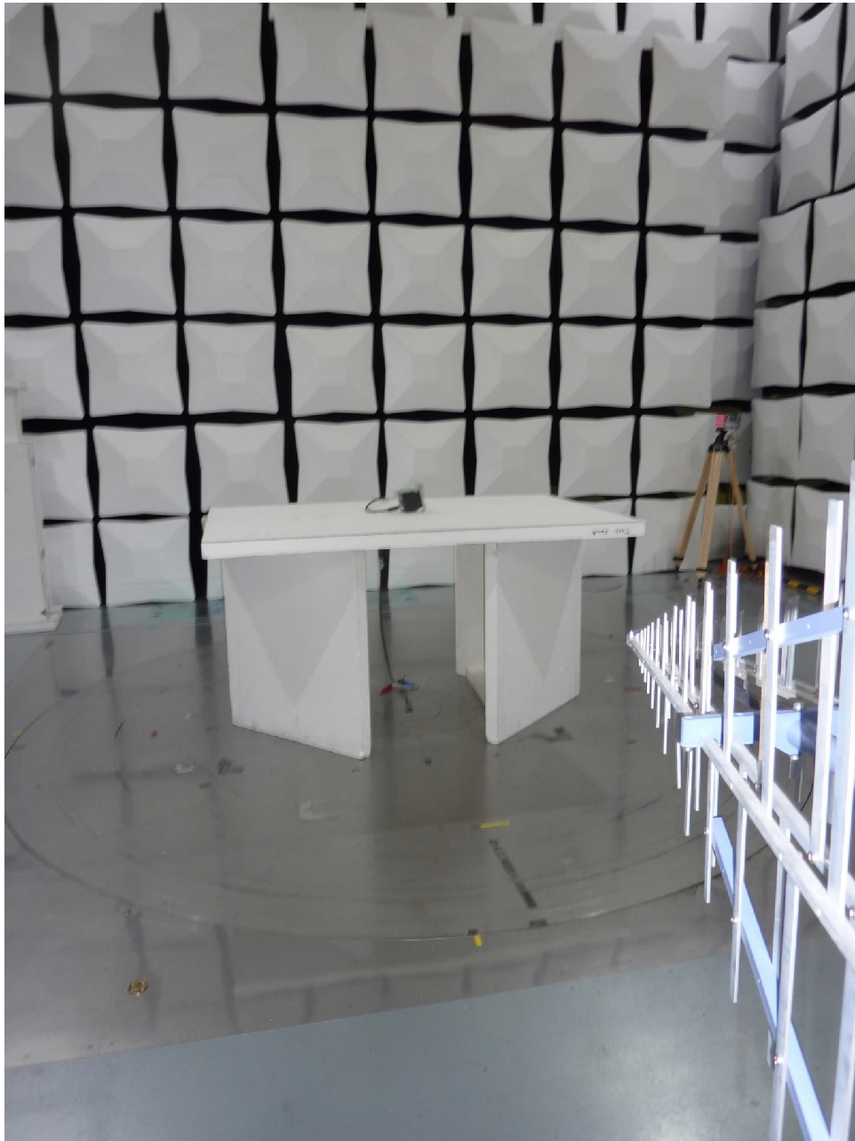
Test setup semi anechoic chamber <1 GHz
