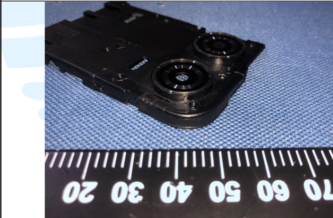
EUT Photo(WLAN/BT/GPS Antenna)
