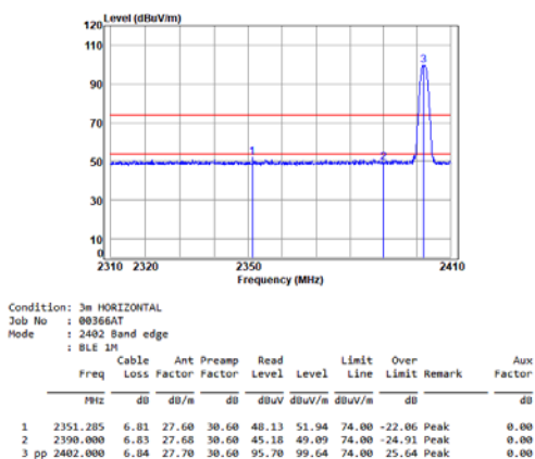
BLE_1M_TX_CH_00_Horizontal
