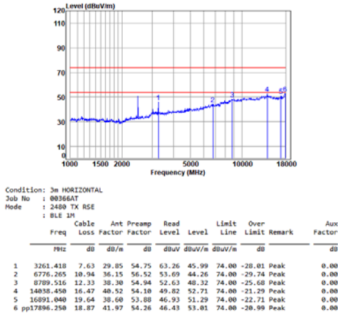
BLE_1M_TX_CH_39_Horizontal
