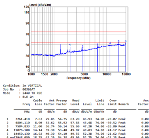
BLE_2M_TX_CH_19_Vertical
