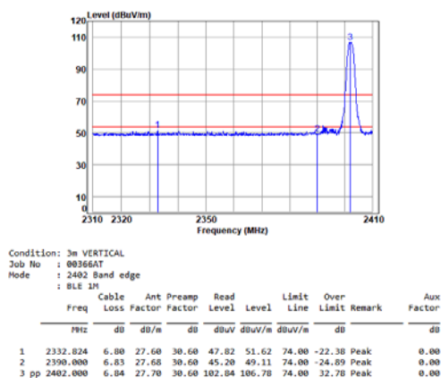
BLE_1M_TX_CH_00_Vertical
