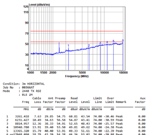
BLE_2M_TX_CH_19_Horizontal
