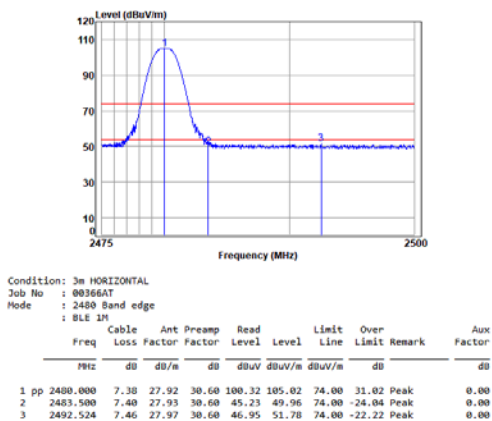
BLE_1M_TX_CH_39_Horizontal
