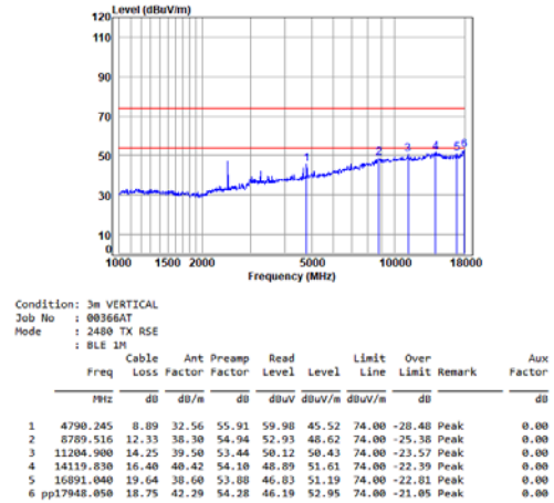
BLE_1M_TX_CH_39_Vertical
