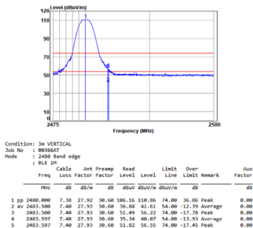
BLE_1M_TX_CH_39_Vertical
