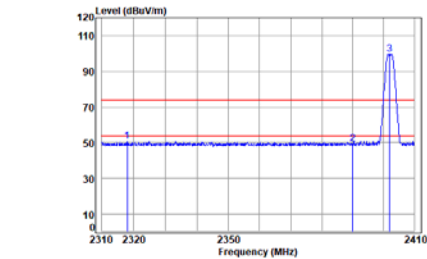
BLE_2M_TX_CH_00_Horizontal
